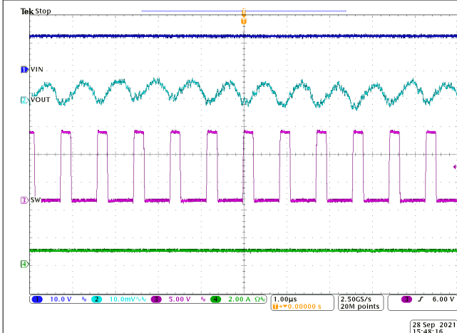
8-8. Steady State Waveforms, I_{OUT} = 1.0 A
