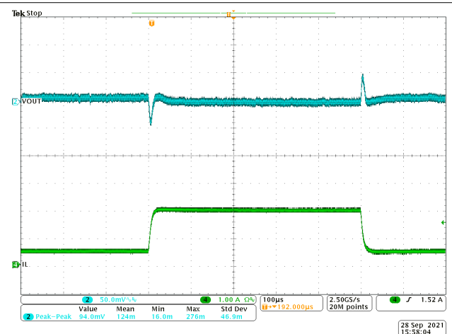
8-11. Transient Response 0.5 to 2 A with Slew Rate of 2.5 A/µs
