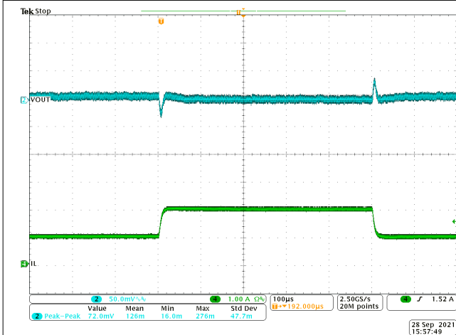
8-12. Transient Response 1 to 2 A with Slew Rate of 2.5 A/µs
