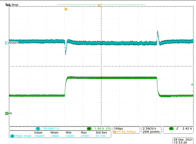
8-13. Transient Response 1.5 to 3 A with Slew Rate of 2.5 A/µs
