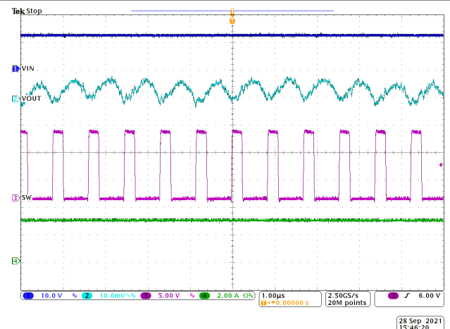
8-9. Steady State Waveforms, I_{OUT} = 3 A
