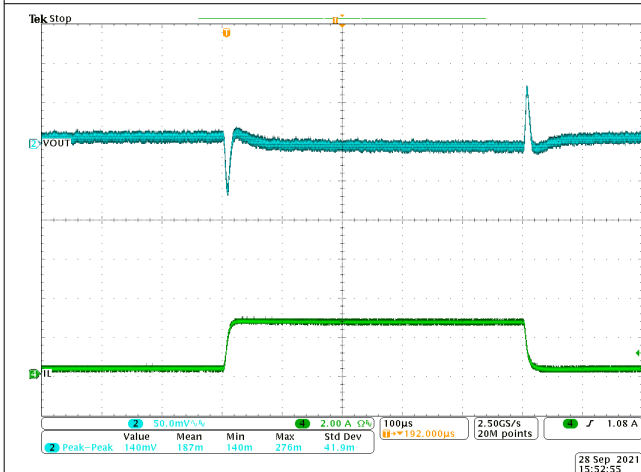
8-10. Transient Response 0.3 to 2.7 A with Slew Rate of 2.5 A/µs
