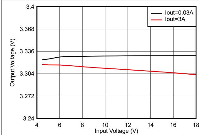
8-4. Line Regulation
