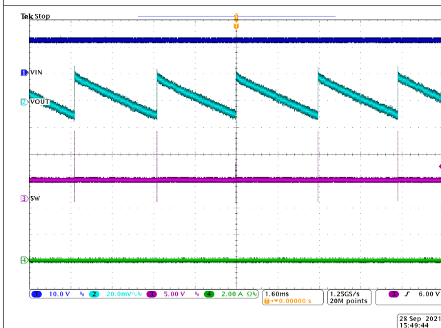
8-6. Steady State Waveforms, I_{OUT} = 0\text{ A}
