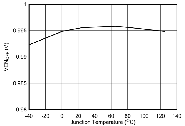
Figure 5-4. Enable Off Threshold Voltage
