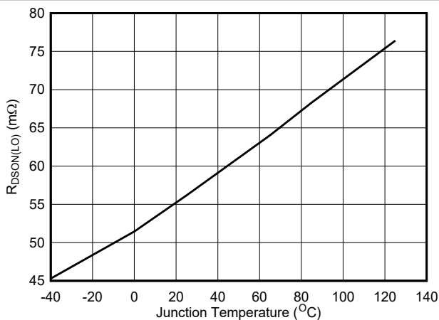
Figure 5-5. Low-Side R_{dson}
