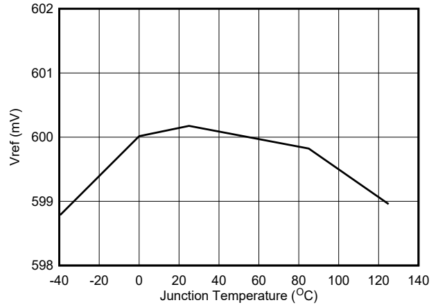
Figure 5-2. Vref Voltage
