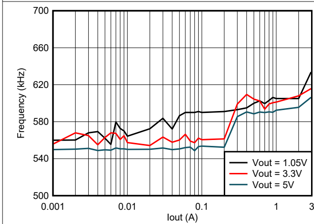
5-9. TPS563206 Frequency vs Loading
