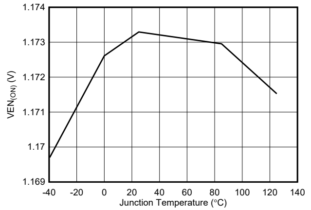
6-2. Enable On Threshold Voltage
