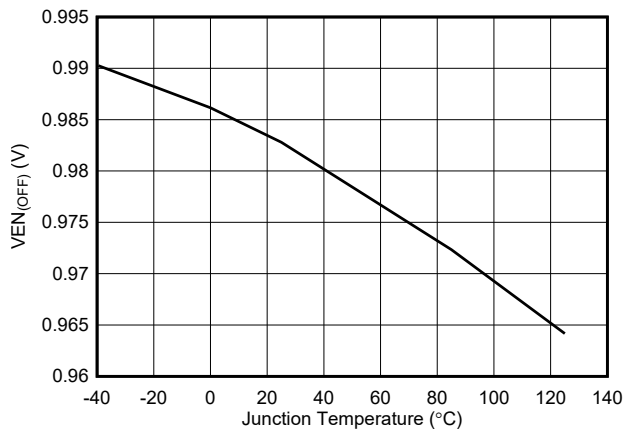
6-3. Enable Off Threshold Voltage
