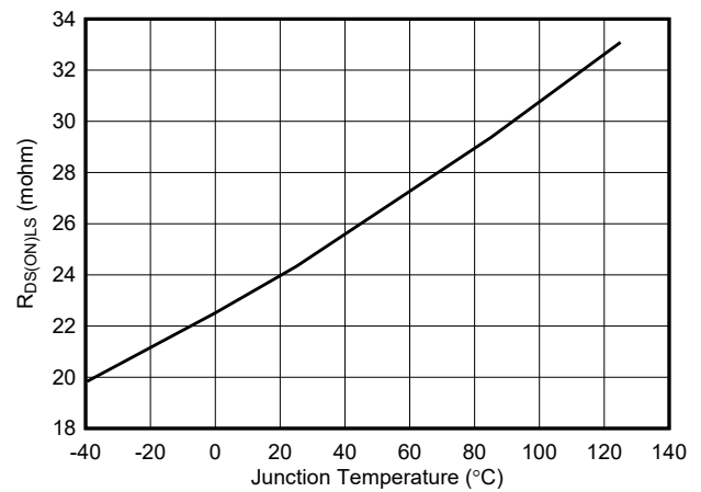
6-4. Low-Side R_{DS(ON)}
