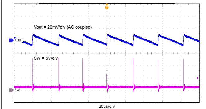
8-6. Output Voltage Ripple with 0.01-A Loading
