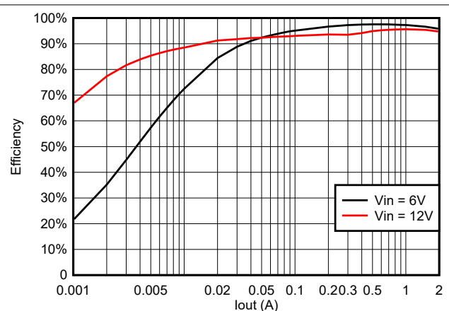
6-10. Efficiency at 5 V_{OUT} with a 3.3- \mu\text{H} Inductor
