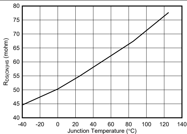
6-5. High-Side R_{DS(ON)}
