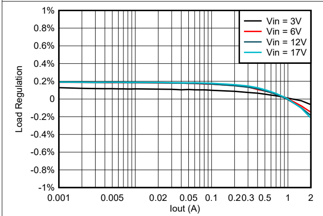
8-4. Load Regulation vs Loading
