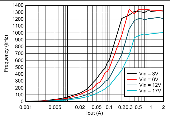
8-3. Frequency vs Loading
