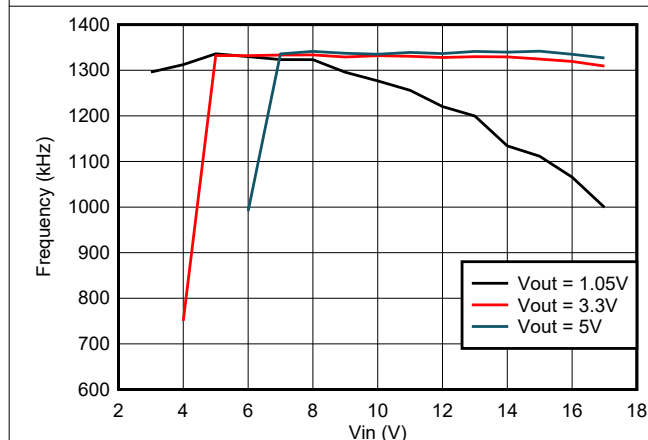
6-11. Frequency vs Input Voltage, I_{OUT} = 2\text{ A}
