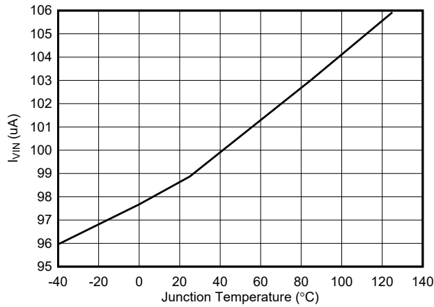
6-1. Quiescent Current
