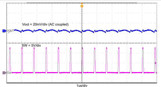
8-7. Output Voltage Ripple with 2-A Loading
