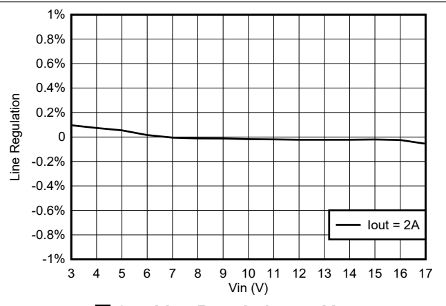
8-5. Line Regulation vs V_{IN}
