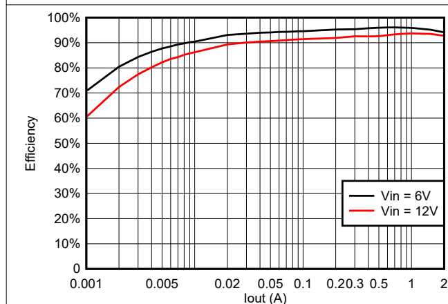
6-9. Efficiency at 3.3 V_{OUT} with a 2.2- \mu\text{H} Inductor
