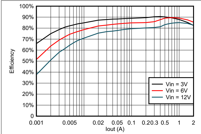
8-2. Efficiency vs Loading
