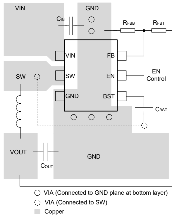
8-16. Suggested Layout
