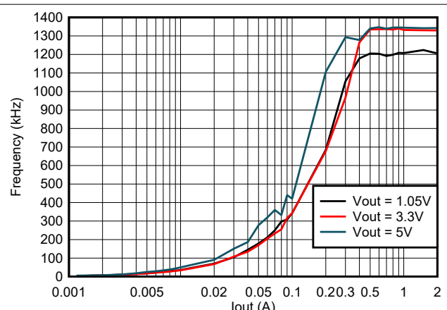
6-12. Frequency vs Loading, V_{IN} = 12\text{ V}
