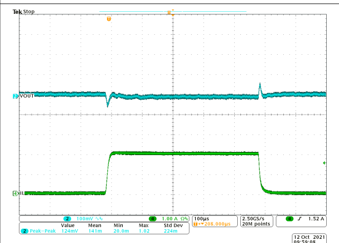
8-13. Transient Response 0 to 2 A with Slew Rate of 2.5 A/ \mu\text{s} (FCCM)
