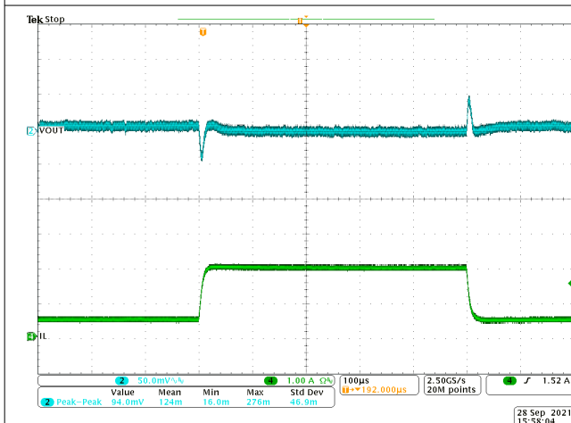
8-10. Transient Response 0.5 to 2 A with Slew Rate of 2.5 A/ \mu\text{s}
