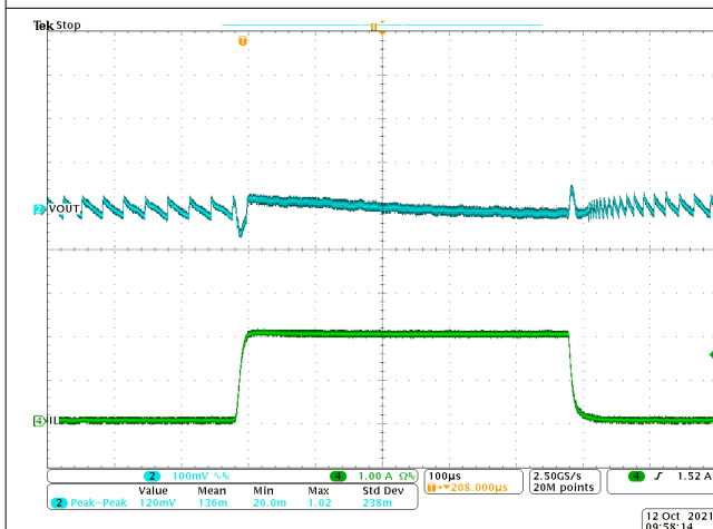
8-12. Transient Response 0 to 2 A with Slew Rate of 2.5 A/ \mu\text{s} (ECO)
