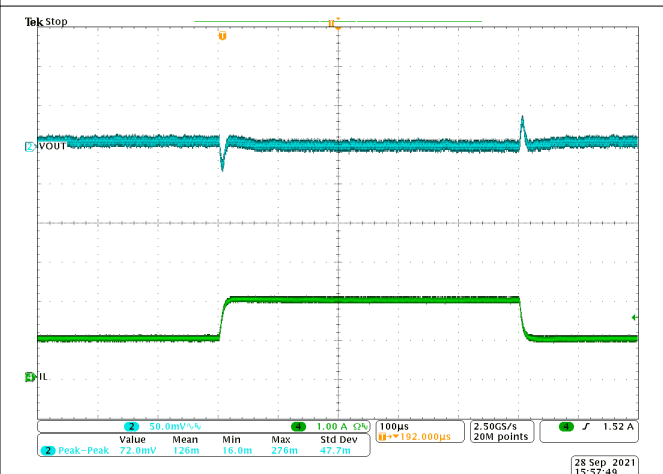
8-11. Transient Response 1 to 2 A with Slew Rate of 2.5 A/ \mu\text{s}
