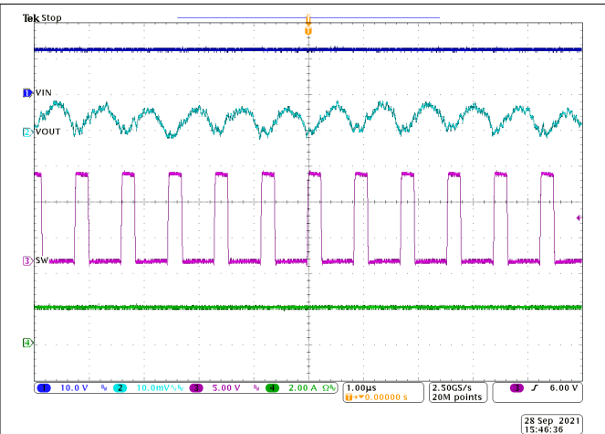
8-9. Steady State Waveforms, I_{OUT} = 2\text{ A}
