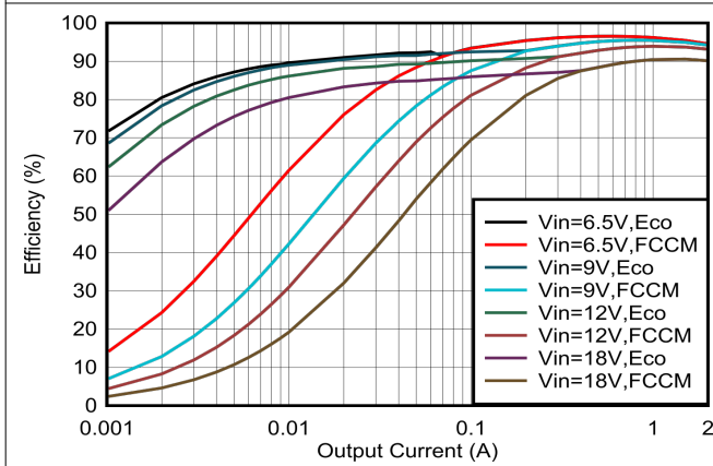
6-15. V_{OUT} = 5\text{-V} Efficiency, L = 3.3\ \mu\text{H}
