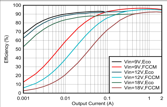
6-16. V_{OUT} = 7\text{-V} Efficiency, L = 3.3\ \mu\text{H}
