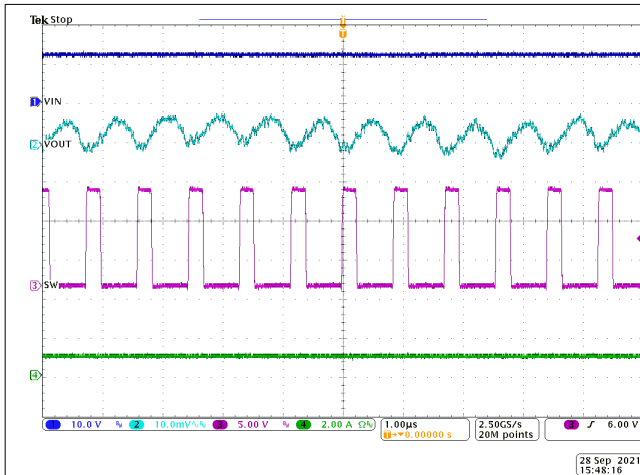
8-8. Steady State Waveforms, I_{OUT} = 1.0\text{ A}
