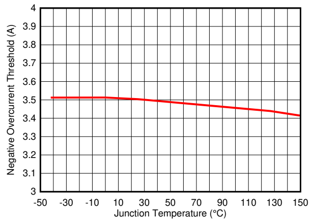
図 5-4. Negative Overcurrent Limit
