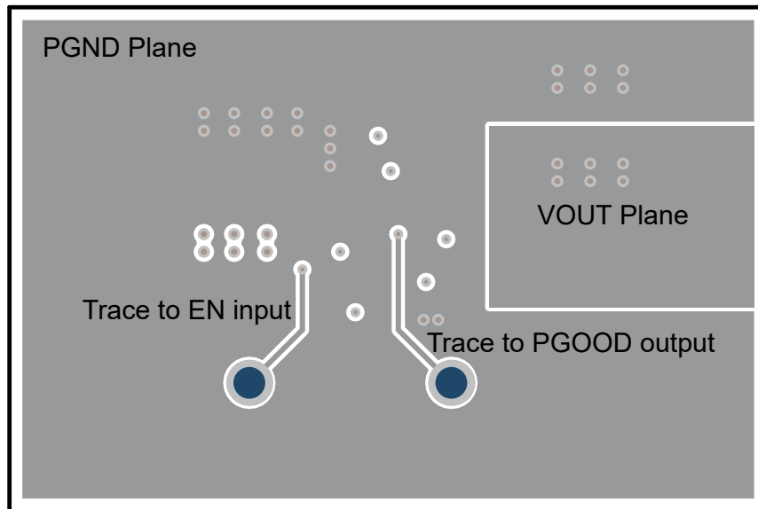
図 7-34. Bottom Layer Layout (Viewed from Top)
