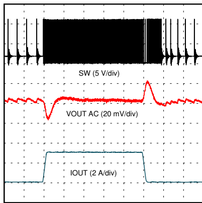
Time (20 μs/div) V_{IN} = 12 V 0.1 A to 3.1 A step 1 A/μsec MODE = DCM
