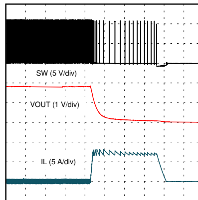
7-30. Short Circuit Response
