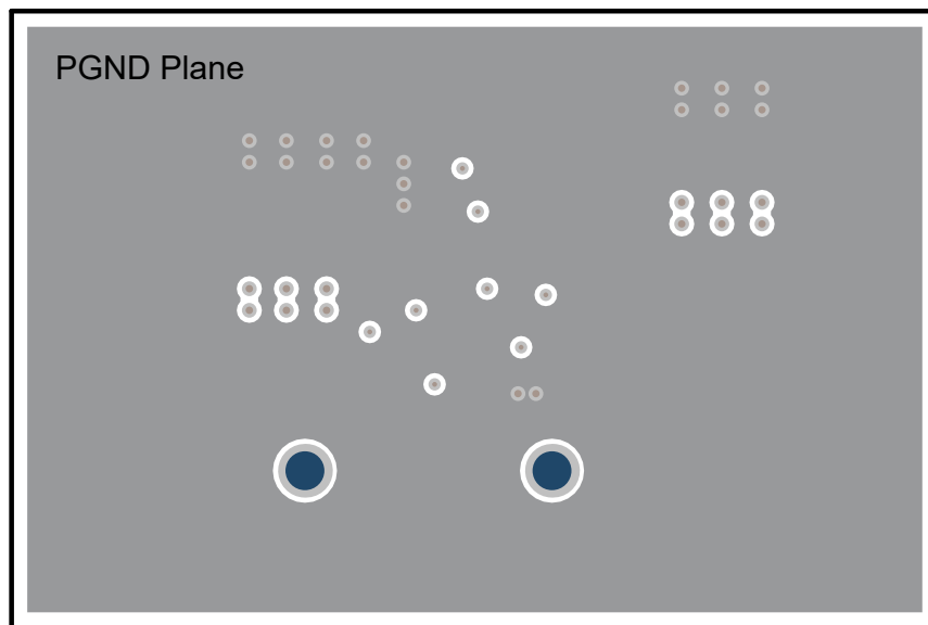
7-32. Signal Layer 1 Layout
