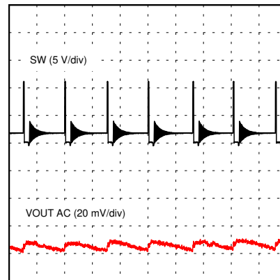
Time (4 μs/div) V_{IN} = 12 V I_{LOAD} = 0.1 A MODE = DCM
