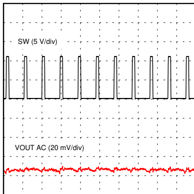
Time (1 μs/div) V_{IN} = 12 V I_{LOAD} = 0.1 A MODE = FCCM
