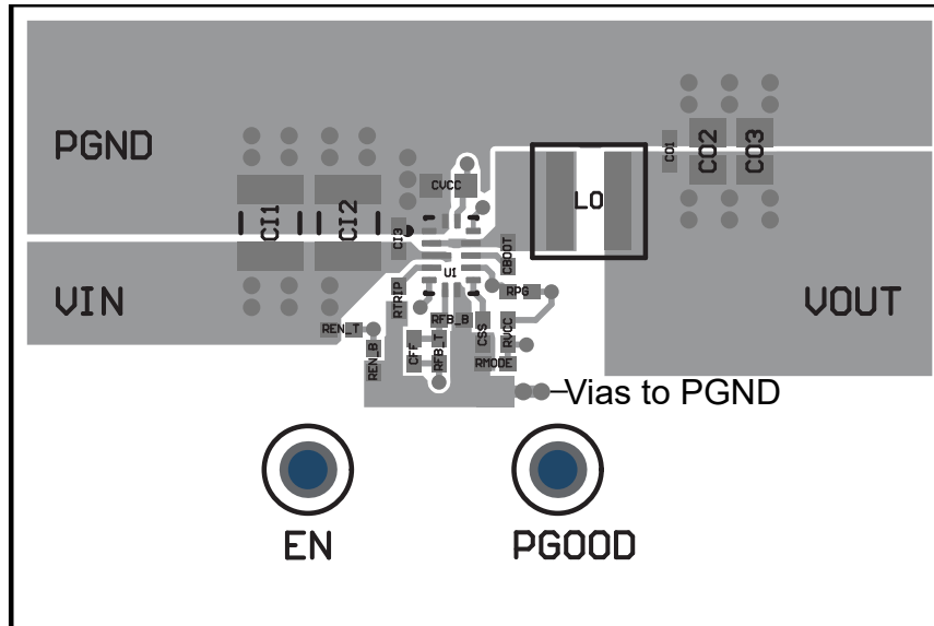
7-31. Top Layer Layout
