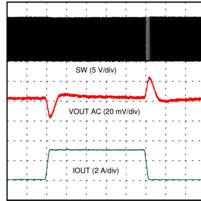
Time (20 μs/div) V_{IN} = 12 V 0.1 A to 3.1 A step 1 A/μsec MODE = FCCM
