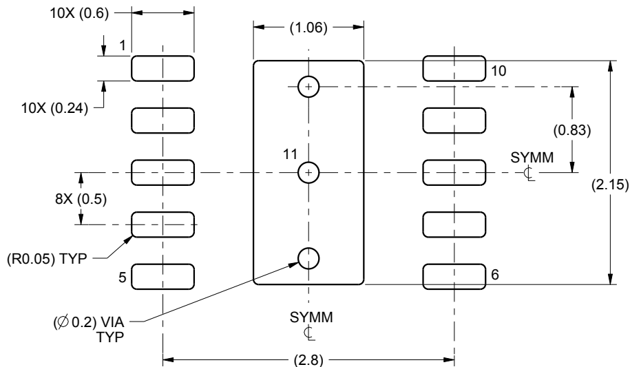
LAND PATTERN EXAMPLE SCALE:20X
