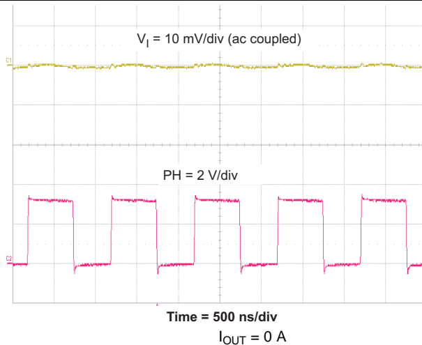
Figure 49. Input Ripple
