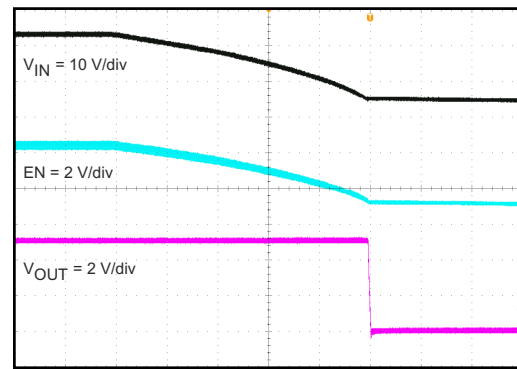
Time - 2 ms/div 8-13. Shutdown Relative to VIN
