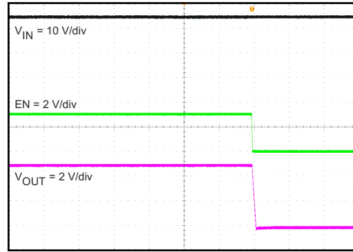
8-15. Shutdown Relative to EN
