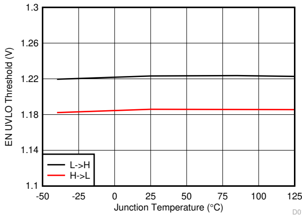
6-11. EN Threshold vs Junction Temperature
