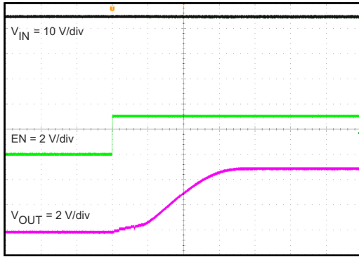
8-14. Start-Up Relative to EN
