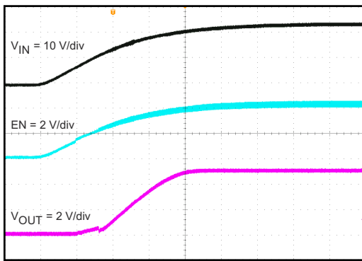
Time - 2 ms/div 8-12. Start-Up Relative to VIN
