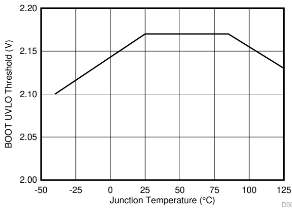
6-9. BOOT-SW UVLO Threshold vs Junction Temperature
