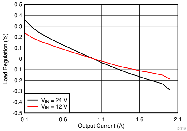
8-4. Load Regulation
