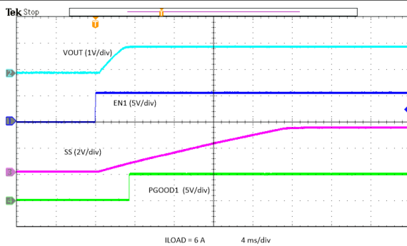
8-39. Power Up with EN
