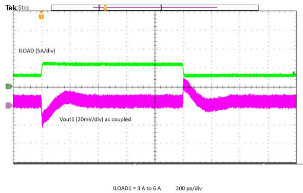
8-13. V_{OUT1} Load Transient
