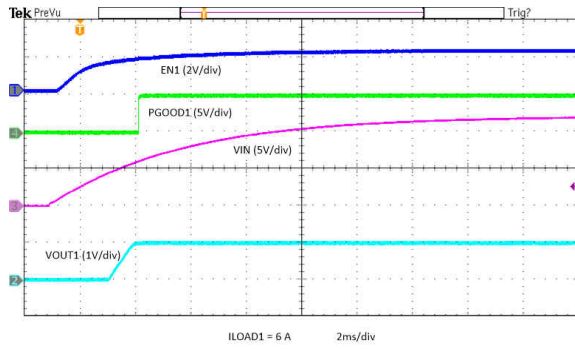
8-23. Power Up with V_{IN} V_{OUT1}
