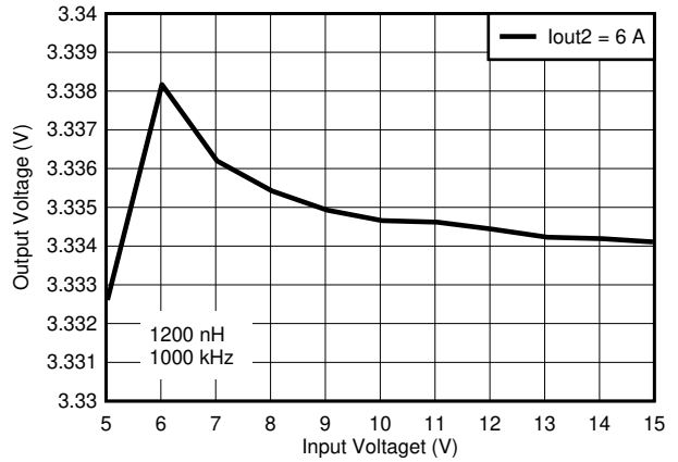
8-10. Line Regulation V_{OUT2}
