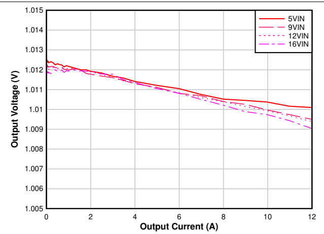
6-6. Output Voltage Regulation vs Output Current, V_{OUT} = 1.0\text{ V} , F_{SW} = 1\text{ MHz}
