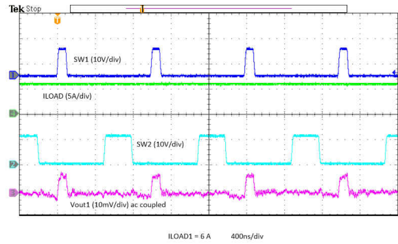
8-28. V_{OUT1} Output Ripple – 6-A Load
