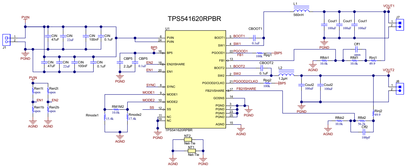
図 8-1. 12-V Input, 1.0-V and 3.3-V Dual Output Regulator Application Schematic
