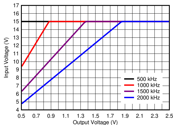
图 8-2. Maximum Input Voltage Versus Output Voltage
