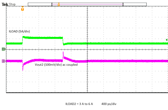
8-14. V_{OUT2} Load Transient
