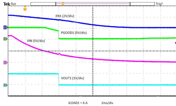
8-24. Power Down with V_{IN} V_{OUT1}
