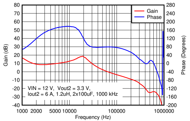
8-12. V_{OUT2} Bode Plot
