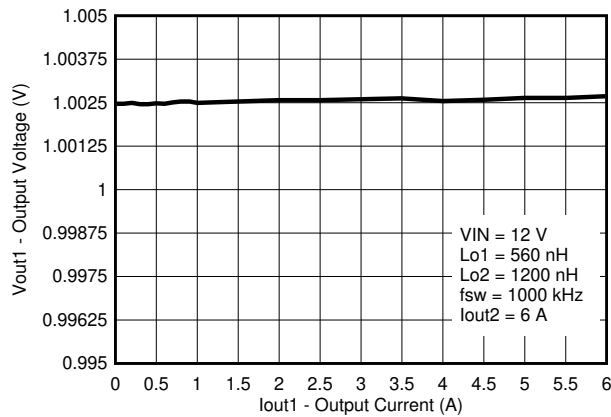
8-5. V_{OUT1} Load Regulation
