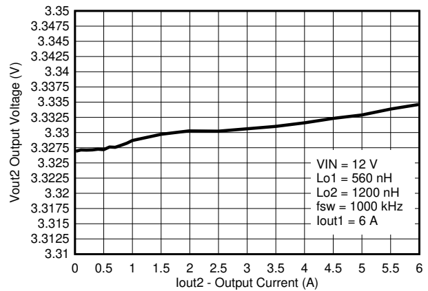
8-6. V_{OUT2} Load Regulation
