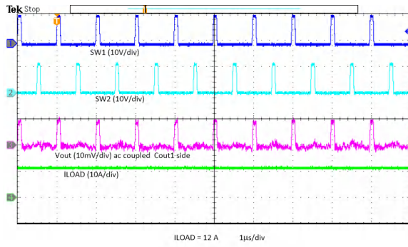
8-46. Output Ripple – 12-A Load
