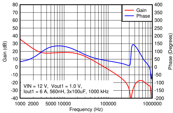
8-11. V_{OUT1} Bode Plot
