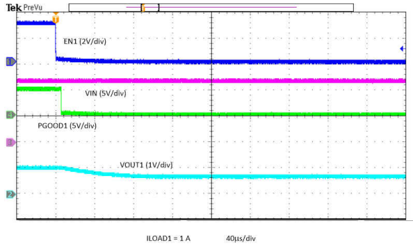
8-21. Power Down with EN 1 with Pre Bias
