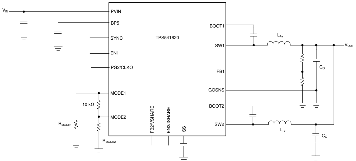
7-3. Dual-phase Configuration with External Clock
