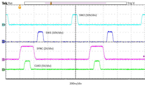
8-27. Sync In to SW1 and SW2 Delay
