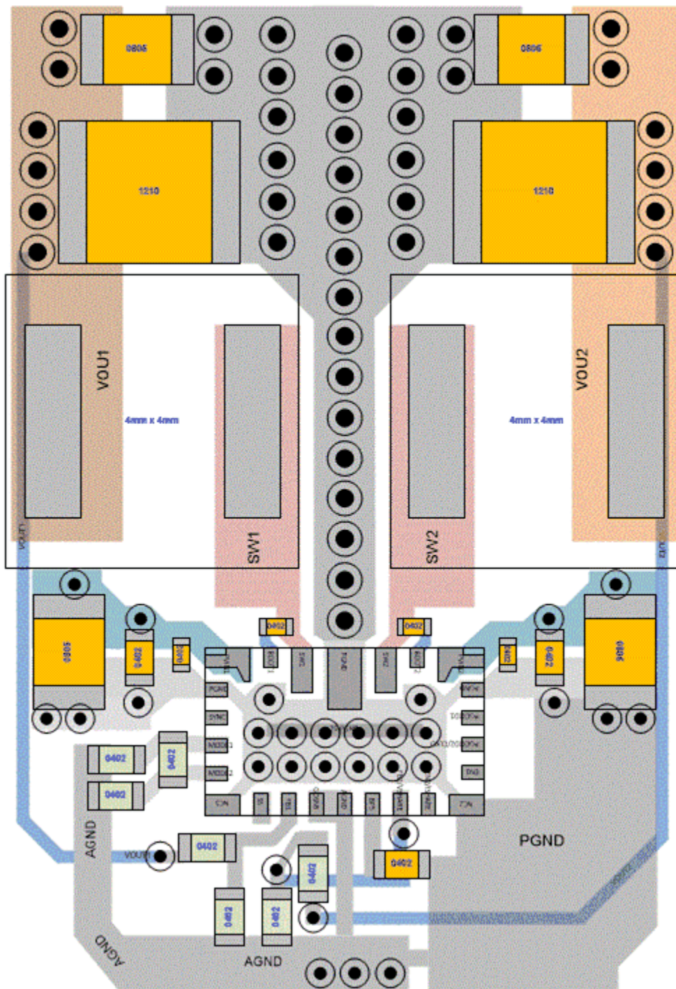
10-1. Example PCB Layout for Dual-output Configuration
