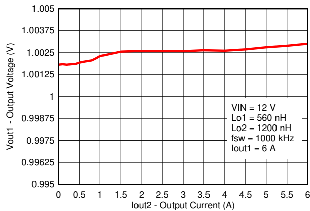
8-7. V_{OUT1} Cross Regulation
