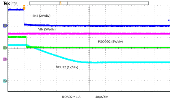
8-22. Power Down with EN 2 with Pre Bias
