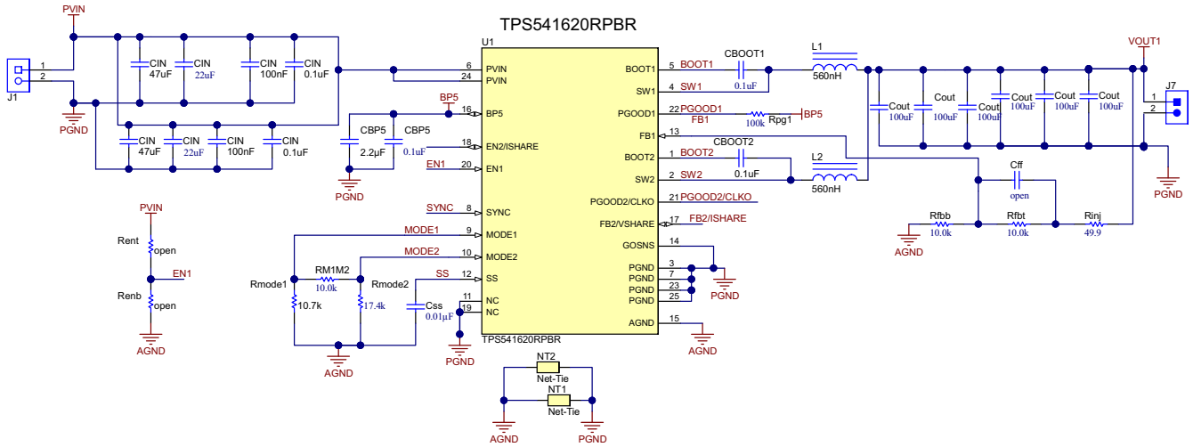
图 8-32. 12-V Input, 1.0-V Output 2-Phase Converter Application Schematic
