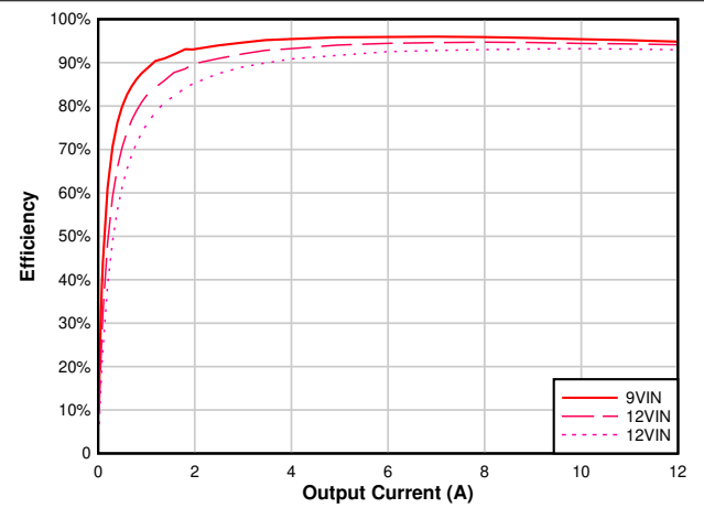
6-4. Efficiency vs Output Current, V_{OUT} = 5.5\text{ V} , F_{SW} = 1\text{ MHz}
