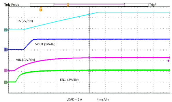
8-41. Power Up with V_{IN}
