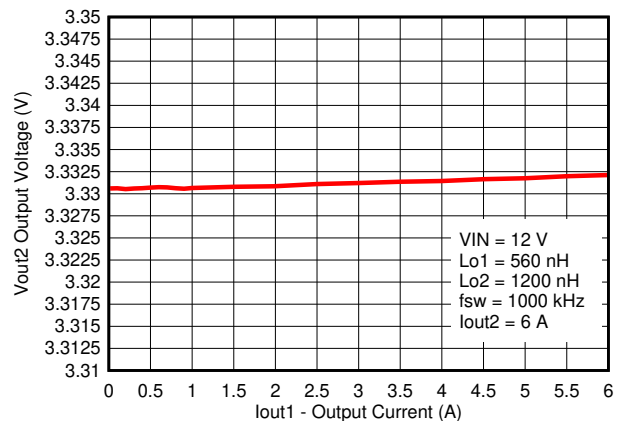
8-8. V_{OUT2} Cross Regulation
