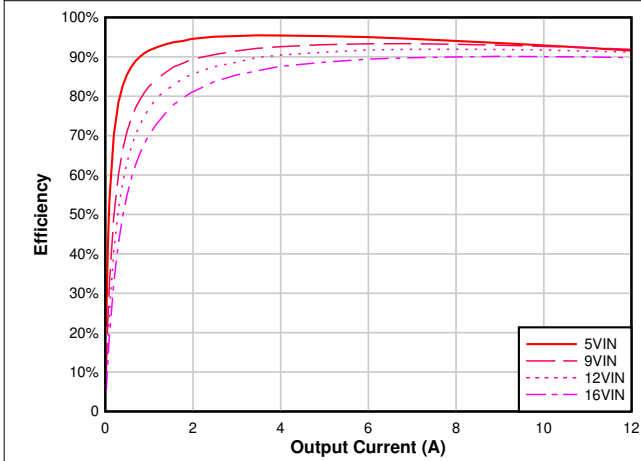
6-3. Efficiency vs Output Current, V_{OUT} = 3.3\text{ V} , F_{SW} = 1\text{ MHz}
