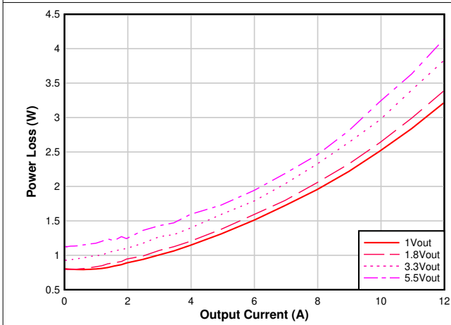
6-5. Power Dissipation vs Output Current, V_{IN} = 12\text{ V} , F_{SW} = 1\text{ MHz}
