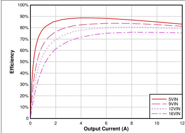
6-1. Efficiency vs Output Current, V_{OUT} = 1.0\text{ V} , F_{SW} = 1\text{ MHz}
