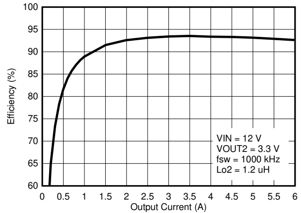
8-4. V_{OUT2} Efficiency
