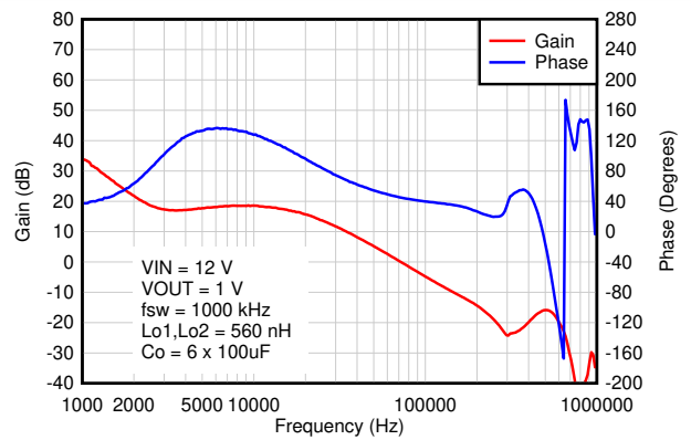
8-37. Bode Plot
