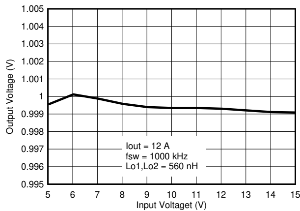
8-36. Line Regulation
