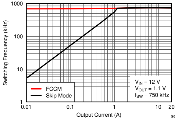
6-7. Switching Frequency vs. Output Current
