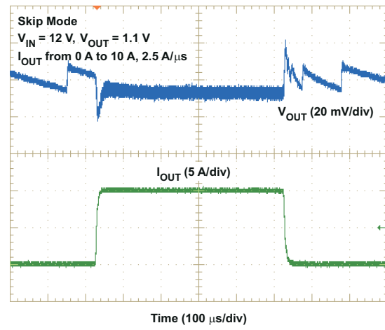
6-22. Skip Mode Load Transient
