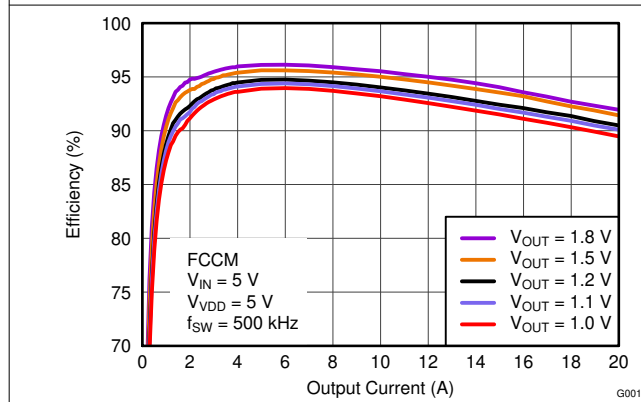
6-32. Efficiency vs Output Current
