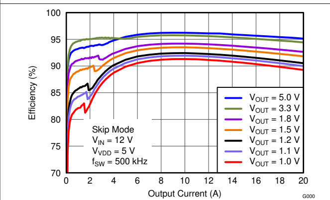
6-31. Efficiency vs Output Current
