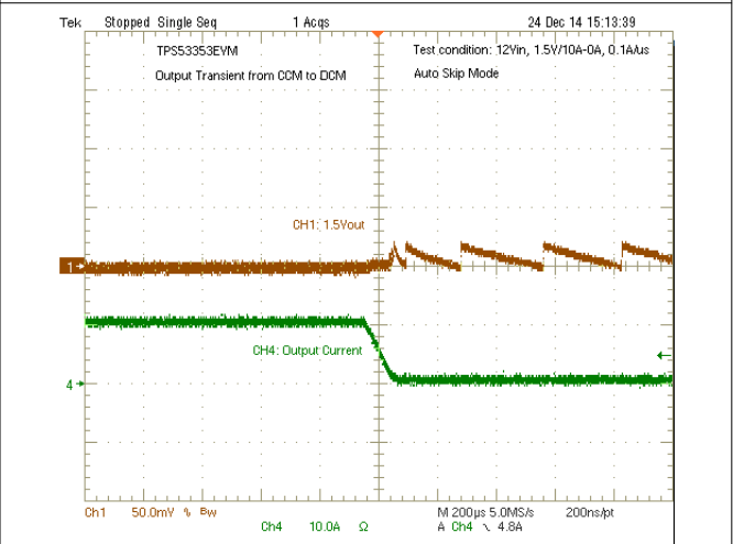
8-8. Output Transient from DCM to DCM
