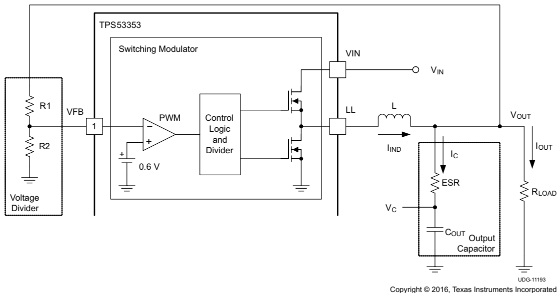
7-4. Simplified Modulator Model
