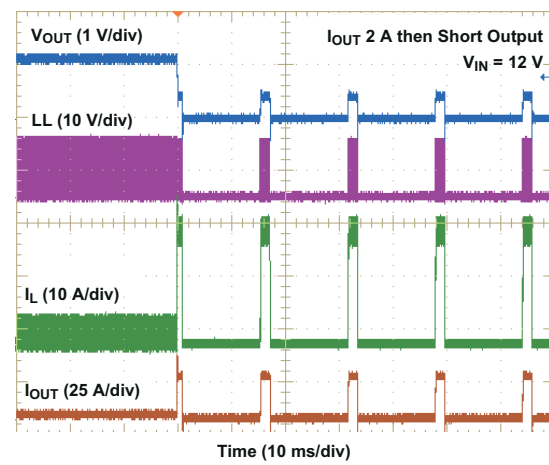
6-24. Output Short-Circuit Protection Waveforms
