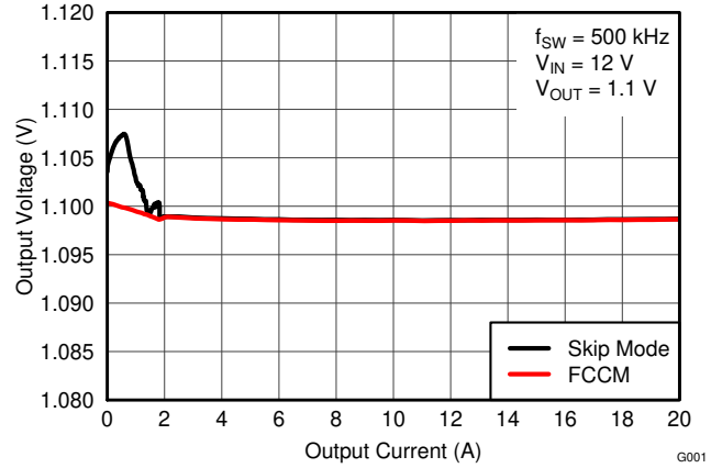
6-10. Output Voltage vs. Output Current
