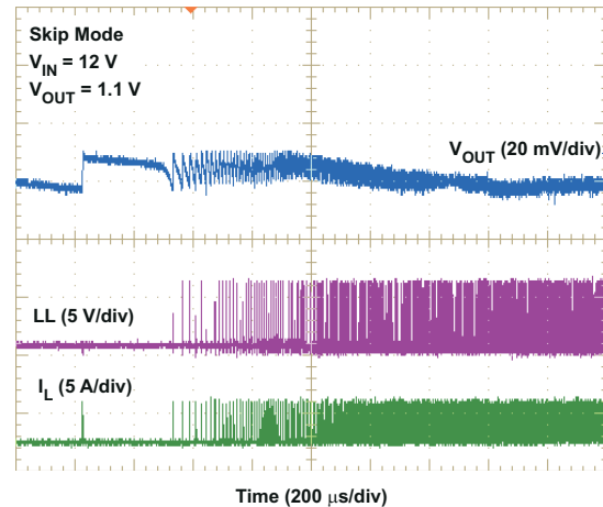
6-20. DCM-to-CCM Transition Waveforms
