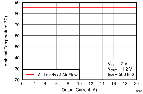
6-26. Safe Operating Area
