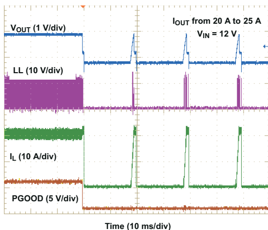
6-23. Overcurrent Protection Waveforms
