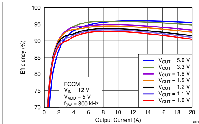
6-28. Efficiency vs Output Current
