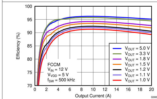
6-30. Efficiency vs Output Current
