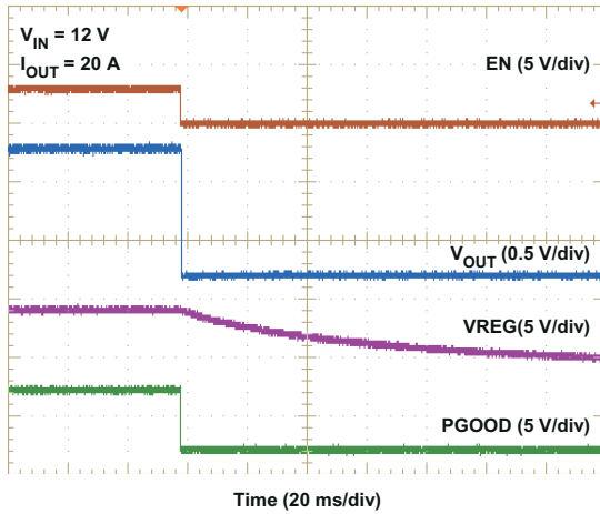
6-15. Shutdown Waveforms
