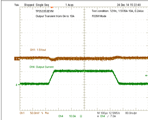
8-9. Output Transient with FCCM Mode
