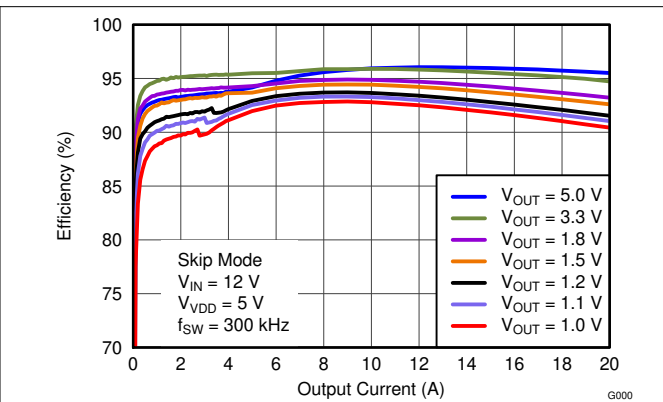
6-29. Efficiency vs Output Current
