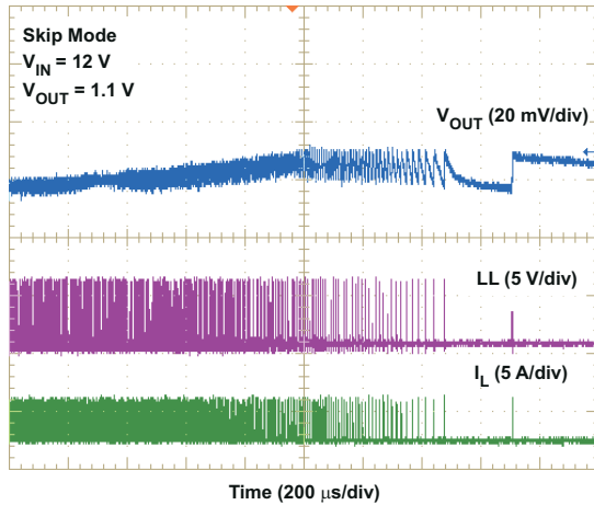
6-19. CCM-to-DCM Transition Waveforms
