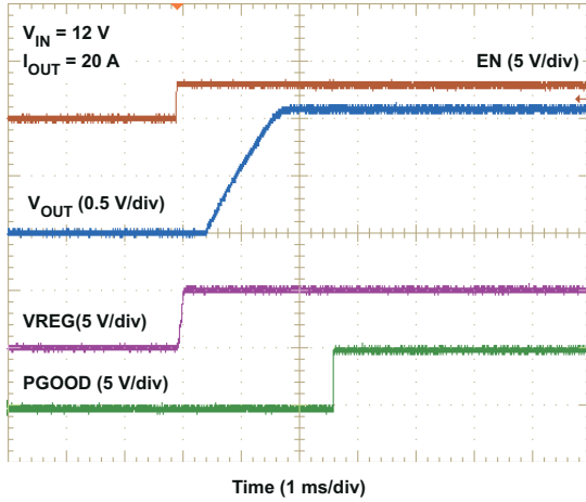
6-13. Start-Up Waveforms
