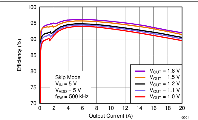
6-33. Efficiency vs Output Current
