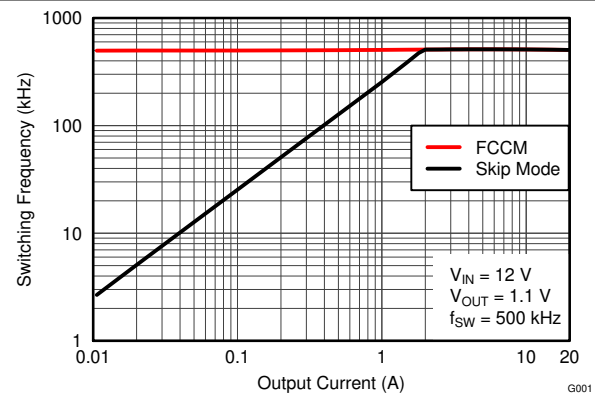
6-6. Switching Frequency vs. Output Current
