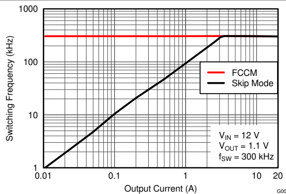
6-5. Switching Frequency vs. Output Current
