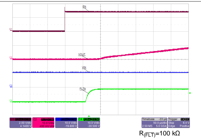
Figure 34. EN Turn ON Delay : EN ↑ to Output Ramp ↑
