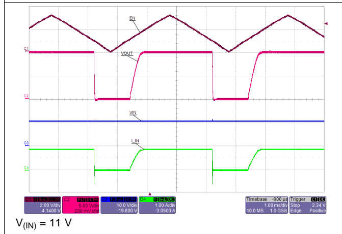
Figure 33. Turn ON and OFF with Enable
