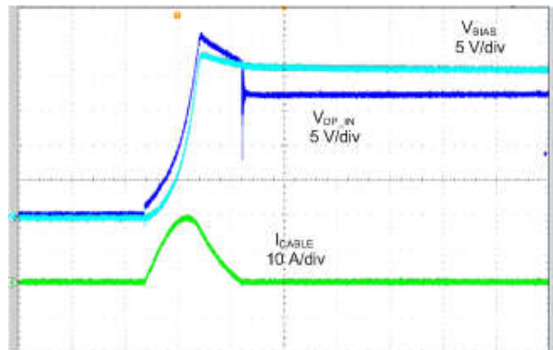
9-7. Enabled With OVP_SEL = High, OUT Shorted to Battery
