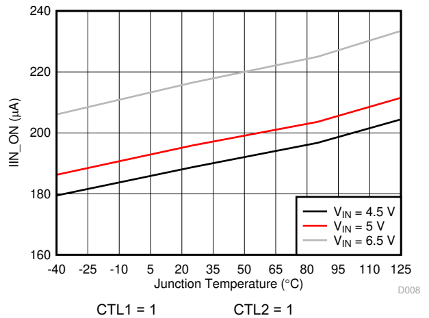
6-8. Enabled IN Supply Current – CDP (11) vs Temperature
