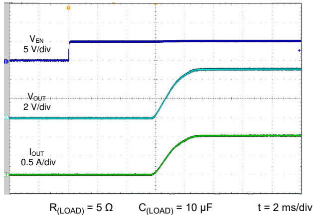
图 6-18. Turnon Response
