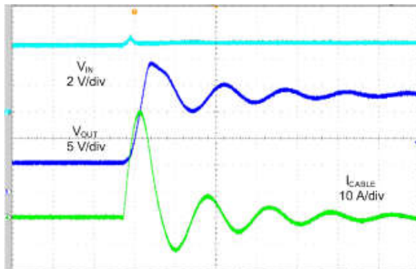
9-6. DC-DC Input Is Floating, OUT Shorted to Battery
