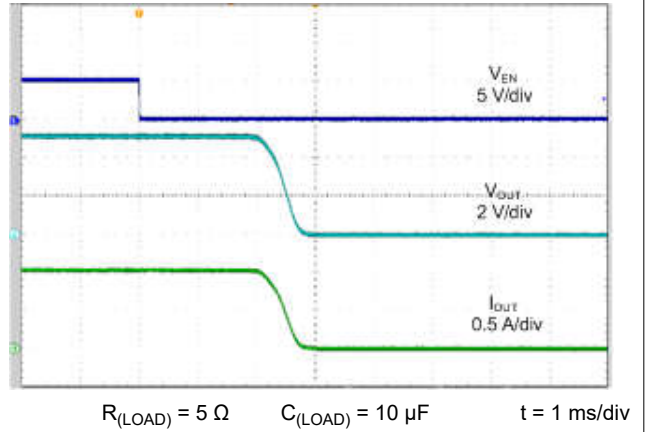
图 6-19. Turnoff Response
