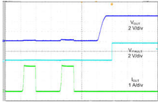
6-23. Short Circuit to No Load (CDP)
