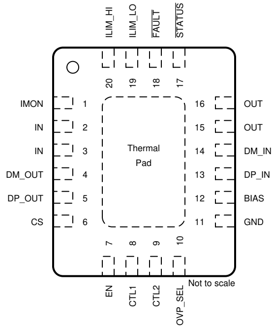
FIG 5-1. RVC Package 20-Pin WQFN Top View
