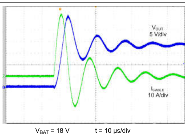
图 9-3. Disabled, 35-V, 1210, X7R C_{OUT} Capacitor Without SMAJ18
