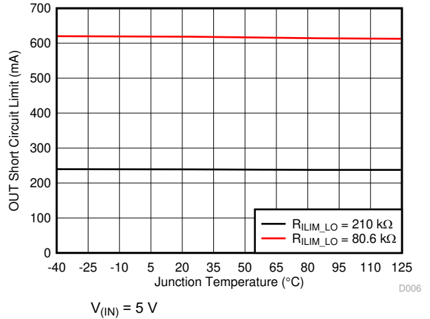
6-6. OUT Short-Circuit Current Limit vs Temperature II
