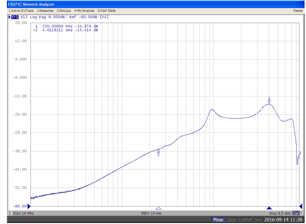
Figure 6-35. On-State Cross-Channel Isolation vs Frequency
