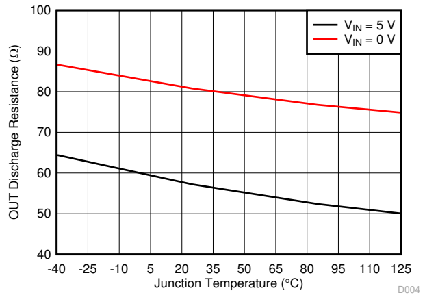
6-4. OUT Discharge Resistance (OVP) vs Temperature
