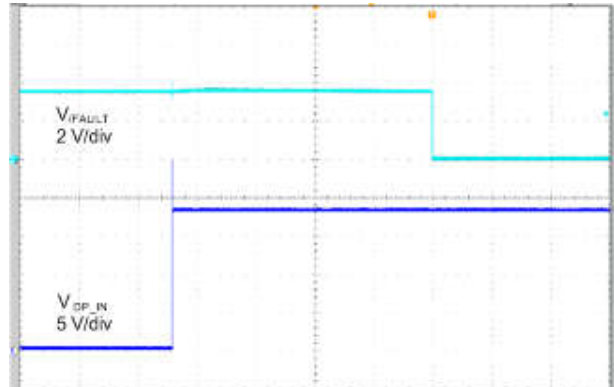
6-29. DP_IN Short to Battery
