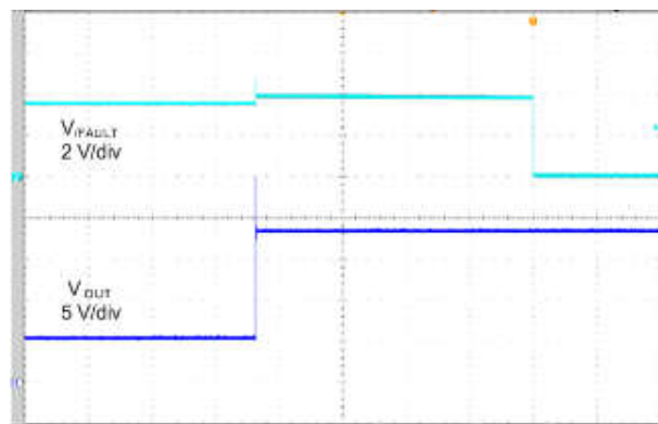
6-25. Load-Detection Set Time
