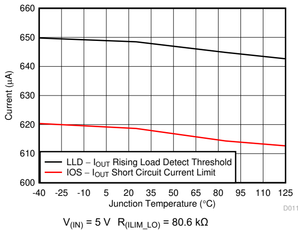
6-9. I (OUT) Rising Load-Detect Threshold and OUT Short-Circuit Limit vs Temperature
