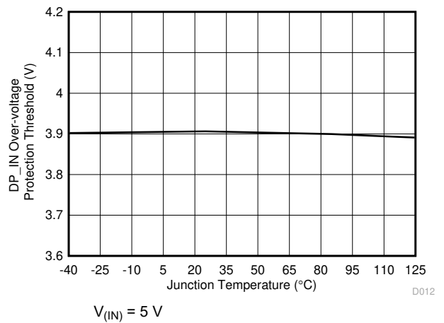
6-10. DP_IN Overvoltage Protection Threshold vs Temperature
