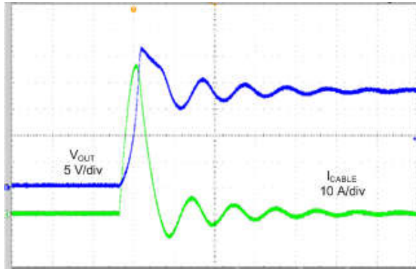
9-4. Disabled, 25-V, 1206, X7R C OUT Capacitor With SMAJ18, OUT Shorted to Battery
