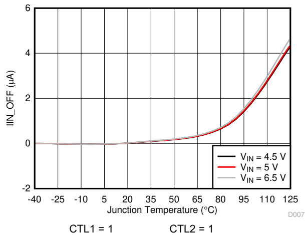
6-7. Disabled IN Supply Current vs Temperature
