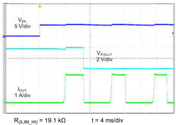
图 6-21. Enable Into Short (CDP) – Thermal Cycling
