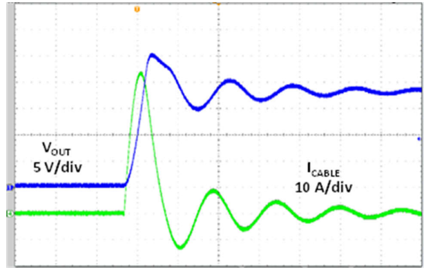
9-5. Disabled, 35-V, 1210, X7R C OUT Capacitor With SMAJ18, OUT Shorted to Battery
