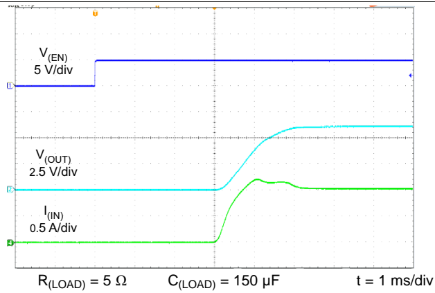
Figure 20. Turnon Response
