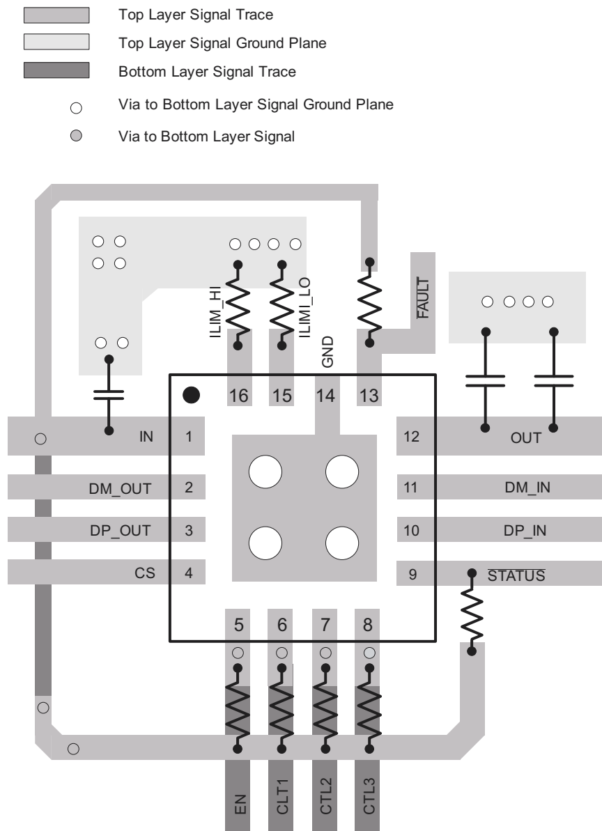
Figure 58. TPS2549 Layout Diagram
