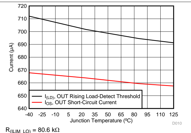
Figure 10. I_{OUT} Rising Load-Detect Threshold and I_{OUT} Short-Circuit Current Limit vs Temperature
