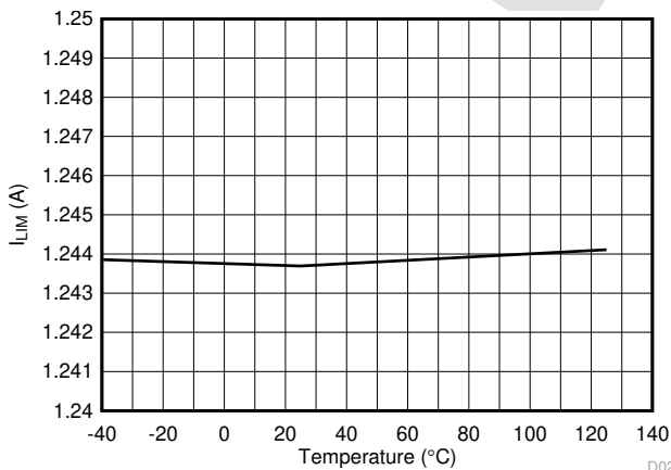
7-23. 2x Mode (2xFBn = 1) Current Limit vs Temperature
