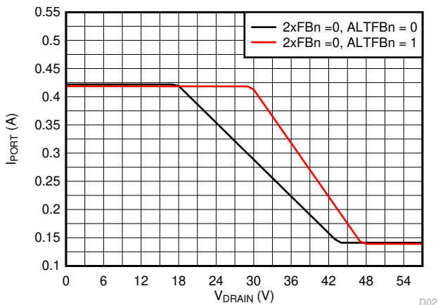
7-27. 1x Mode (2xFBn = 0) Current Foldback vs Drain Voltage
