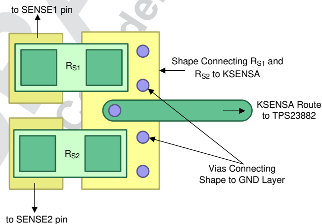
FIG 12-2. Kelvin Sense Layout Example
