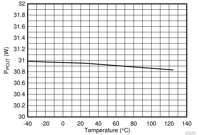
7-20. P CUT Threshold (30W) vs Temperature
