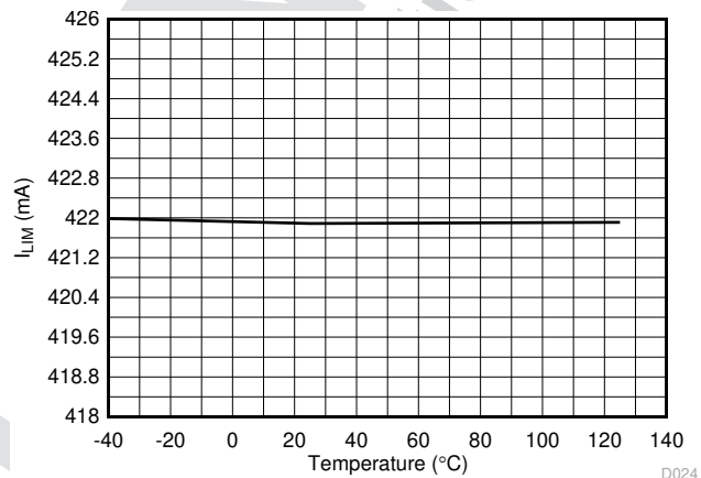
7-22. 1x Mode (2xFBn = 0) Current Limit vs Temperature
