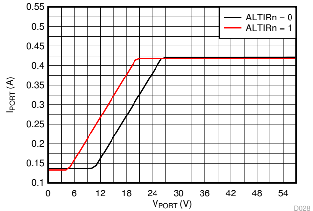
7-26. Inrush Current Foldback vs Port Voltage
