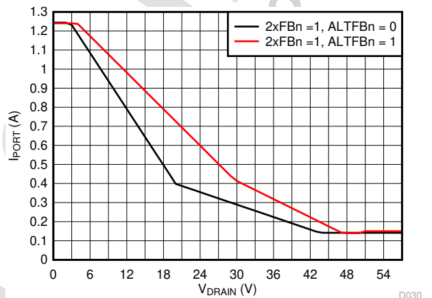
7-28. 2x Mode (2xFBn = 1) Current Foldback vs Drain Voltage
