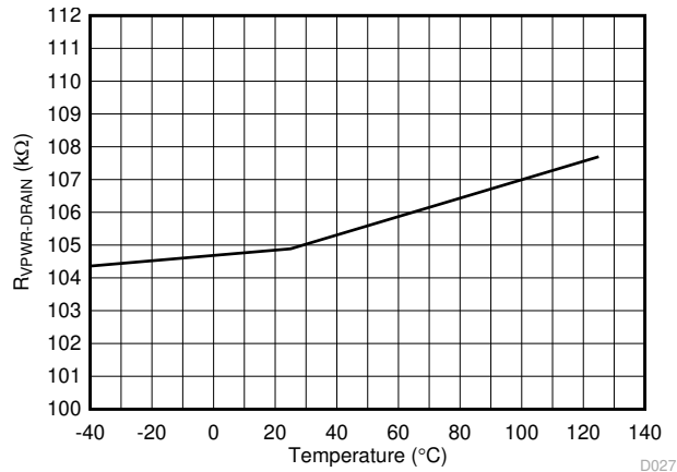
7-25. R OFF (VPWR to DRAIN) vs Temperature
