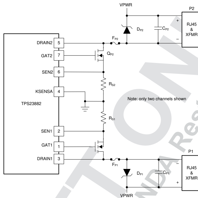
FIG 12-1. Kelvin Current-Sense Connection
