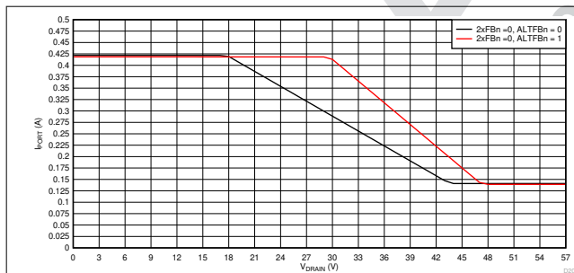
图 9-51. 1x Mode (2xFBn = 0) Foldback Curves, I_{PORT} vs V_{DRAIN}
