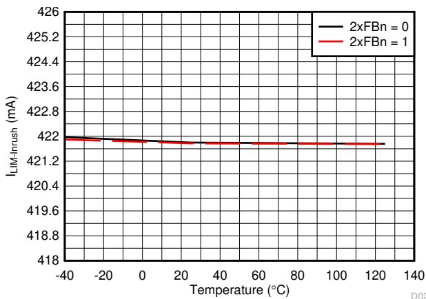
7-21. Inrush Current Limit vs Temperature
