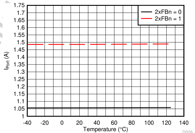
7-24. I SHORT Threshold vs Temperature
