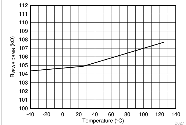
6-27. R_{\text{OFF}} (VPWR to DRAIN) vs Temperature
