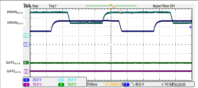
図 9-11. 4-Pair Open Circuit Detection Signature
