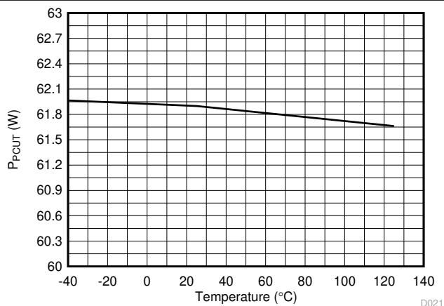
Figure 6-21. 4-Pair PCut Threshold (60W) vs Temperature
