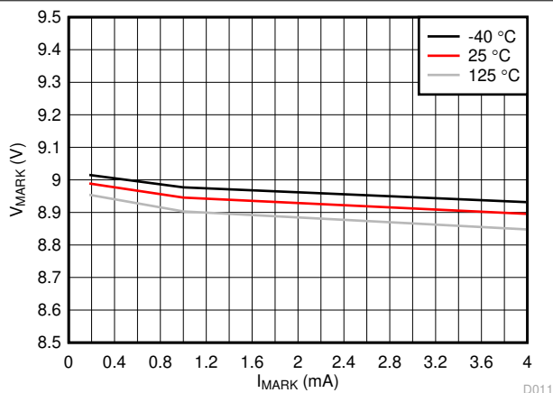
Figure 6-11. Mark Voltage vs I_{MARK} and Temperature
