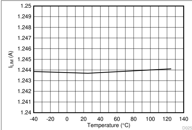
6-25. 2x Mode ( 2x\text{FBn} = 1 ) Current Limit vs Temperature
