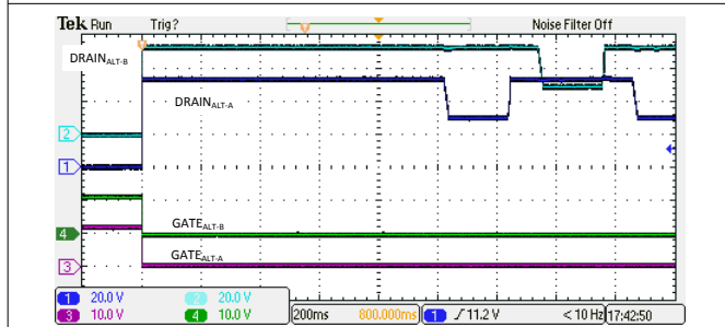
図 9-8. 4-Pair Backoff Due to 4PPCut Fault
