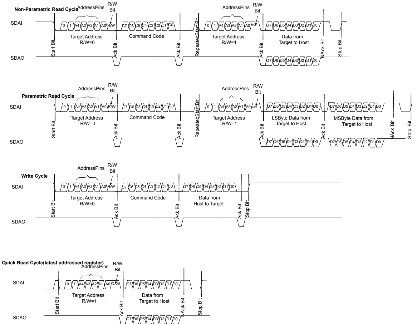
図 8-6. I 2 C interface Read and Write Protocol – Configuration A
