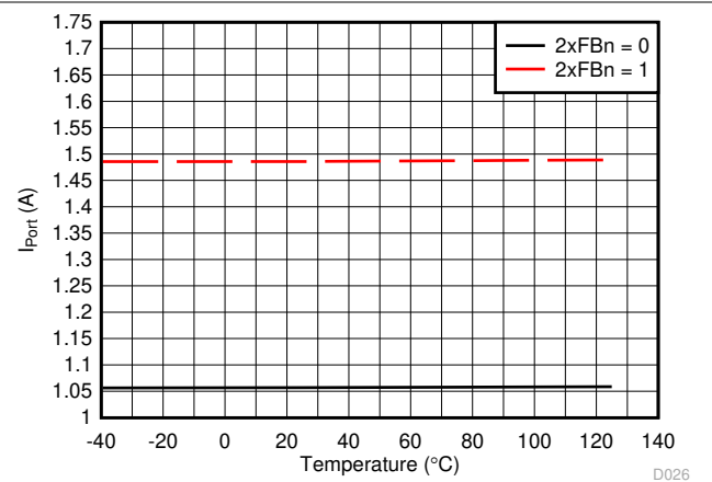
6-26. I_{\text{SHORT}} Threshold vs Temperature
