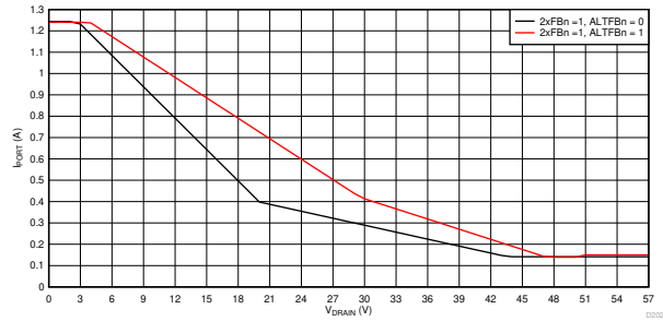
8-57. 2x Mode (2xFBn = 1) Foldback Curves, I PORT VS V DRAIN
