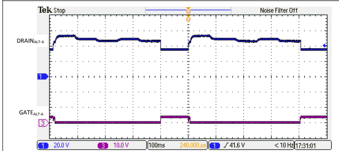
図 9-14. 2-Pair Semiauto Mode Discovery with a Valid Class 0-3 Load
