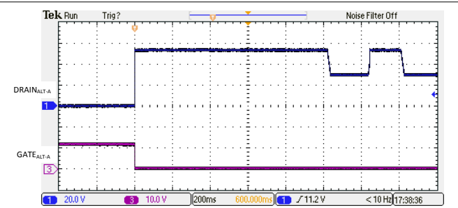
図 9-5. 2-Pair Backoff Due to PCut Fault
