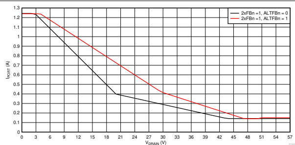
図 8-80. 2x Mode (2xFBn = 1) Foldback Curves, I PORT VS V DRAIN
