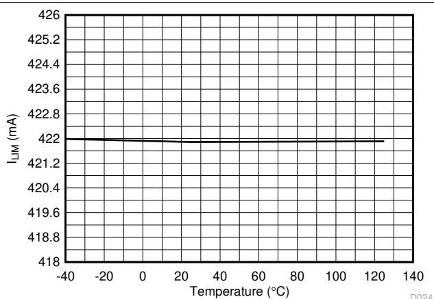
Figure 6-24. 1x Mode (2xFBn = 0) Current Limit vs Temperature
