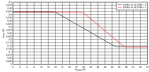
8-56. 1x Mode (2xFBn = 0) Foldback Curves, I PORT VS V DRAIN
