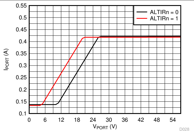
6-28. Inrush Current Foldback vs Port Voltage
