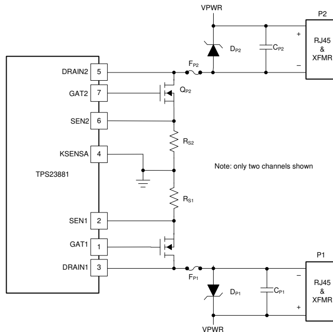
図 9-28. Kelvin Current-Sense Connection
