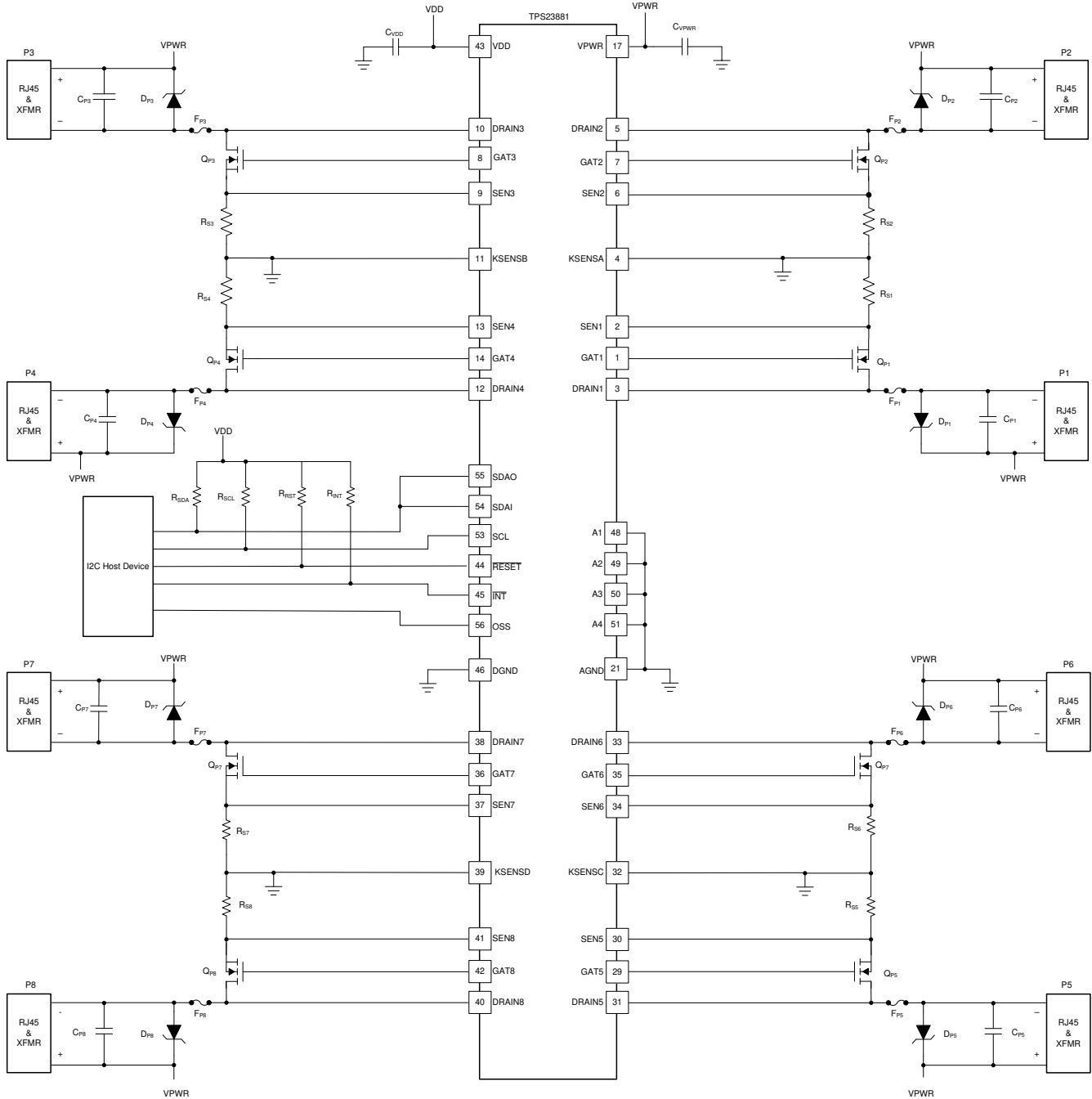
図 9-1. Eight 2-Pair Port Application
