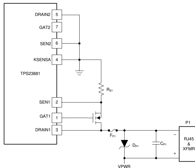
☒ 9-3. Unused PORT2 Connections
