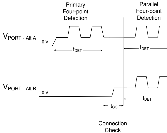
图 8-5. 4-Pair Port, Detection and Connection Check Waveforms with a Dual Signature Load
