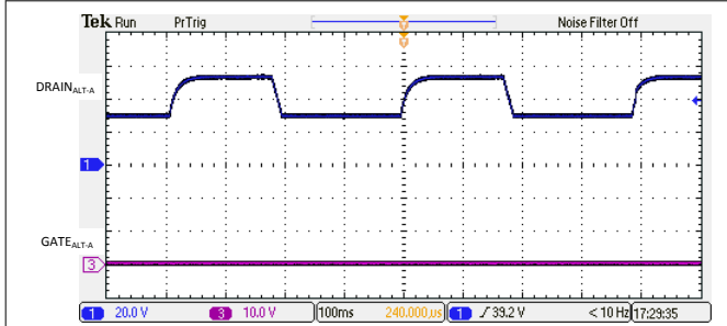
図 9-10. 2-Pair Open Circuit Detection Signature
