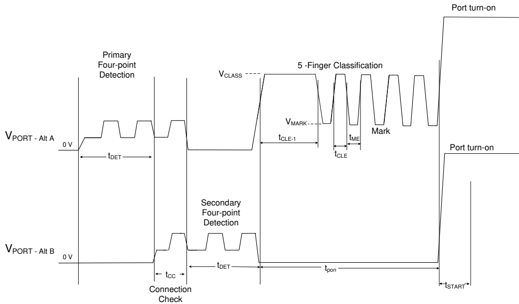
図 7-6. 4-Pair Single Signature Detection, 5-Event Classification and Turn-On
