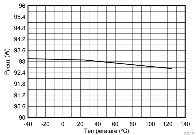
Figure 6-22. 4-Pair PCut Threshold (90W) vs Temperature
