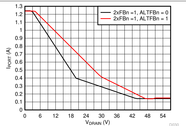
6-30. 2x Mode ( 2x\text{FBn} = 1 ) Current Foldback vs Drain Voltage
