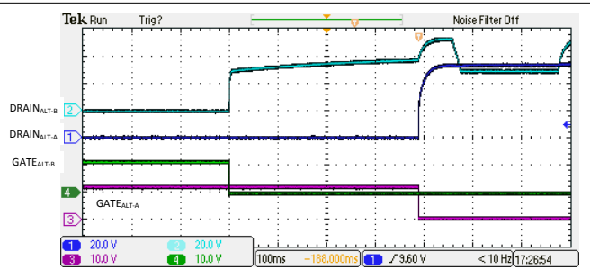
図 9-9. 4-Pair Single Signature Class 0-4 Disconnect
