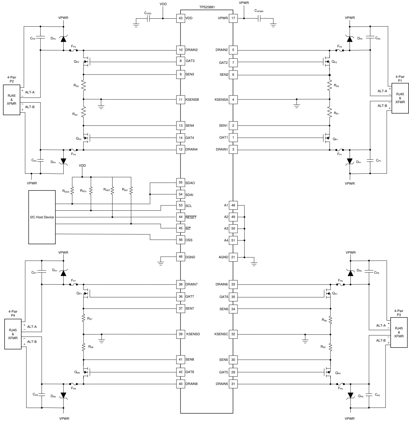
9-2. Four 4-Pair Port Application
