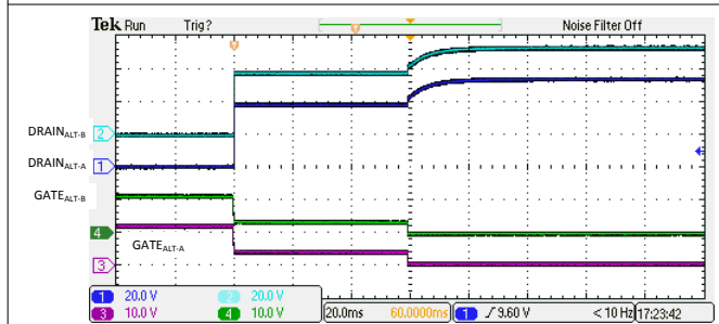
図 9-6. 4-Pair I_{LIM} Foldback and Turn Off
