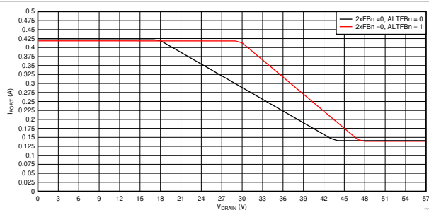
図 8-79. 1x Mode (2xFBn = 0) Foldback Curves, I PORT VS V DRAIN
