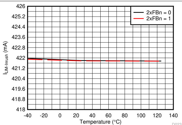
Figure 6-23. Inrush Current Limit vs Temperature
