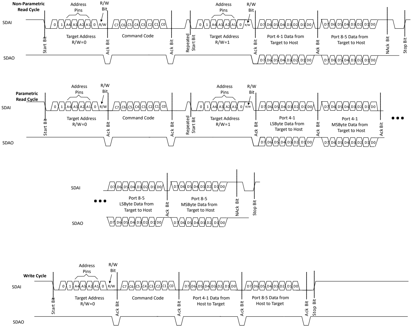
図 8-7. I 2 C interface Read and Write Protocol – Configuration B
