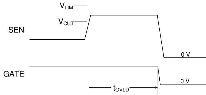
図 7-2. Overcurrent Fault Timing
