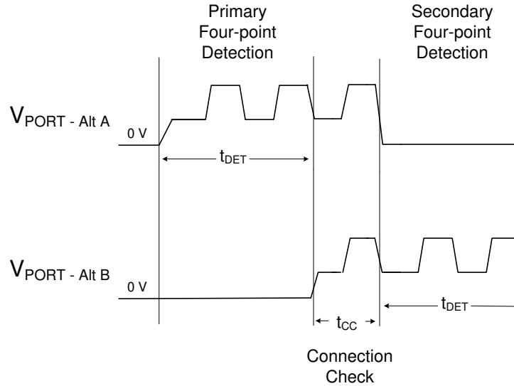
图 8-4. 4-Pair Port, Detection and Connection Check Waveforms with a Single Signature Load
