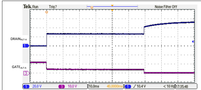
図 9-4. 2-Pair I_{LIM} Foldback and Turn-Off
