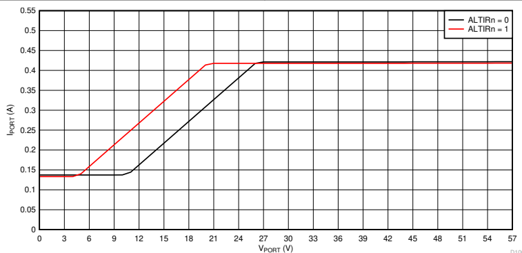
図 8-81. Inrush Foldback Curves, I PORT VS V PORT
