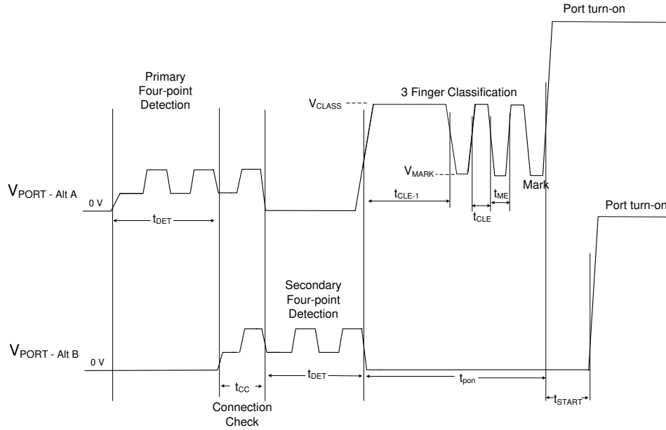
図 7-5. 4-Pair Single Signature Detection, 3-Event Classification and Turn On
