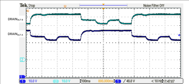
図 9-13. 4-Pair High Resistance (36kΩ) Detection Signature
