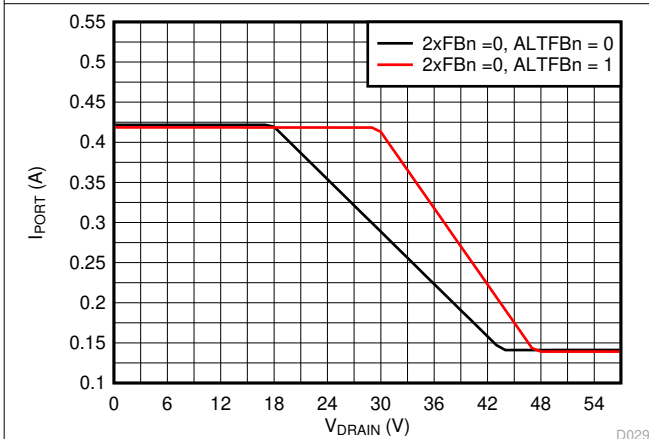
6-29. 1x Mode ( 2x\text{FBn} = 0 ) Current Foldback vs Drain Voltage
