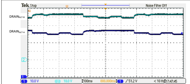
図 9-12. 4-Pair Low Resistance (11kΩ) Detection Signature
