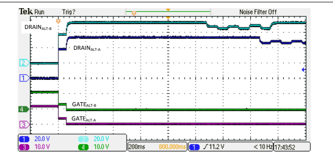
図 9-7. 4-Pair Backoff Due to I_{LIM} Fault
