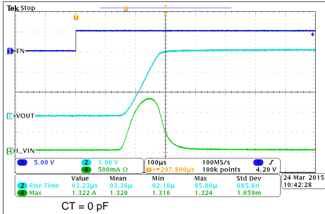
Figure 66. Inrush with CT = 0 pF
