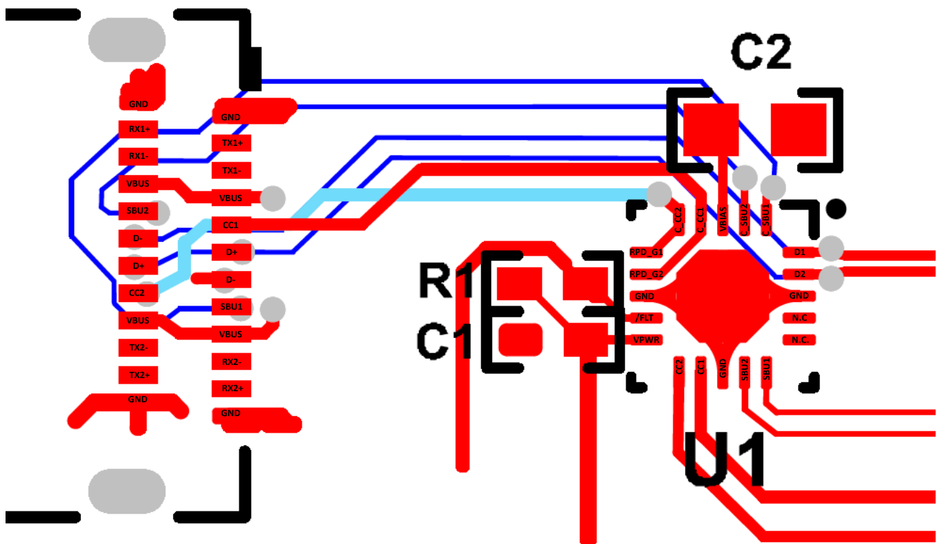
34. TPD6S300A Typical Layout
