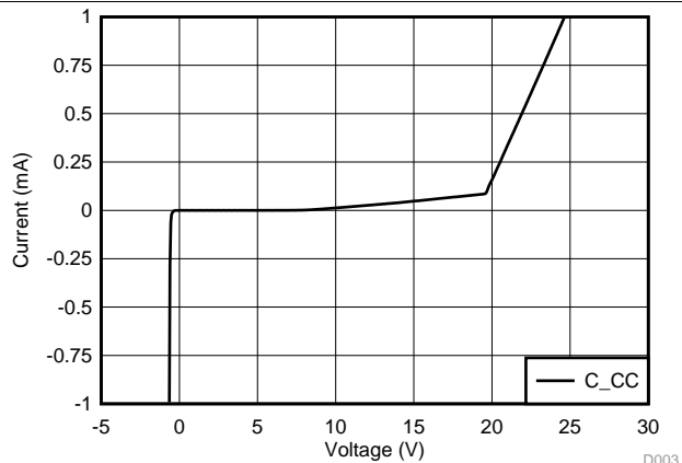
24. C_CC IV Curve
