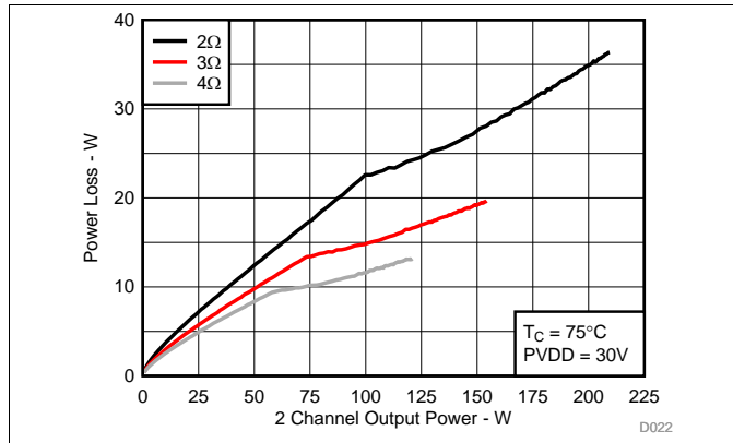
Figure 23. System Power Loss vs Output Power, AD-mode
