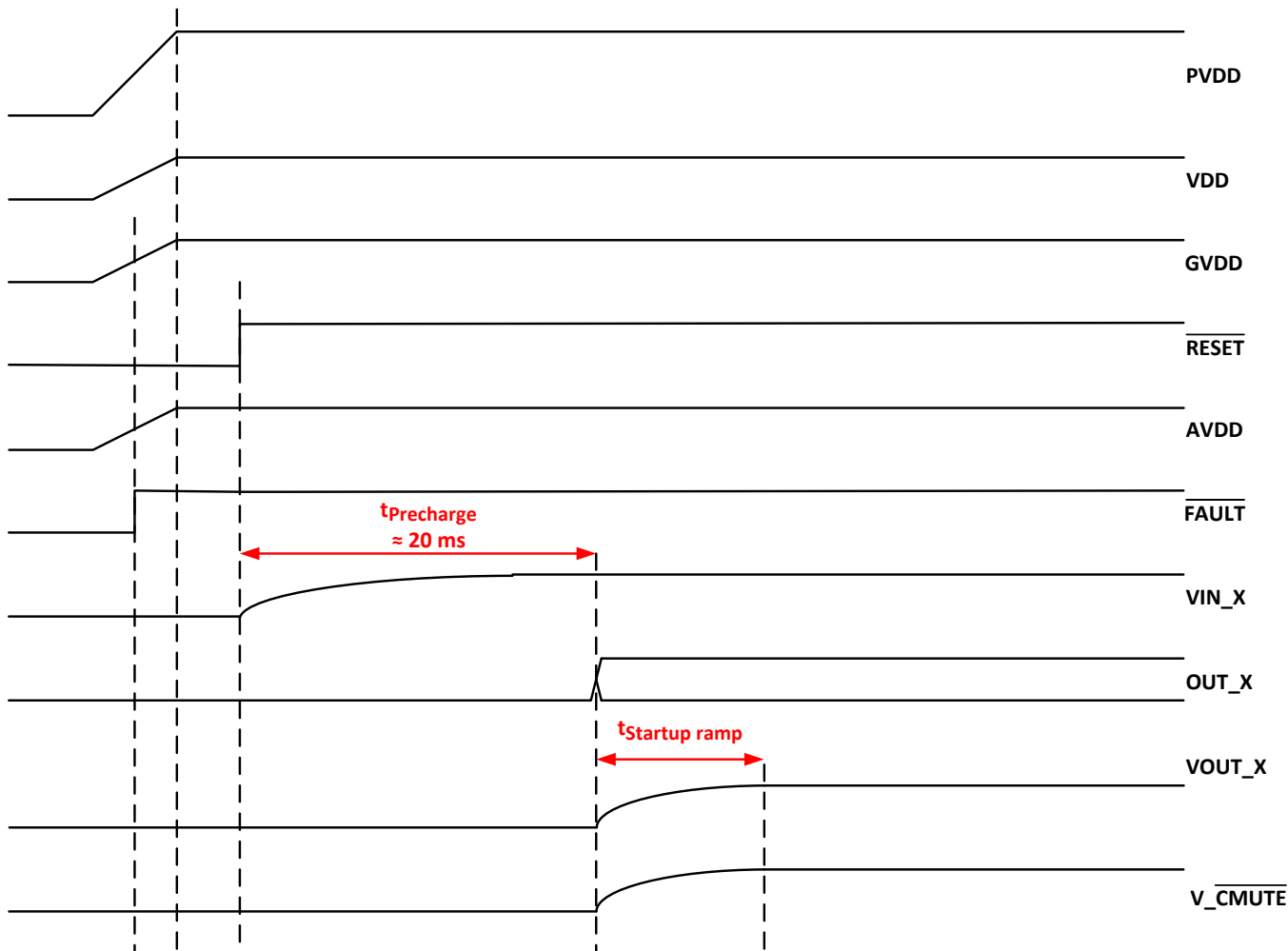
47. Startup Timing
