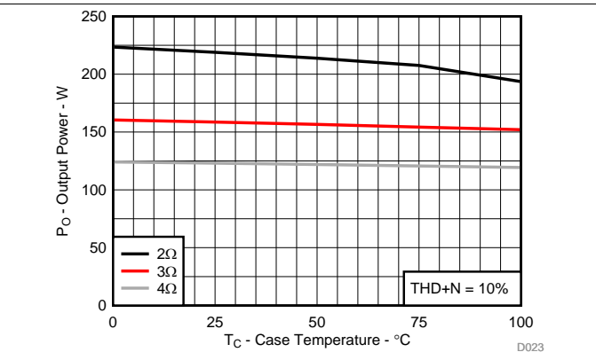
Figure 24. Output Power vs Case Temperature, AD-mode
