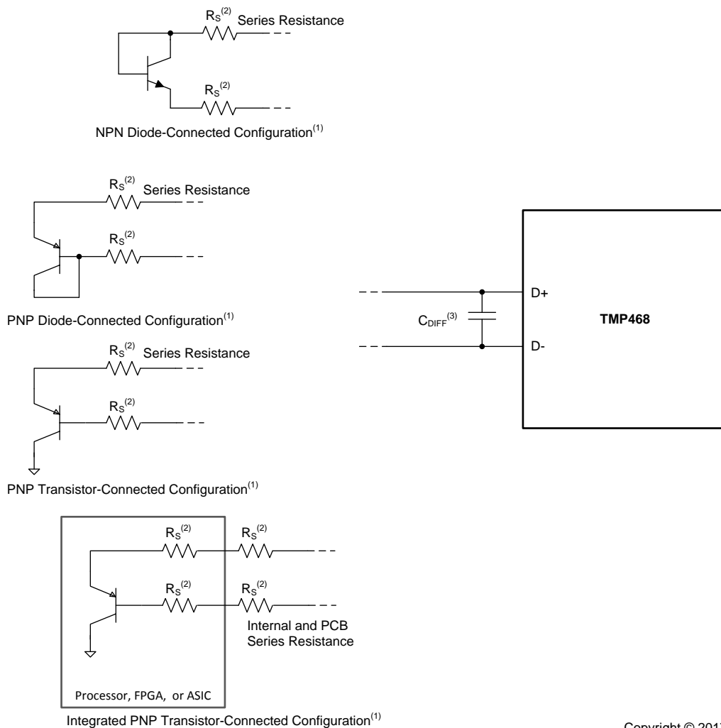
✎ 23. TMP468 Remote Transistor Configuration Options
