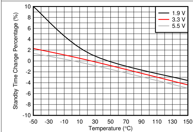
6-10. Standby Time vs Temperature
