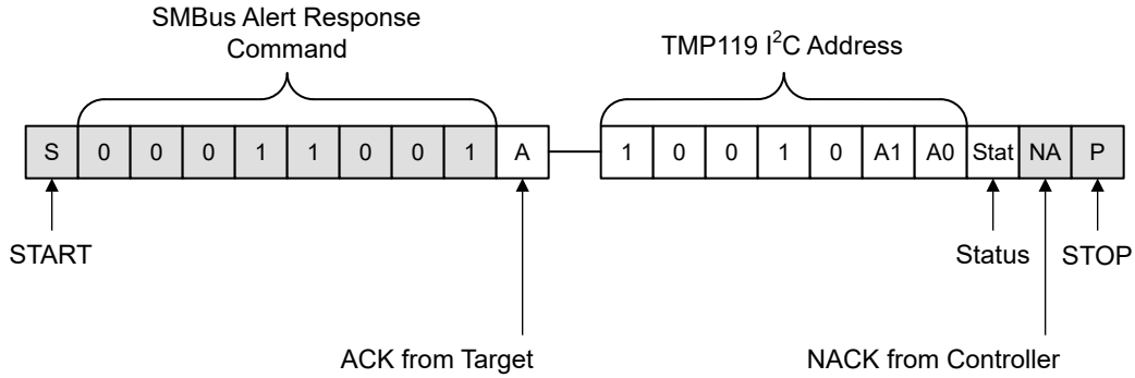
7-12. SMBus ALERT Timing Diagram
