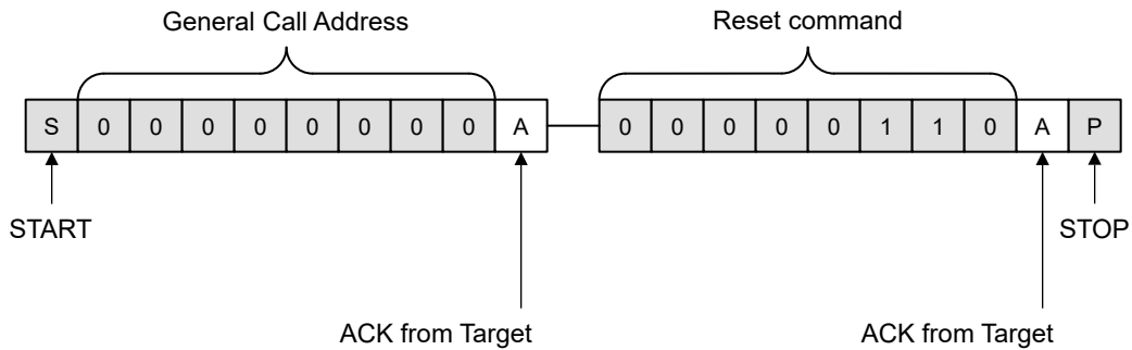
7-13. General-Call Reset Command Timing Diagram
