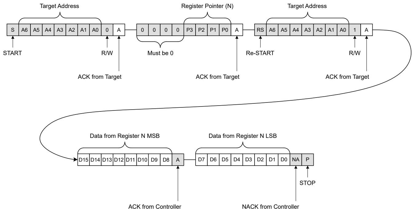
7-11. Read Word Command Timing Diagram
