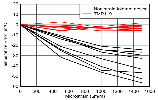
图 6-13. Temperature Error vs Microstrain
