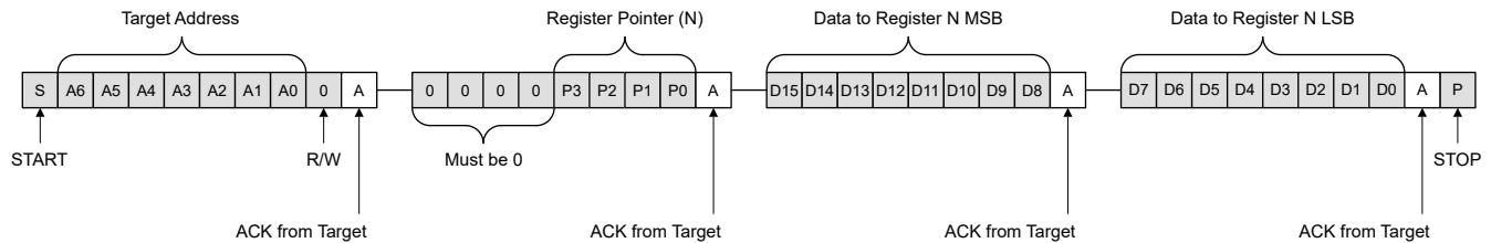
7-10. Write Word Command Timing Diagram
