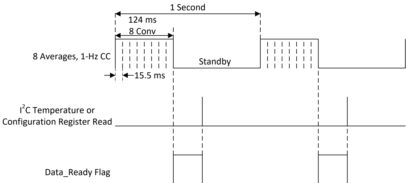
図 7-2. Averaging Timing Diagram
