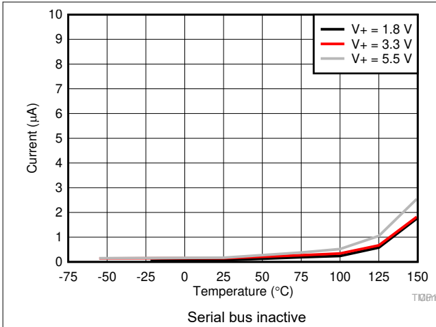
6-6. Quiescent Current in Shutdown Mode
