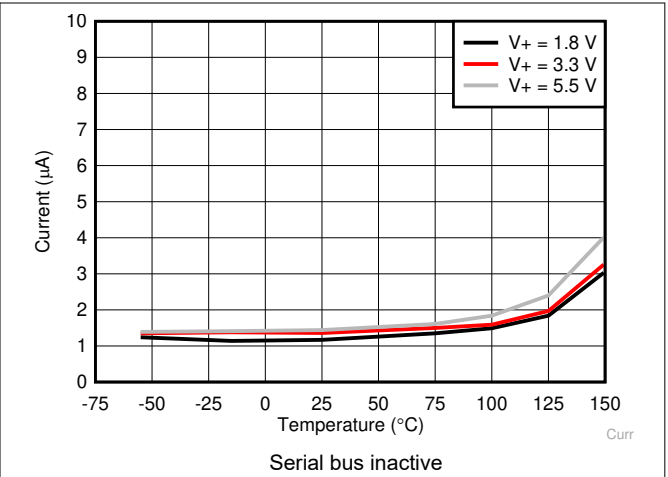
6-7. Quiescent Current in Standby Mode
