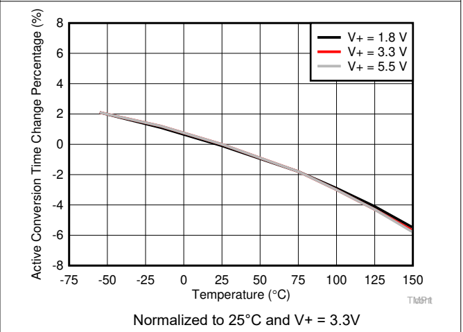
6-9. Active Conversion Time vs Temperature
