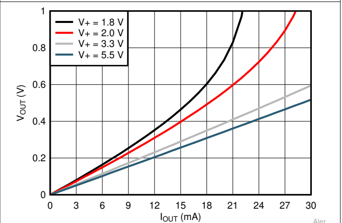
6-11. ALERT Pin Output Voltage vs Pin Sink Current
