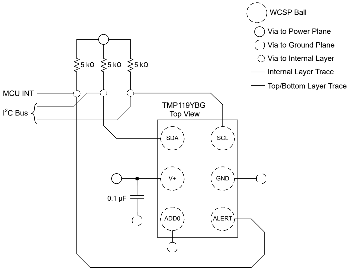
図 8-5. YBG Layout Recommendation
