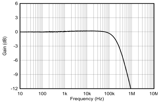
6-11. Sensitivity vs Frequency, All Gains Normalized to 1Hz
