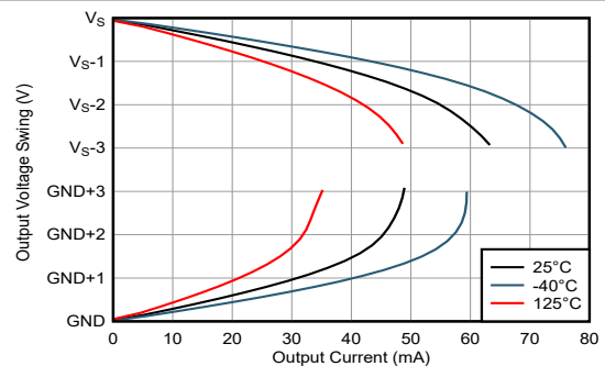
6-20. Output Swing vs Output Current
