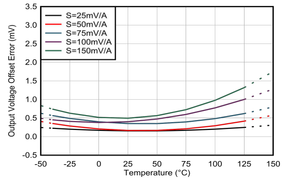
6-2. Offset Error vs Temperature
