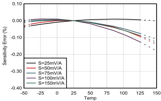
6-1. Sensitivity Error vs Temperature
