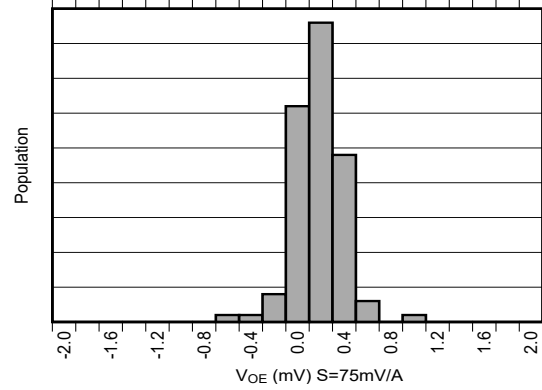
6-8. Offset Error Production Distribution
