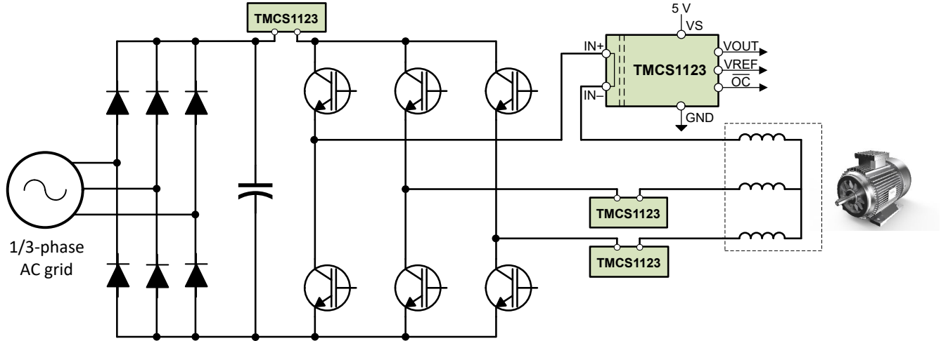
図 9-2. Inline Motor Phase Current Sensing
