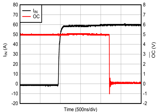
6-17. Overcurrent Output Response With MASK
