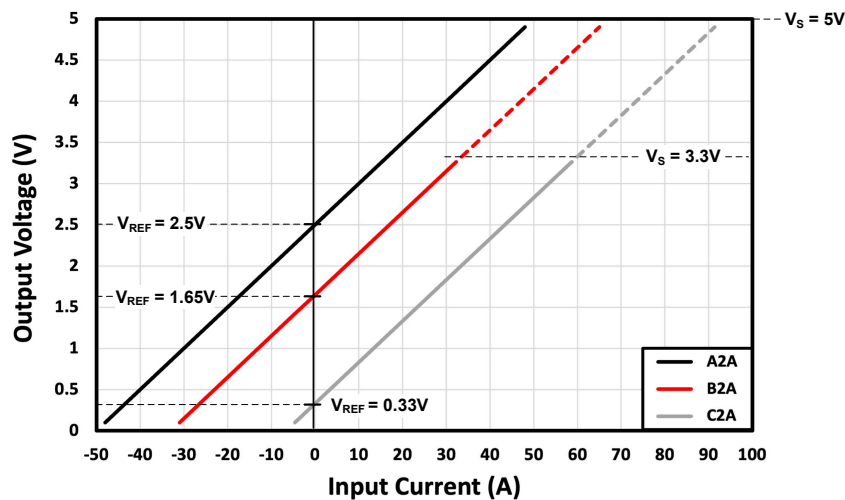
Figure 8-5. Output Voltage Relationship to Input Current for TMCS1123x2A
