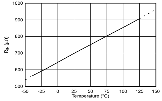
6-22. Input Conductor Resistance vs Temperature
