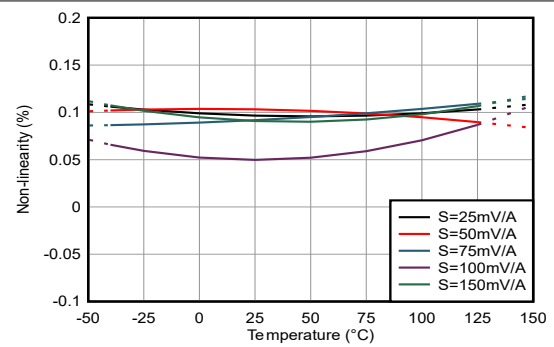
6-4. Non-Linearity vs Temperature
