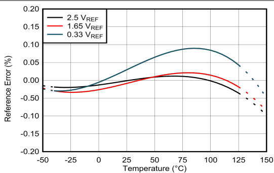
6-3. Reference Error vs Temperature
