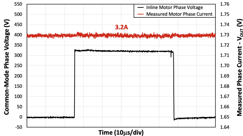
☒ 9-3. Inline Motor Current-Sense Input and Output Signals
