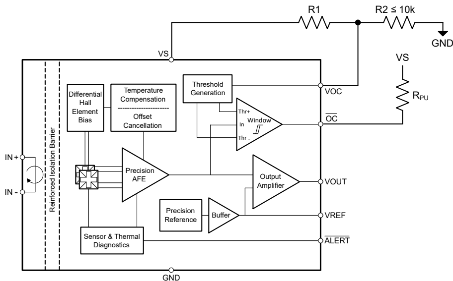
図 8-6. User Configurable Overcurrent Threshold Using Power Supply Voltage
