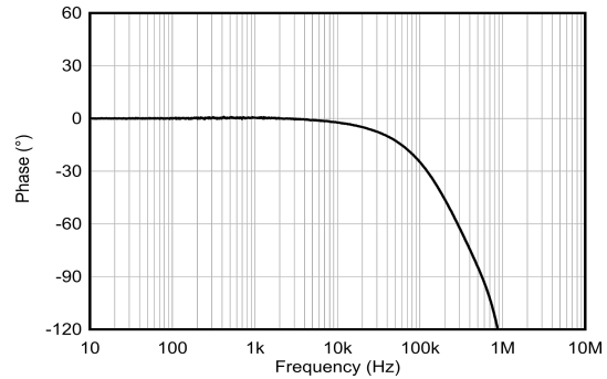
6-12. Phase vs Frequency, All Gains
