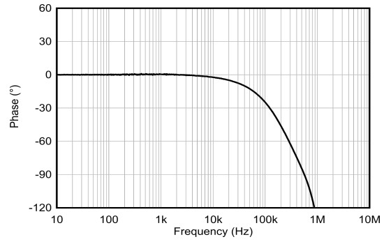
6-12. Phase vs Frequency, All Gains
