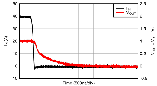
6-16. Voltage Output Step Response, Falling
