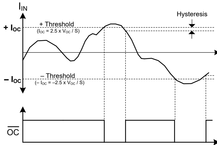
图 8-8. Overcurrent Output Response
