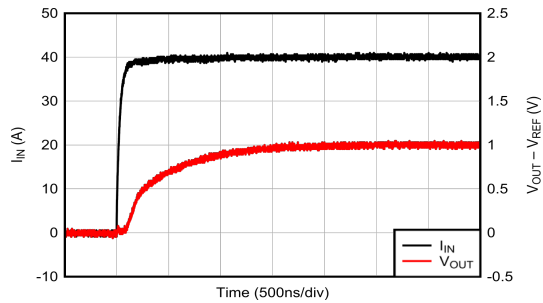
6-15. Voltage Output Step Response, Rising
