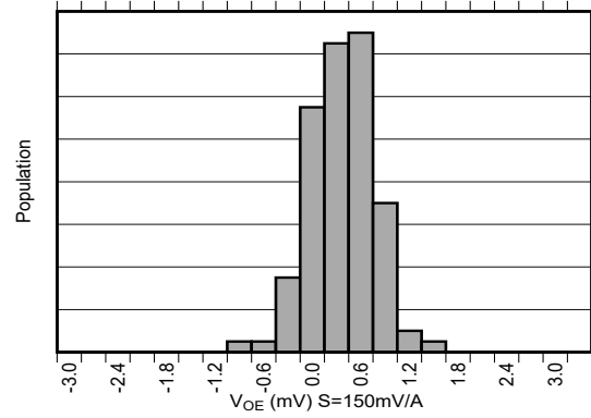
6-10. Offset Error Production Distribution
