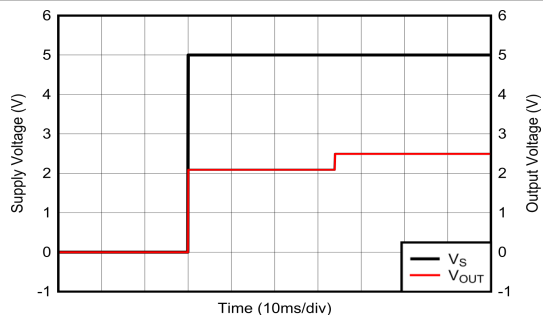
6-19. Startup Transient Response
