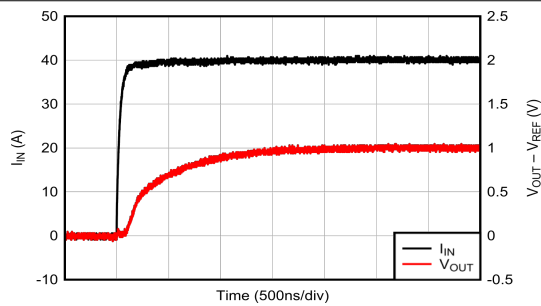
6-15. Voltage Output Step Response, Rising
