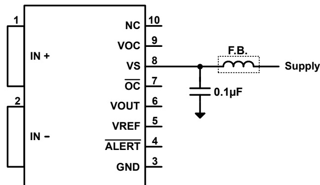
☒ 9-4. Power Supply Noise Filtering
