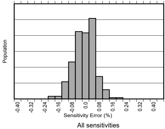
6-5. Sensitivity Error Production Distribution
