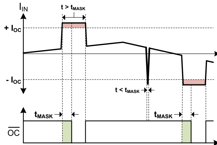
図 8-8. Overcurrent Detection MASK Diagram
