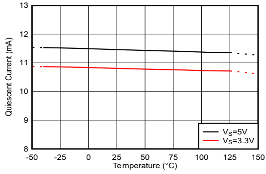
6-21. Quiescent Current vs Temperature
