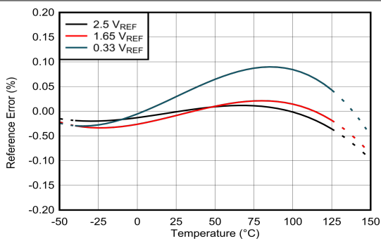
6-3. Reference Error vs Temperature
