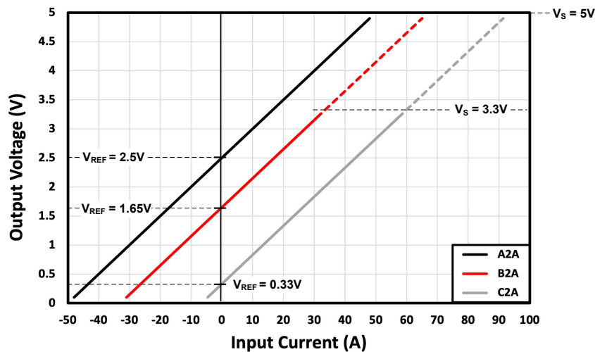
図 8-4. Output Voltage Relationship to Input Current for TMCS1123x2A
