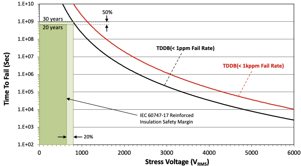
☒ 8-2. Insulation Lifetime
