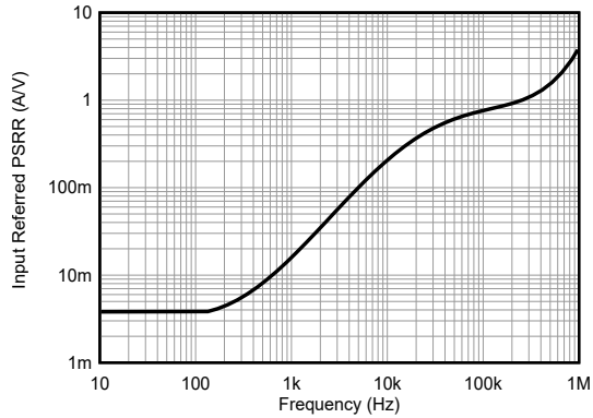
6-13. PSRR vs Frequency
