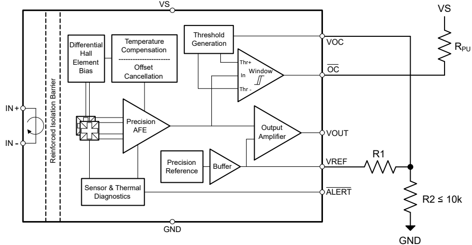
图 8-7. User Configurable Overcurrent Threshold Using Zero Current Output Reference Voltage
