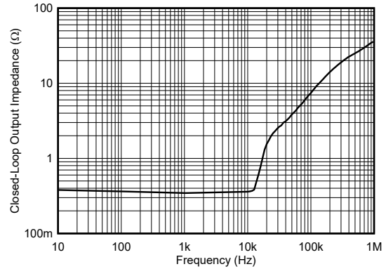
6-14. Output Impedance vs Frequency
