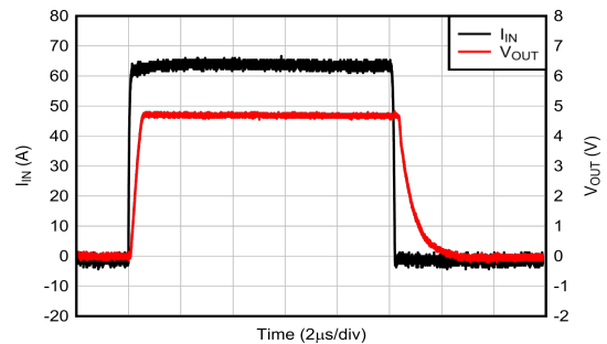
6-18. Current Overload Response
