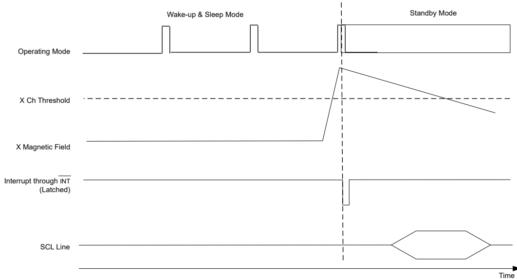
☒ 7-11. Wake-Up and Sleep Mode Operation With Back-Up Battery
