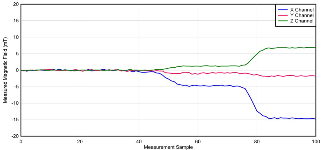
☒ 7-12. Tamper Detection During Continuous Conversion
