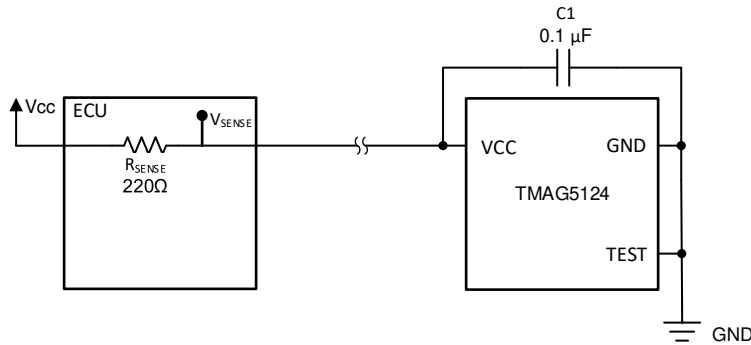
図 9-1. Typical High-Side Sensing Diagram
