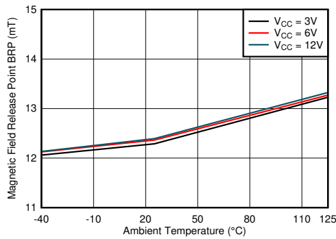
7-21. B RP vs Temperature
