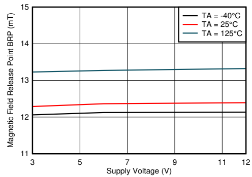
7-22. B RP vs V CC
