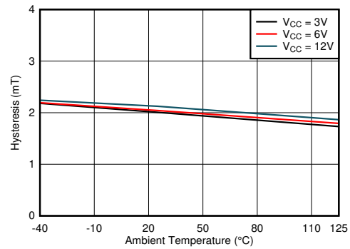
7-23. Hysteresis vs Temperature
