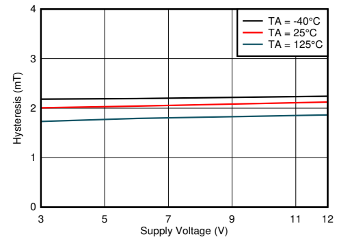
7-24. Hysteresis vs V CC
