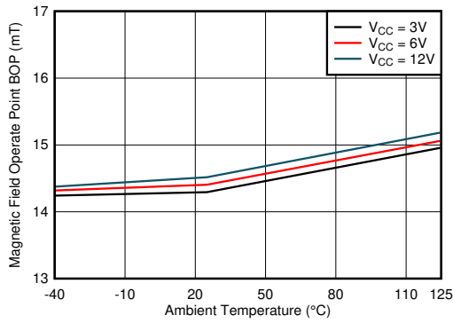
7-19. B OP vs Temperature
