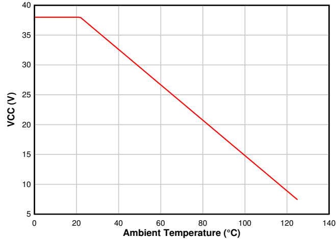
☒ 10-1. Power Derating Curve
