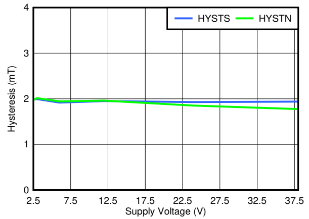
7-10. TMAG5123C Hysteresis vs Supply Voltage
