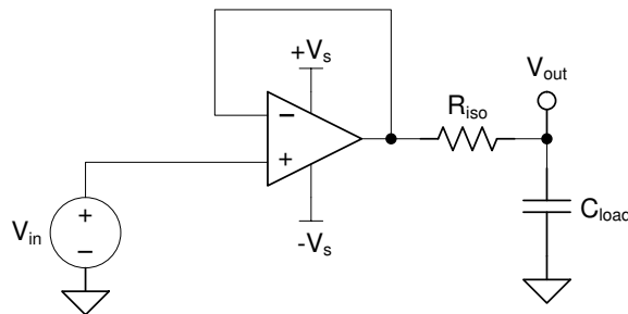
図 6-5. Extending Capacitive Load Drive With the TLV9361-Q1
