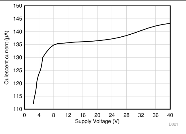
6-22. Quiescent Current vs Supply Voltage
