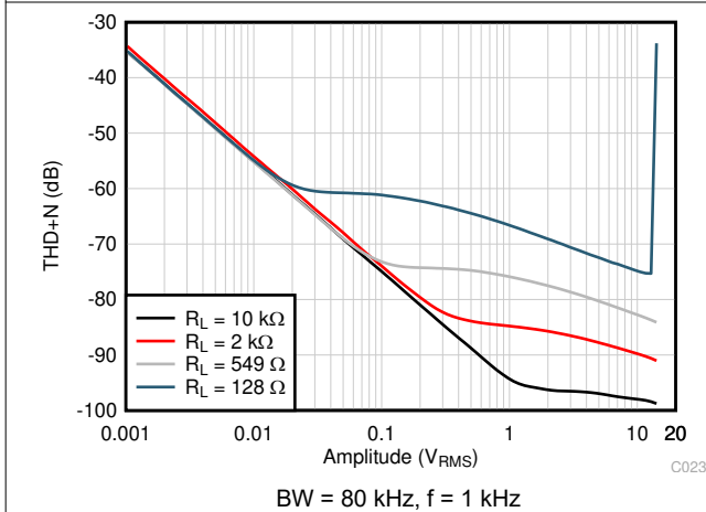
6-21. THD+N vs Output Amplitude
