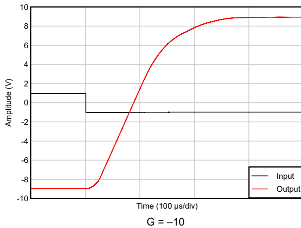
图 5-37. Overload Recovery (Negative)
