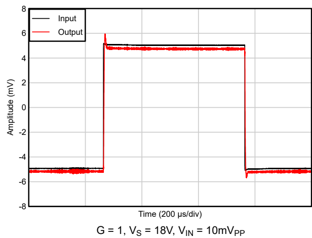
图 5-40. Small-Signal Step Response
