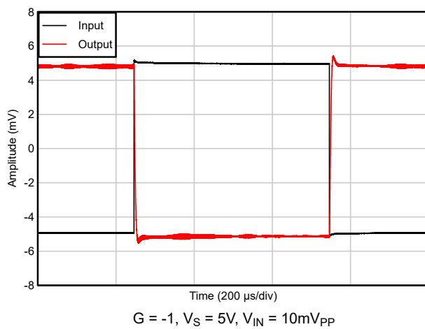
图 5-39. Small-Signal Step Response
