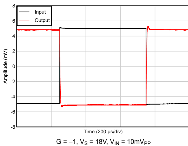
图 5-41. Small-Signal Step Response
