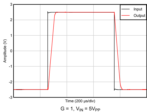
图 5-42. Large-Signal Step Response
