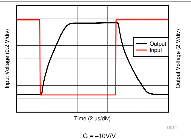
Figure 6-22. Overload Recovery
