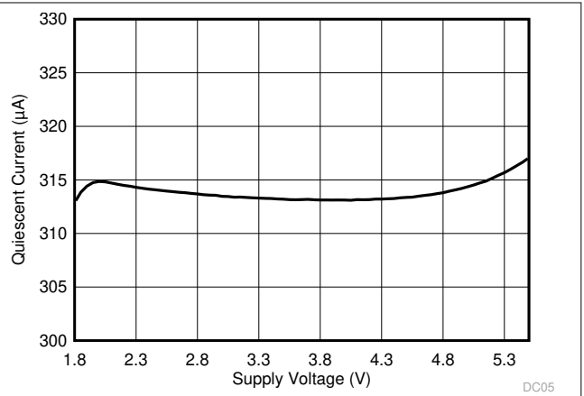
6-34. Quiescent Current vs Supply Voltage
