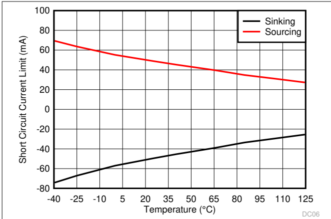
6-33. Short-Circuit Current vs Temperature
