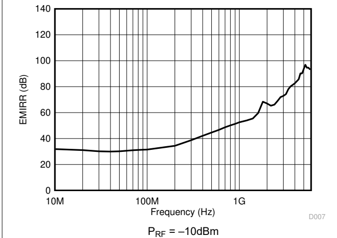
6-37. Electromagnetic Interference Rejection Ratio Referred to Noninverting Input (EMIRR+) vs Frequency
