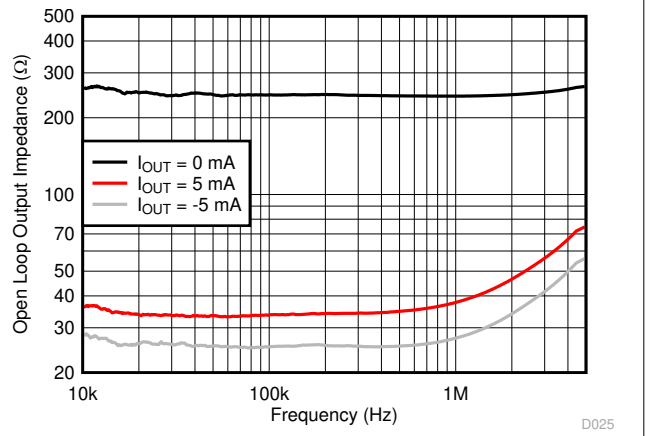
6-36. Open-Loop Output Impedance vs Frequency
