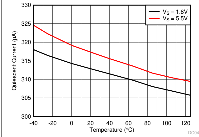
6-35. Quiescent Current vs Temperature
