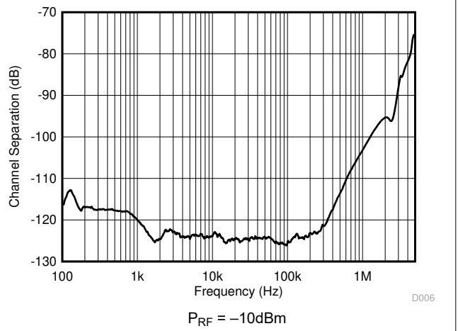
6-38. Channel Separation vs Frequency
