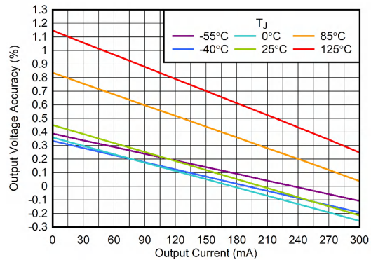
图 5-4. Output Voltage Accuracy vs I_{OUT}
