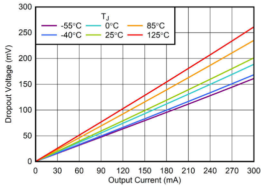
图 5-5. Dropout Voltage vs I_{OUT}
