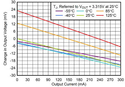
图 5-2. Load Regulation vs I_{OUT}
