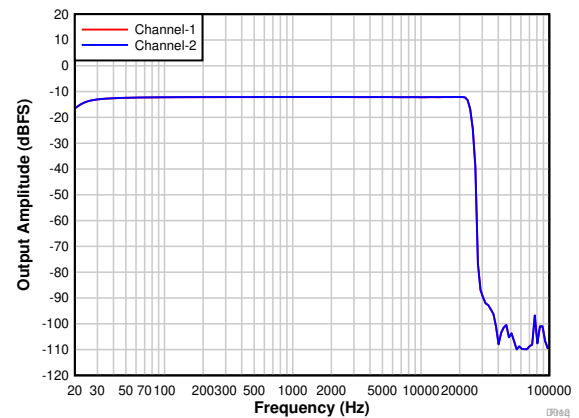
7-15. Frequency Response With a -12\text{-dBr} Input
