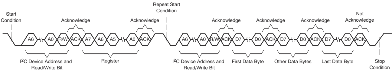
FIG 8-70. I 2 C Multiple-Byte Read Transfer
