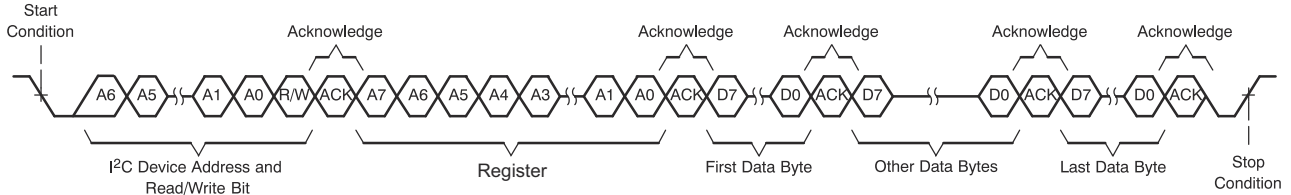
FIG 8-68. I 2 C Multiple-Byte Write Transfer
