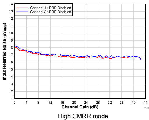
7-24. Input-Referred Noise vs Channel Gain
