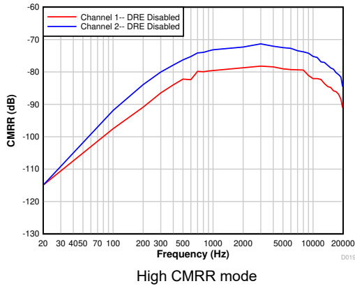
7-22. Common-Mode Rejection Ratio vs Ripple Frequency With 100-mV pp Amplitude and DRE Disabled
