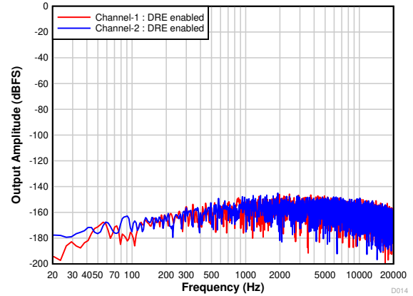
7-17. FFT With Idle Input With DRE Enabled
