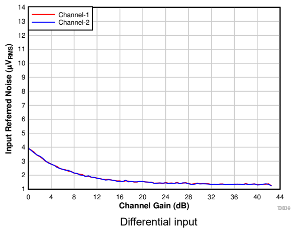
7-13. Input-Referred Noise vs Channel Gain
