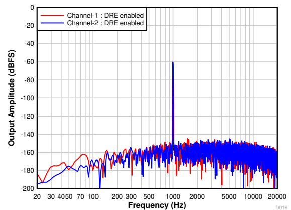
7-19. FFT With a -60-dBr Input With DRE Enabled
