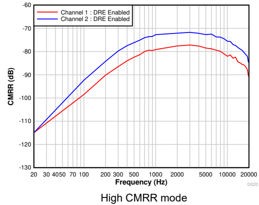
7-23. Common-Mode Rejection Ratio vs Ripple Frequency With 100-mV pp Amplitude and DRE Enabled
