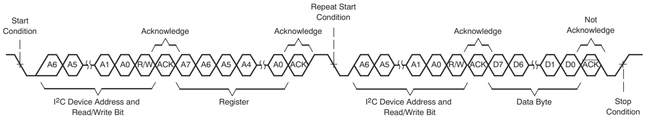
FIG 8-69. I 2 C Single-Byte Read Transfer
