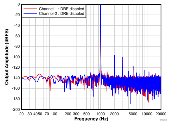
7-21. FFT With a -1-dBr Input With DRE Disabled
