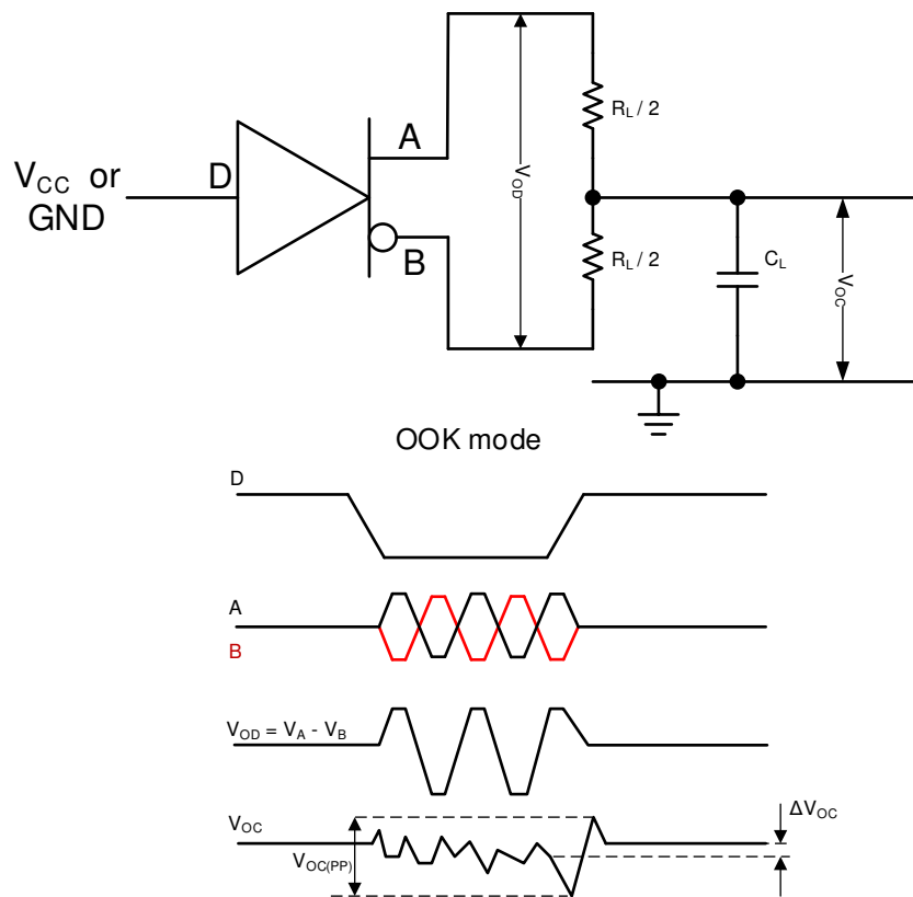
☒ 7-2. Measurement of Driver Differential and Common-Mode Outputs
