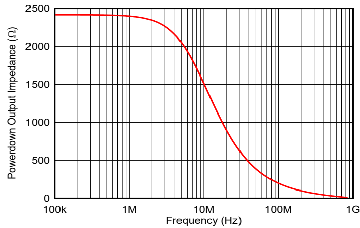
☒ 8-1. Power-Down Output Impedance vs Frequency
