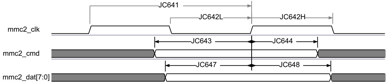
Figure 5-86. MMC/SD/SDIO in - High Speed JC64 - Receiver Mode
