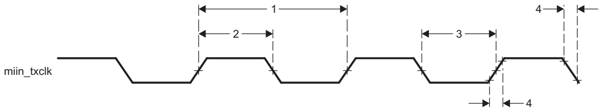
Figure 5-62. Clock Timing (GMAC Transmit) - MII in operation
