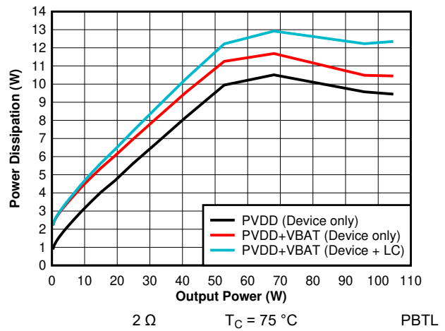
7-35. Power Dissipation vs Output Power - PBTL - 2 \Omega
