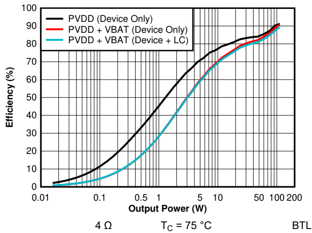
7-7. Efficiency vs Output Power - 14.4 V - 4 \Omega (Zoomed)
