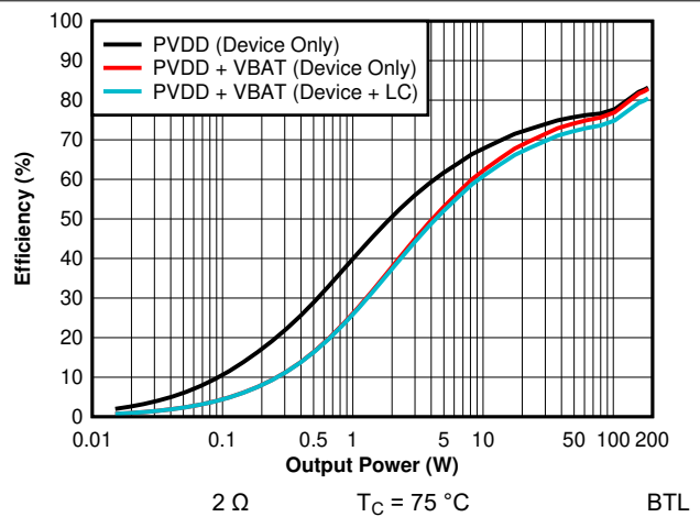
7-10. Efficiency vs Output Power - 14.4 V - 2 \Omega (Zoomed)
