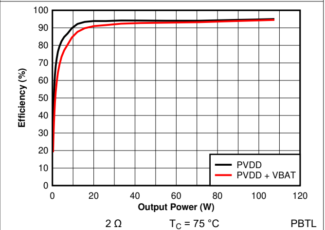
7-40. Efficiency vs Output Power - PBTL - 2 Ohm - 384 kHz
