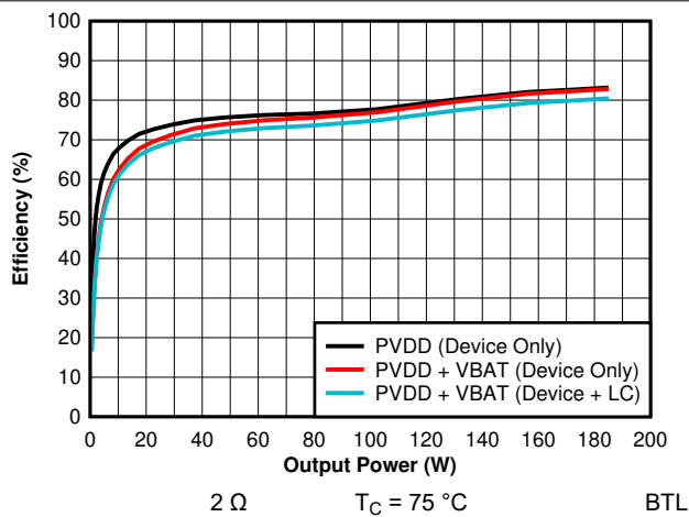
7-9. Efficiency vs Output Power - 14.4 V - 2 \Omega
