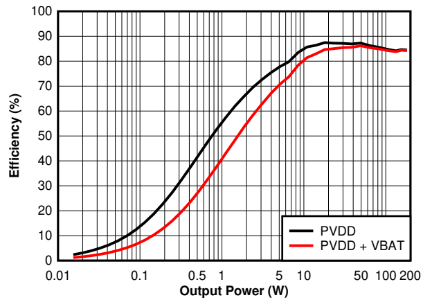
7-26. Efficiency vs Output Power - 2 \Omega - 384 kHz (Zoomed)
