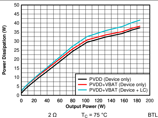
7-11. Power Dissipation vs Output Power - 14.4 V - 2 \Omega
