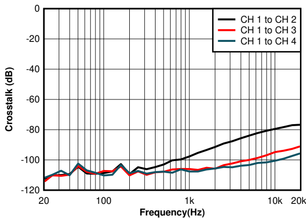
7-15. Crosstalk vs Frequency
