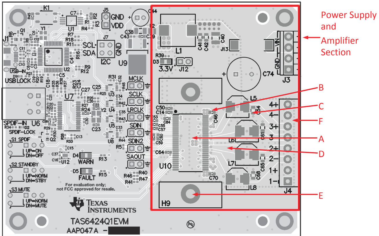
12-1. EVM Layout
