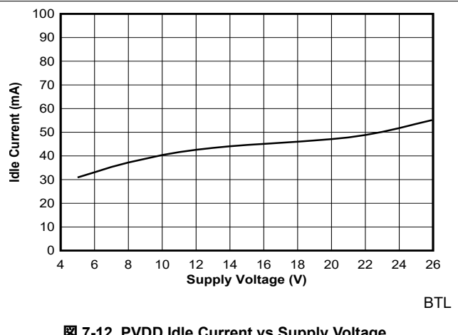
7-12. PVDD Idle Current vs Supply Voltage
