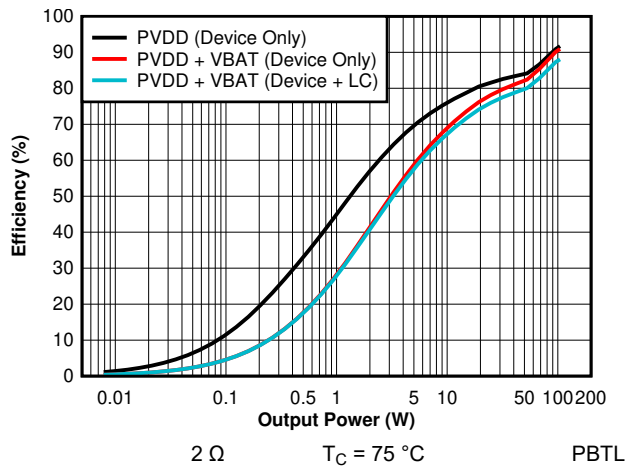
7-34. Efficiency vs Output power - PBTL - 2 \Omega (Zoomed)
