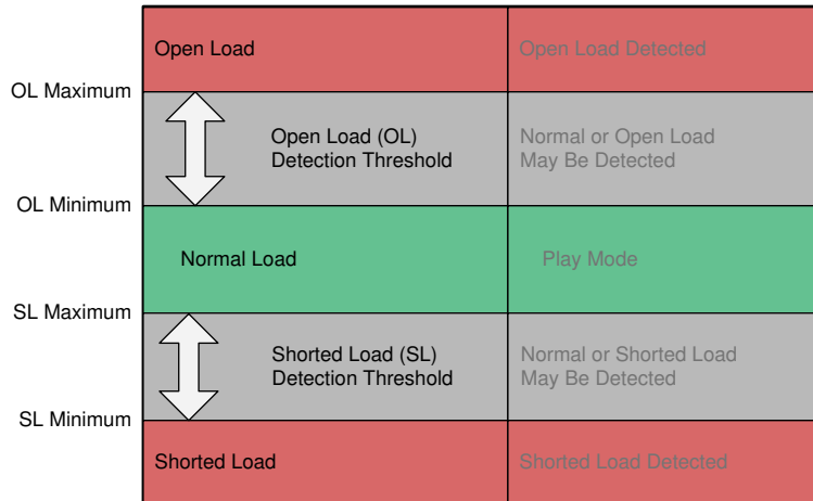
9-7. DC Load Diagnostic Reporting Thresholds
