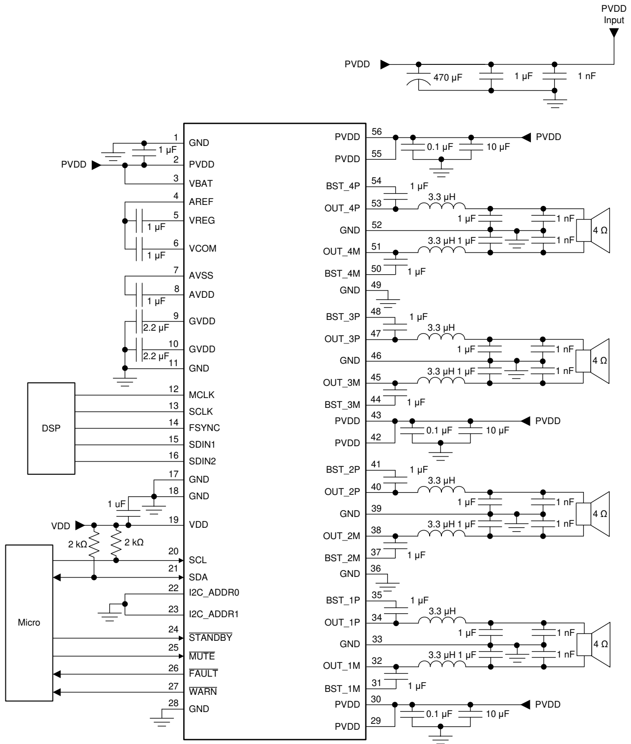
10-2. Typical 4-Channel BTL Application Schematic
