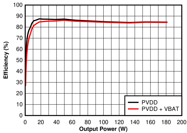
7-25. Efficiency vs Output Power - 2 \Omega - 384 kHz
