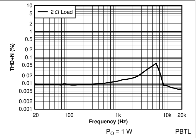
7-38. THD+N vs Frequency - PBTL - 384 kHz
