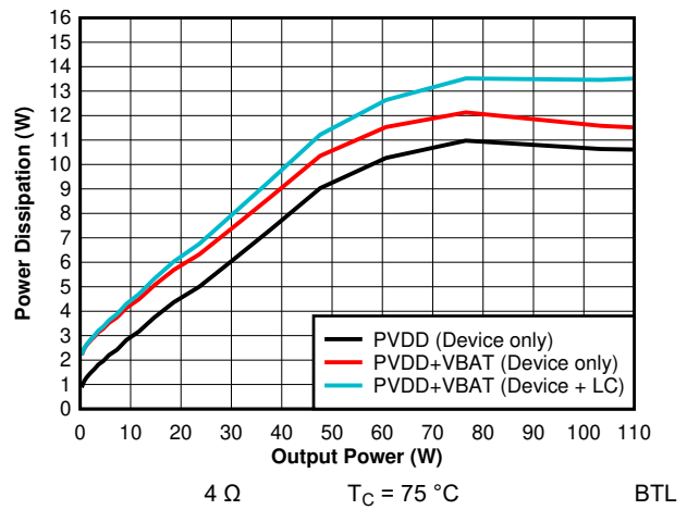
7-8. Power Dissipation vs Output Power - 14.4 V - 4 \Omega
