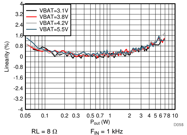
Figure 18. I-sense Linearity vs Output Power
