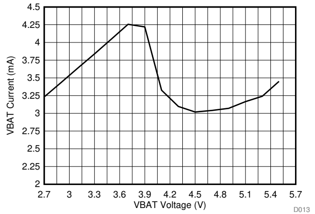
Figure 16. VBAT Idle Current vs VBAT
