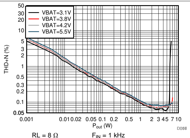
Figure 20. V-sense THD+N vs Output Power
