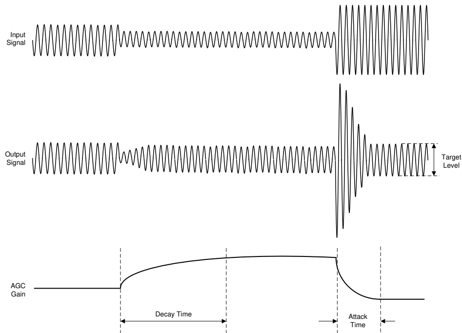
Figure 6-100. AGC Characteristics
