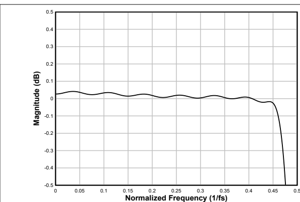
図 6-63. Linear-phase Decimation Filter Pass-Band Ripple
