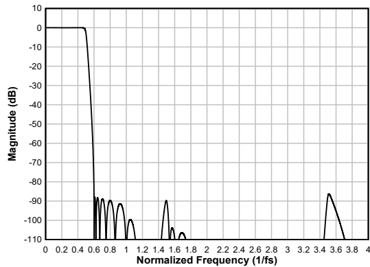
6-94. Ultra Low-latency Decimation Filter Magnitude Response
