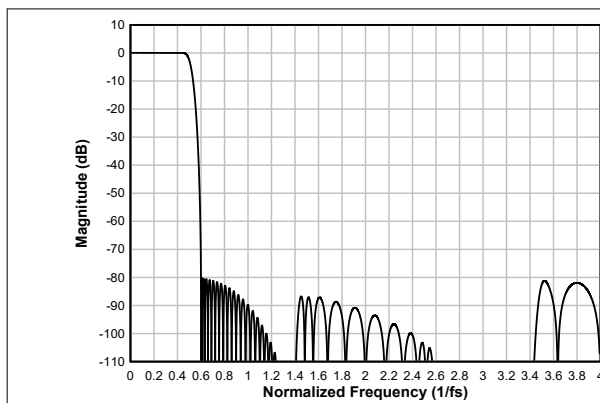
図 6-62. Linear-phase Decimation Filter Magnitude Response
