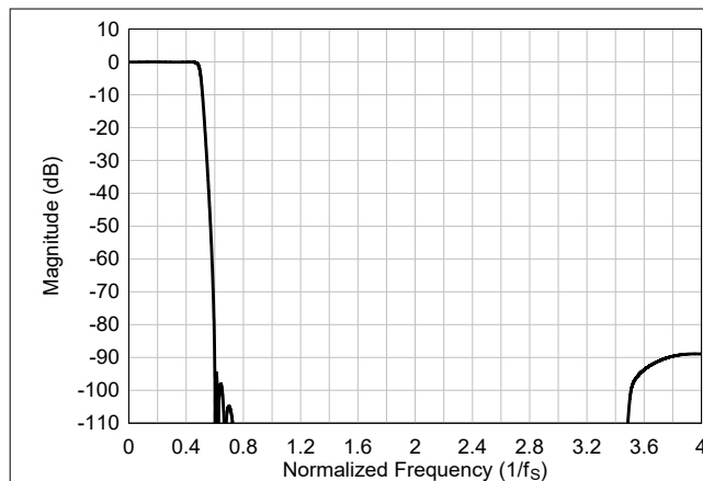
☒ 6-52. Ultra-Low-Latency interpolation Filter Magnitude Response
