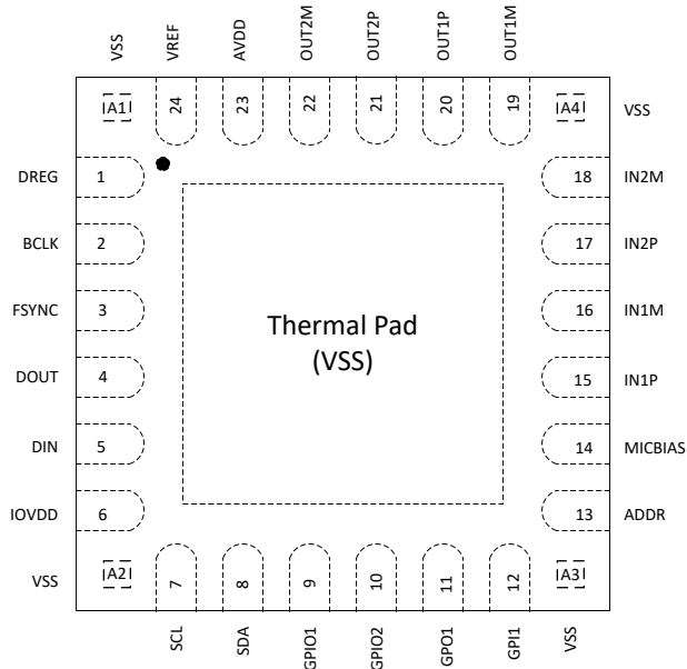
图 4-1. 24-Pin QFN Package with Exposed Thermal Pad and Corner Pins, Top View
