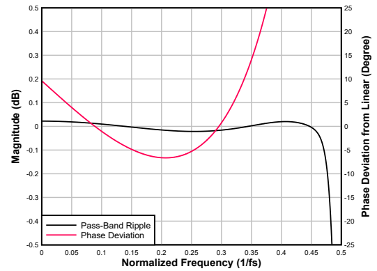
6-95. Ultra Low-latency Decimation Filter Pass-Band Ripple and Phase Deviation
