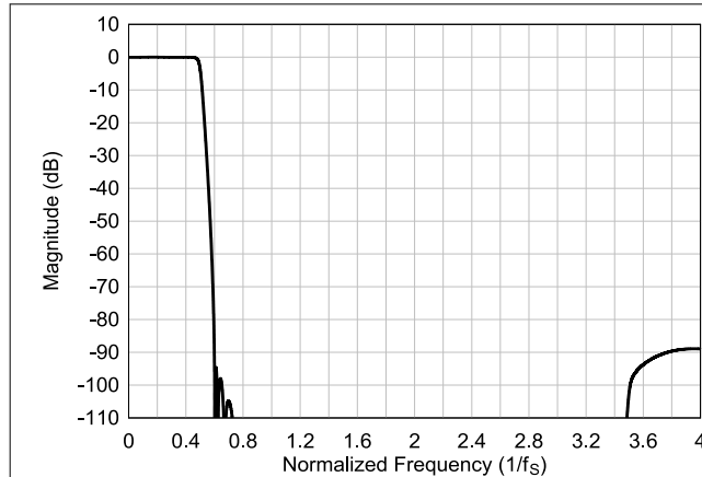
☒ 6-50. Ultra-Low-Latency interpolation Filter Magnitude Response
