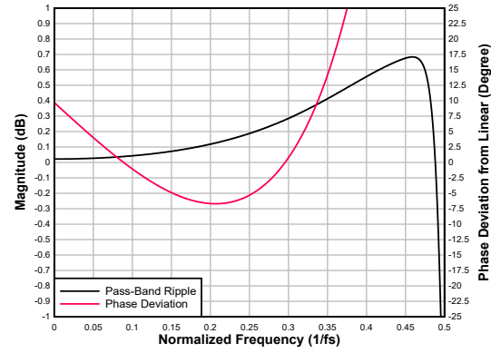
6-93. Ultra Low-latency Decimation Filter Pass-Band Ripple and Phase Deviation
