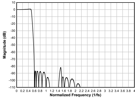
6-92. Ultra Low-latency Decimation Filter Magnitude Response
