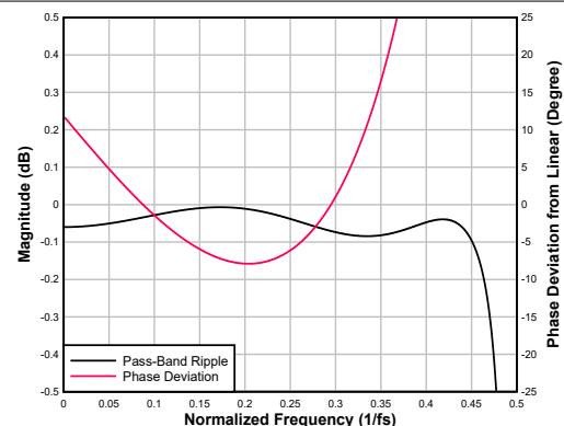
☒ 6-53. Ultra-Low-Latency interpolation Filter Pass-Band Ripple and Phase Deviation
