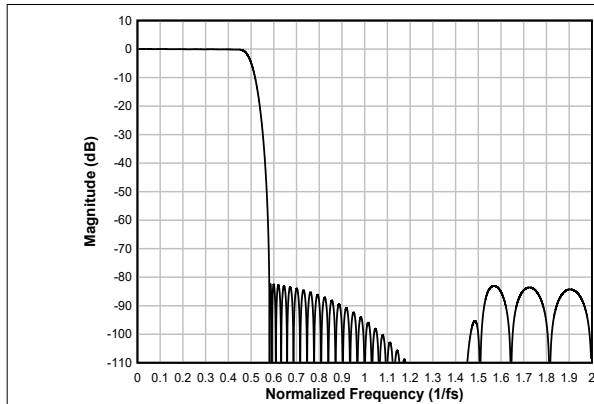
図 6-32. Linear-phase Interpolation Filter Magnitude Response
