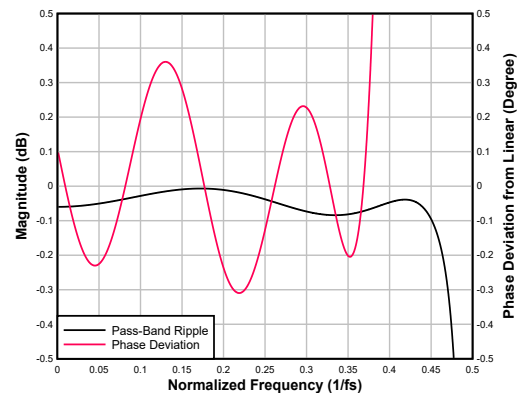
図 6-46. Low-latency Interpolation Filter Pass-Band Ripple and Phase Deviation
