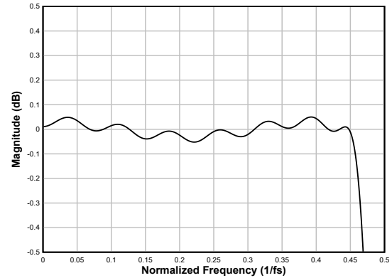
図 6-72. Linear-phase Decimation Filter Pass-Band Ripple
