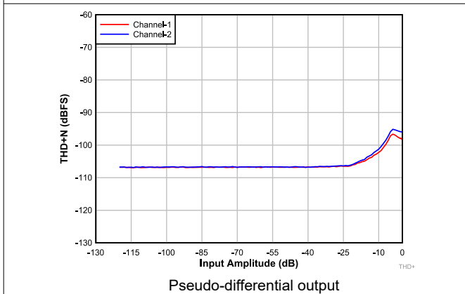
5-7. DAC THD+N Level vs Input
