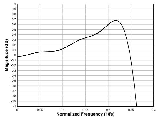
図 6-38. Linear-phase Interpolation Filter Pass-Band Ripple
