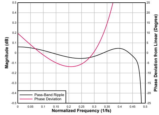
6-100. Ultra Low-latency Decimation Filter Pass-Band Ripple and Phase Deviation
