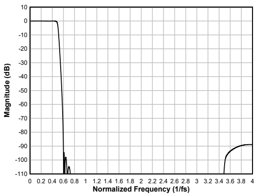
図 6-45. Low-latency Interpolation Filter Magnitude Response
