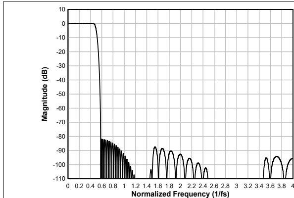
図 6-29. Linear-phase Interpolation Filter Magnitude Response
