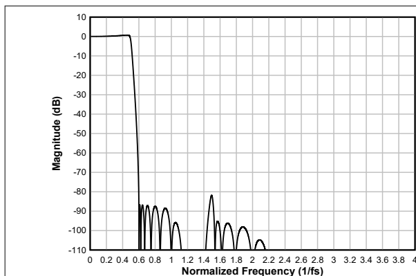
図 6-91. Ultra Low-latency Decimation Filter Magnitude Response
