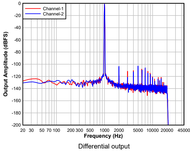
5-15. DAC FFT with -1dBFS Input
