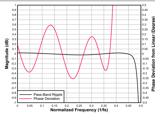
図 6-86. Low-latency Decimation Filter Pass-Band Ripple and Phase Deviation
