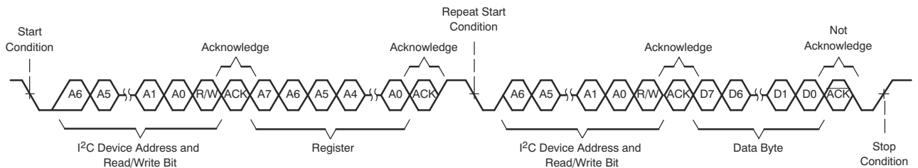
Figure 6-105. I 2 C Single-Byte Read Transfer
