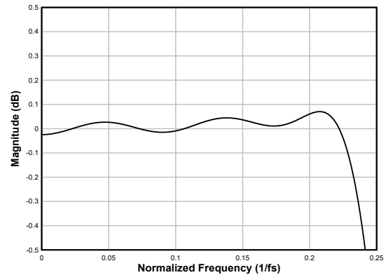
図 6-78. Linear-phase Decimation Filter Pass-Band Ripple
