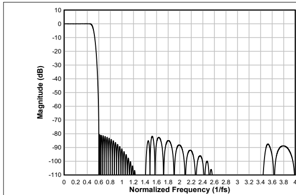
図 6-69. Linear-phase Decimation Filter Magnitude Response
