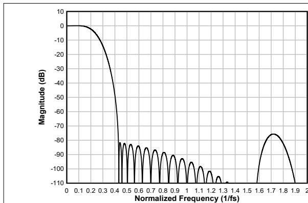
図 6-79. Linear-phase Decimation Filter Magnitude Response
