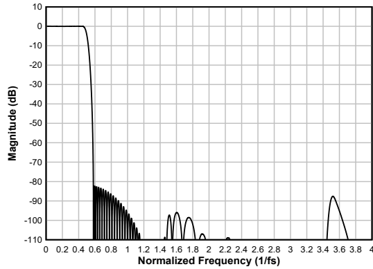
図 6-71. Linear-phase Decimation Filter Magnitude Response
