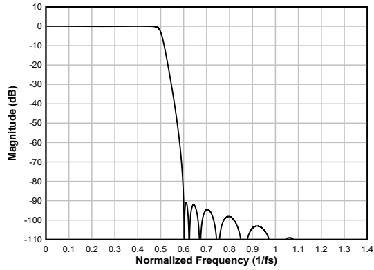
6-99. Ultra Low-latency Decimation Filter Magnitude Response
