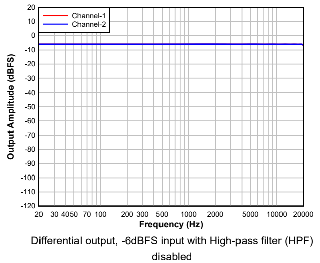
5-18. DAC Frequency Response
