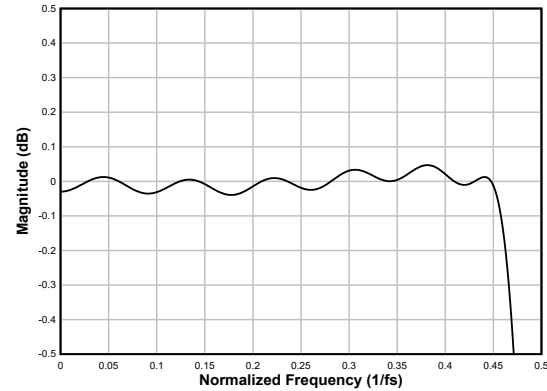
図 6-70. Linear-phase Decimation Filter Pass-Band Ripple
