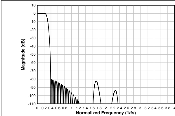
図 6-75. Linear-phase Decimation Filter Magnitude Response
