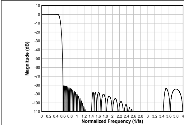
図 6-25. Linear-phase Interpolation Filter Magnitude Response
