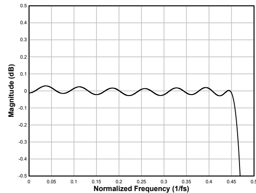
図 6-30. Linear-phase Interpolation Filter Pass-Band Ripple
