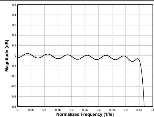
図 6-32. Linear-phase Interpolation Filter Pass-Band Ripple
