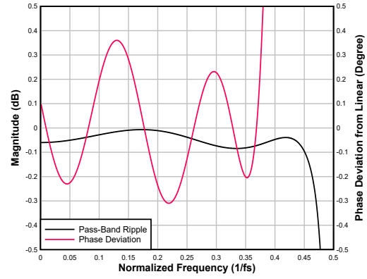
図 6-44. Low-latency Interpolation Filter Pass-Band Ripple and Phase Deviation
