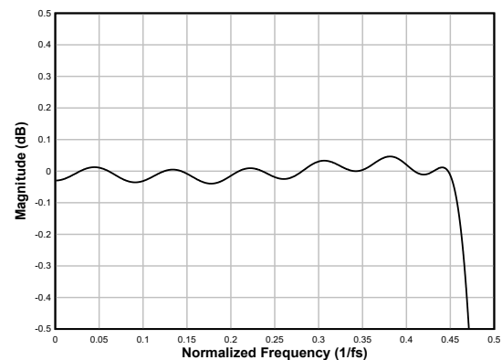
図 6-68. Linear-phase Decimation Filter Pass-Band Ripple
