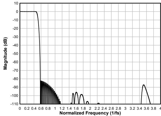
図 6-73. Linear-phase Decimation Filter Magnitude Response
