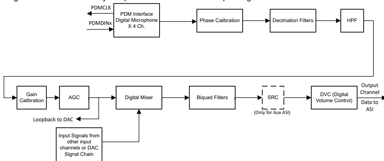
图 6-61. PDM Recording Signal-Chain Processing Flowchart
