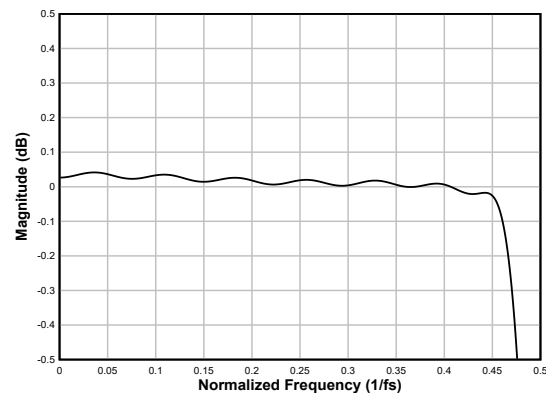
図 6-64. Linear-phase Decimation Filter Pass-Band Ripple
