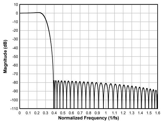
図 6-37. Linear-phase Interpolation Filter Magnitude Response
