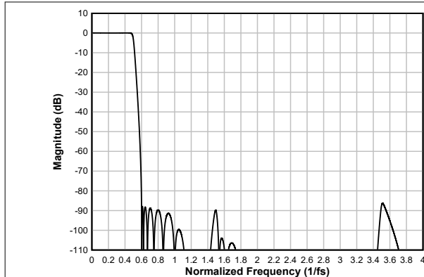
図 6-85. Low-latency Decimation Filter Magnitude Response
