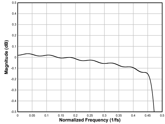
図 6-26. Linear-phase Interpolation Filter Pass-Band Ripple
