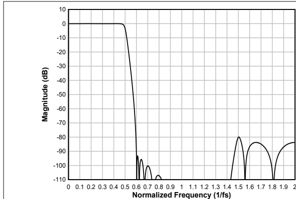
図 6-47. Low-latency Interpolation Filter Magnitude Response
