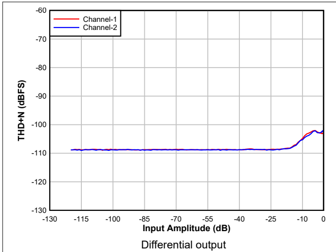
5-5. DAC THD+N Level vs Input
