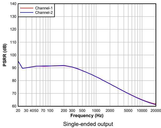
5-17. DAC PSRR vs Frequency
