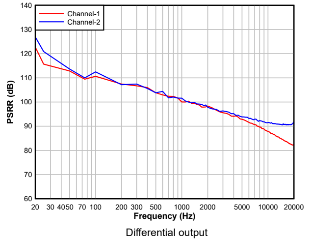
5-16. DAC PSRR vs Frequency
