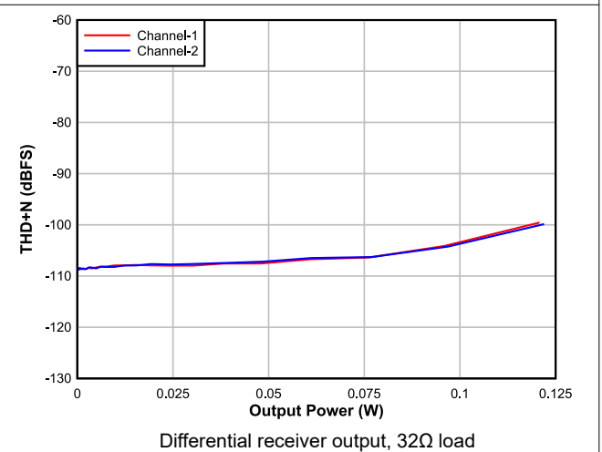
5-8. DAC THD+N Level vs Output Power
