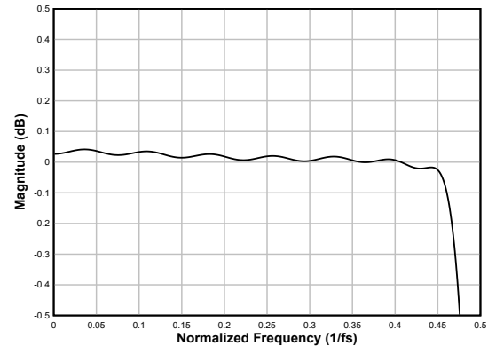
図 6-66. Linear-phase Decimation Filter Pass-Band Ripple
