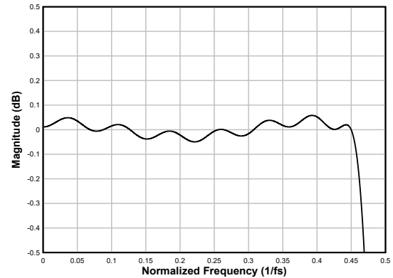
図 6-74. Linear-phase Decimation Filter Pass-Band Ripple
