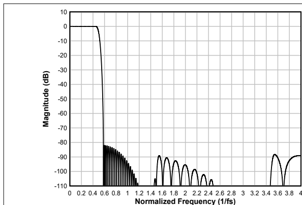
図 6-31. Linear-phase Interpolation Filter Magnitude Response
