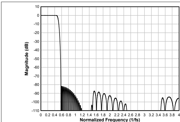
図 6-27. Linear-phase Interpolation Filter Magnitude Response
