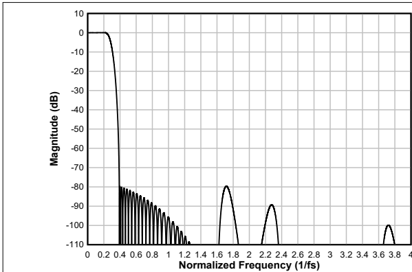
図 6-77. Linear-phase Decimation Filter Magnitude Response
