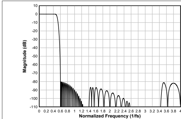
図 6-65. Linear-phase Decimation Filter Magnitude Response
