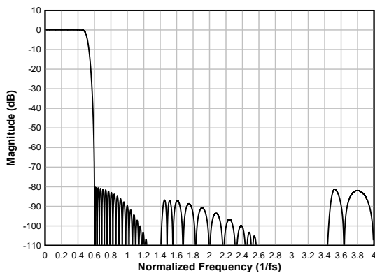
図 6-63. Linear-phase Decimation Filter Magnitude Response
