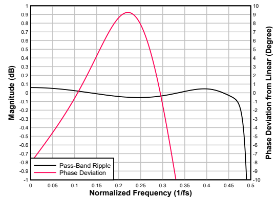
図 6-90. Low-latency Decimation Filter Pass-Band Ripple and Phase Deviation
