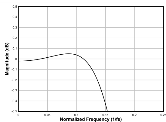
図 6-80. Linear-phase Decimation Filter Pass-Band Ripple
