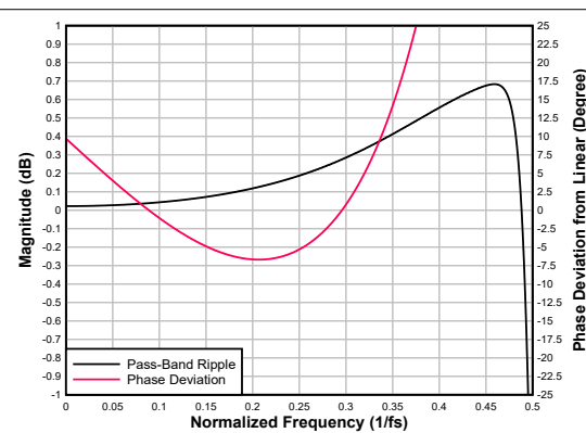
図 6-92. Ultra Low-latency Decimation Filter Pass-Band Ripple and Phase Deviation
