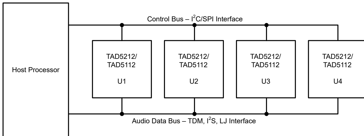
图 6-14. Multiple TAD5112 Devices With Shared Control and Audio Data Buses
