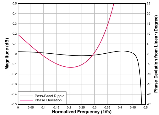
図 6-98. Ultra Low-latency Decimation Filter Pass-Band Ripple and Phase Deviation
