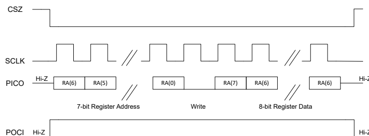
図 6-107. SPI Single-Byte Write Transfer
