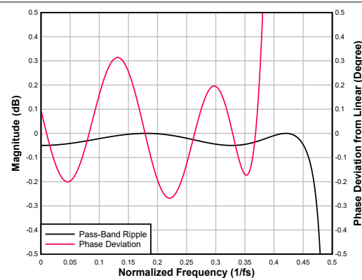
図 6-48. Low-latency Interpolation Filter Pass-Band Ripple and Phase Deviation
