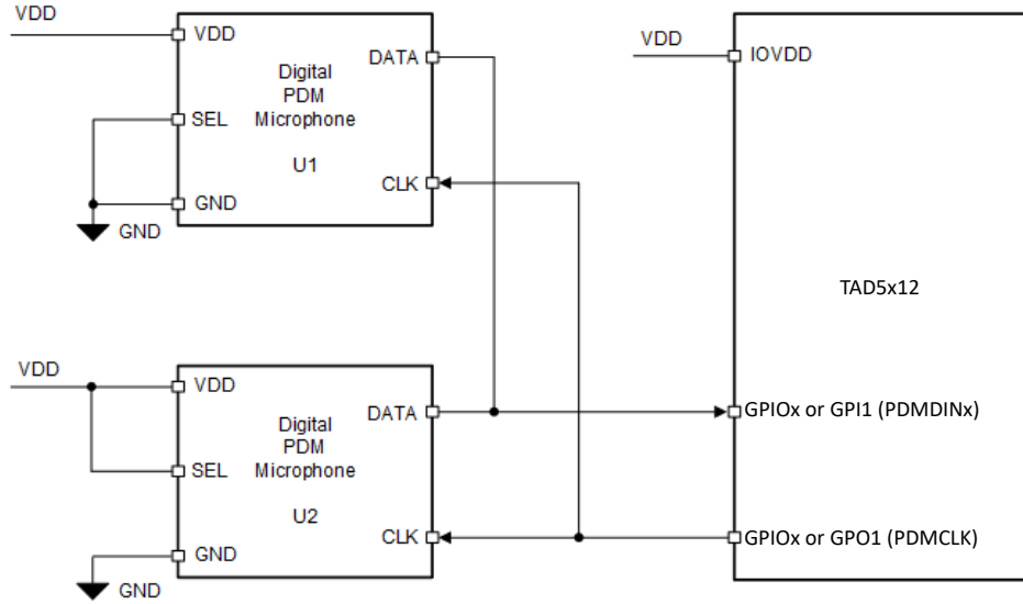
図 6-19. Digital PDM Microphones Connection Diagram for the TAD5112
