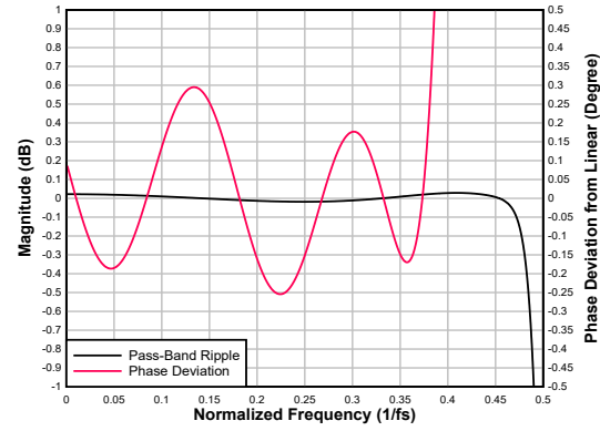
図 6-88. Low-latency Decimation Filter Pass-Band Ripple and Phase Deviation
