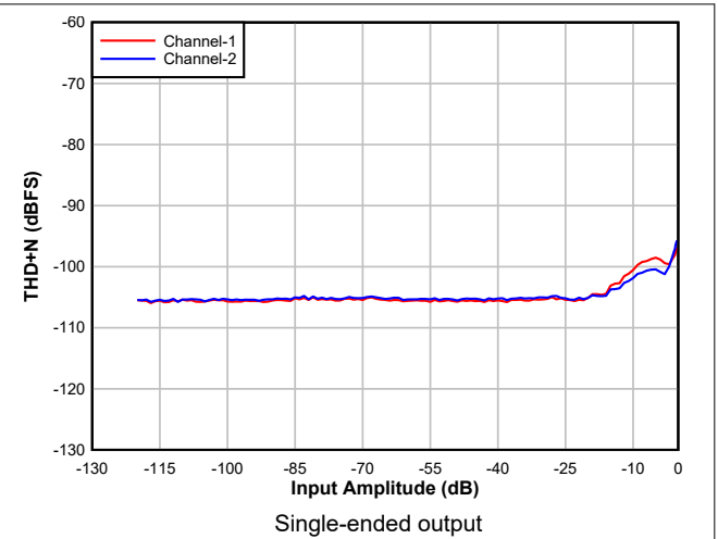
5-6. DAC THD+N Level vs Input
