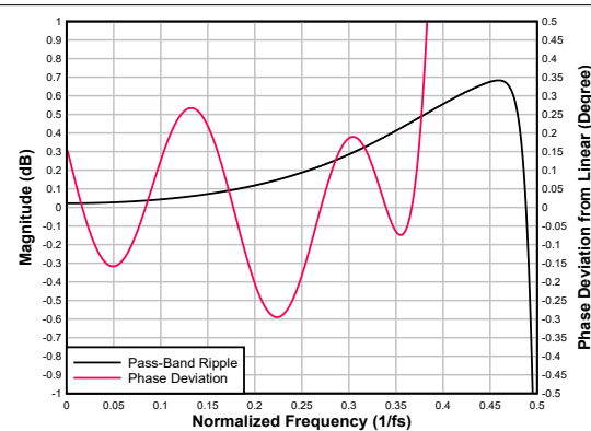
Figure 6-42. Low-latency Decimation Filter Pass-Band Ripple and Phase Deviation
