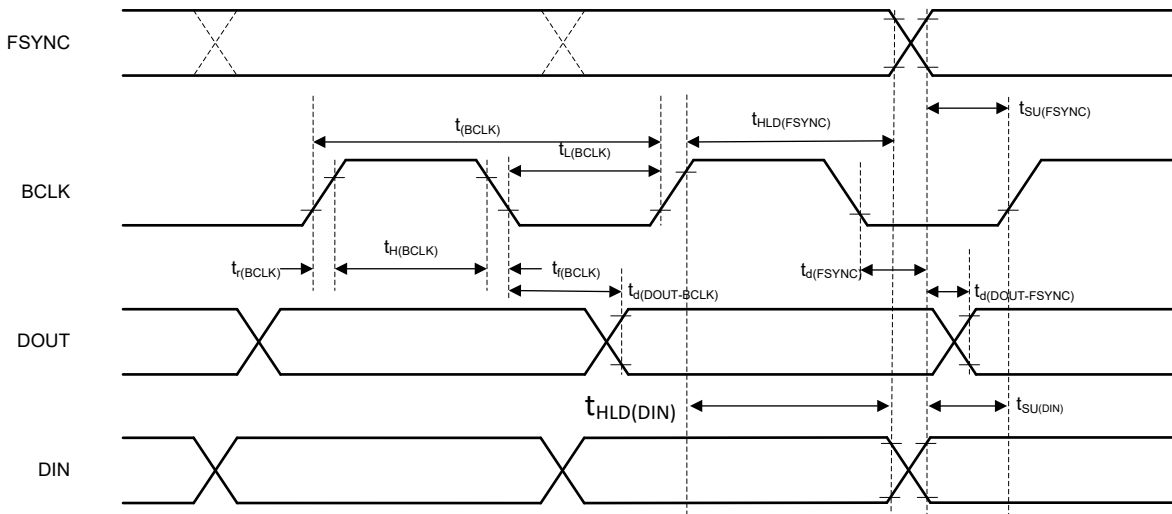
図 5-3. TDM, I 2 S, LJ Interface Timing Diagram
