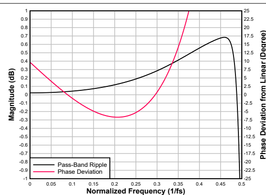
图 6-54. Ultra Low-latency Decimation Filter Pass-Band Ripple and Phase Deviation
