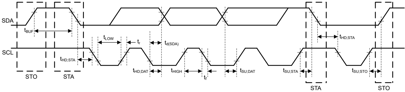
図 5-1. I 2 C Interface Timing Diagram
