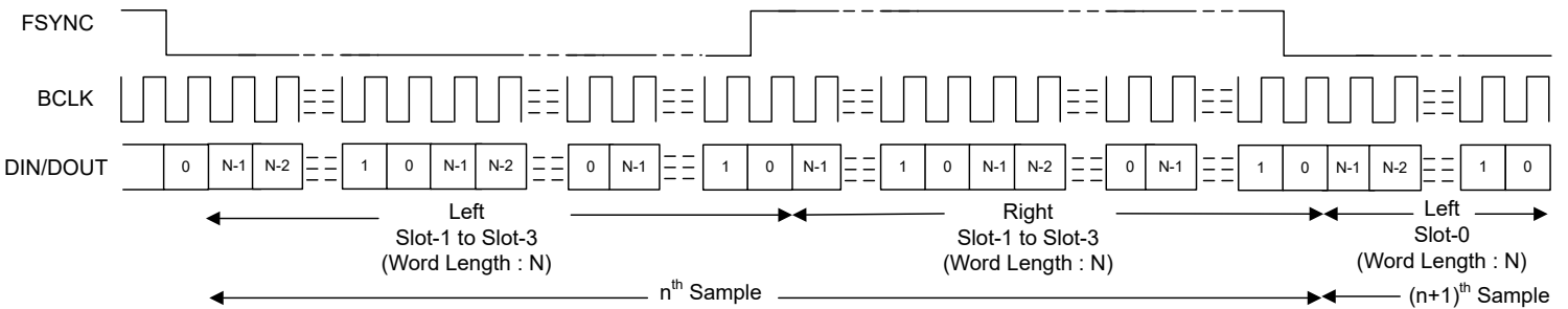
6-7. I 2 S Protocol Timing (No Idle BCLK Cycles, PASI_TX_OFFSET = 0)
