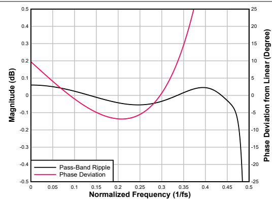
図 6-60. Ultra Low-latency Decimation Filter Pass-Band Ripple and Phase Deviation
