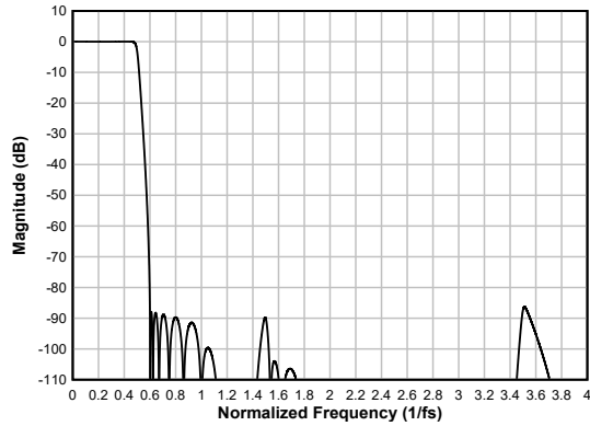
6-55. Ultra Low-latency Decimation Filter Magnitude Response
