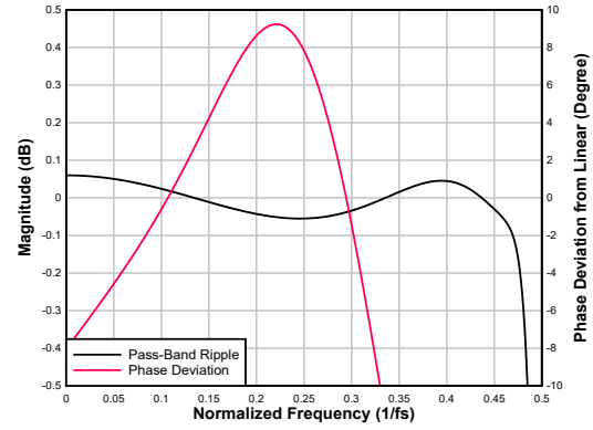
图 6-50. Low-latency Decimation Filter Pass-Band Ripple and Phase Deviation
