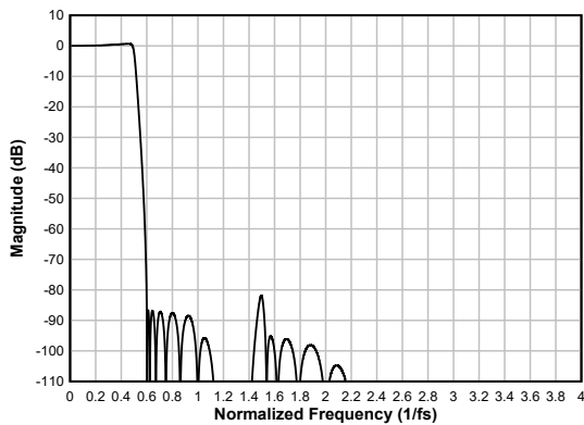
图 6-51. Ultra Low-latency Decimation Filter Magnitude Response
