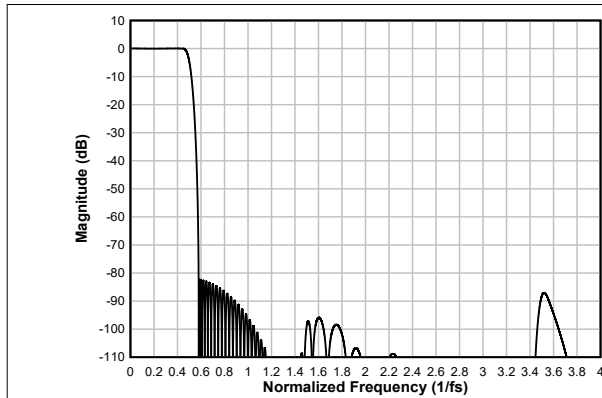
図 6-33. Linear-phase Decimation Filter Magnitude Response
