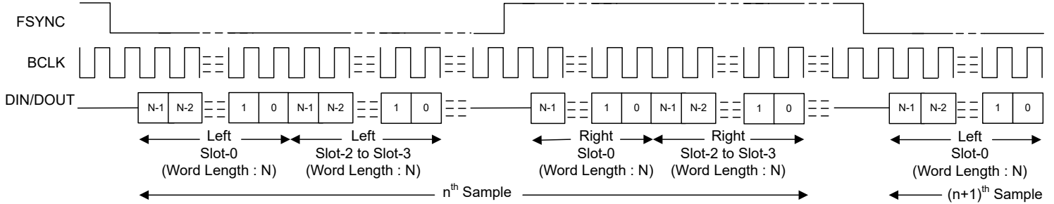
6-5. I 2 S Mode Standard Protocol Timing (PASI_TX_OFFSET = 0)
