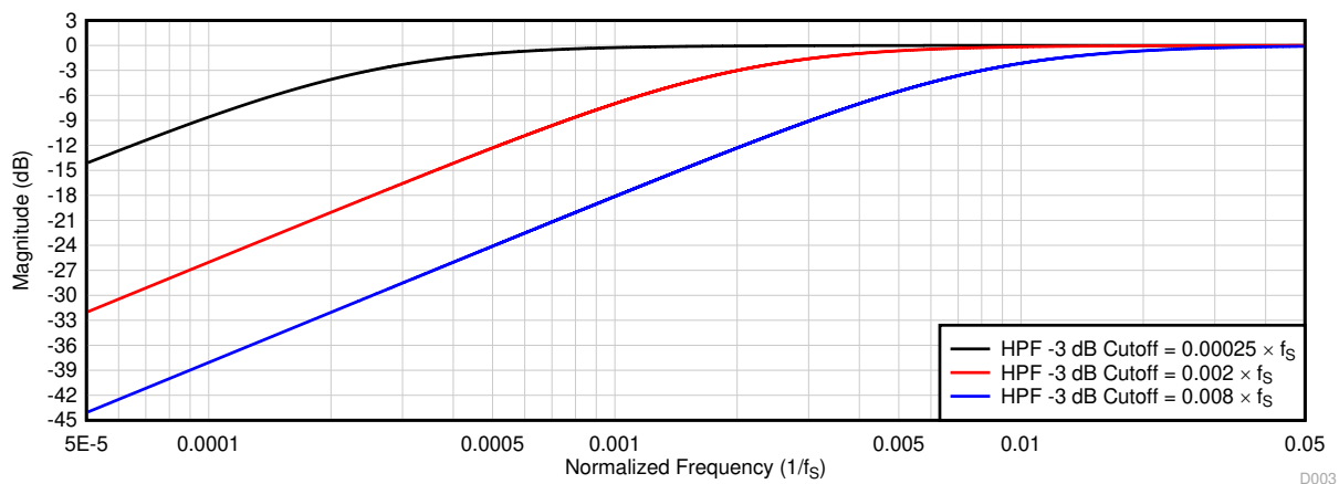
図 6-21. HPF Filter Frequency Response Plot
