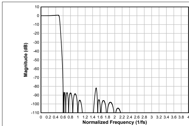
Figure 6-51. Ultra Low-latency Decimation Filter Magnitude Response
