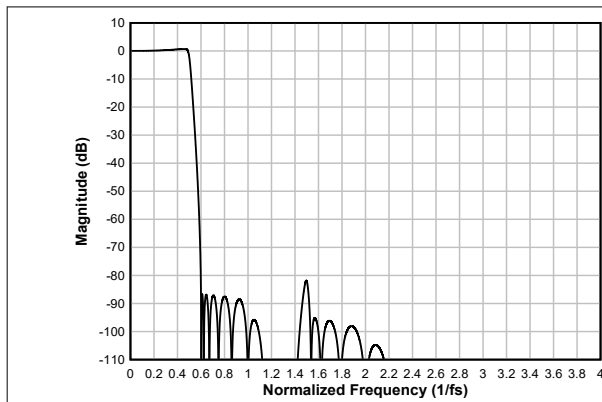
图 6-53. Ultra Low-latency Decimation Filter Magnitude Response
