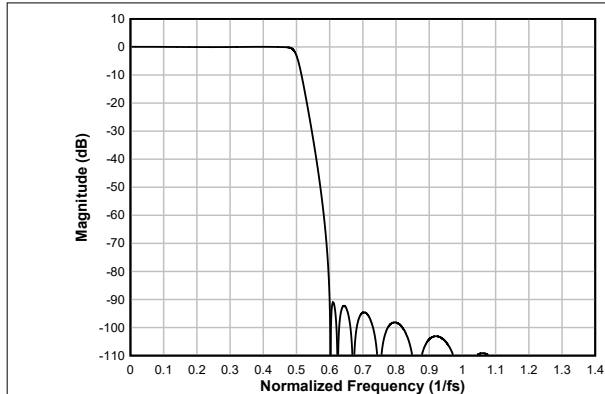
図 6-59. Ultra Low-latency Decimation Filter Magnitude Response
