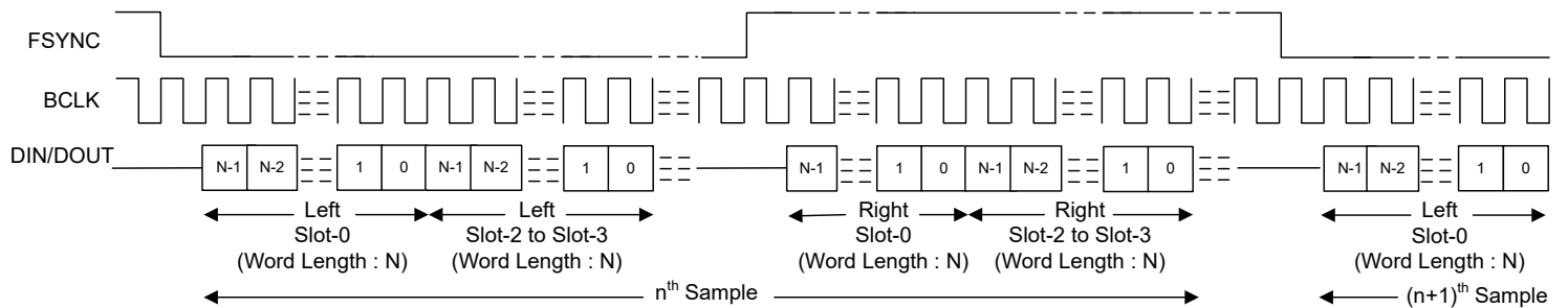
6-8. I 2 S Protocol Timing (PASI_TX_OFFSET = 0 and PASI_BCLK_POL = 1)
