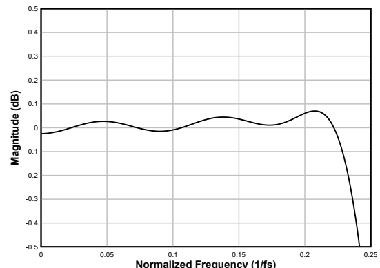
図 6-38. Linear-phase Decimation Filter Pass-Band Ripple
