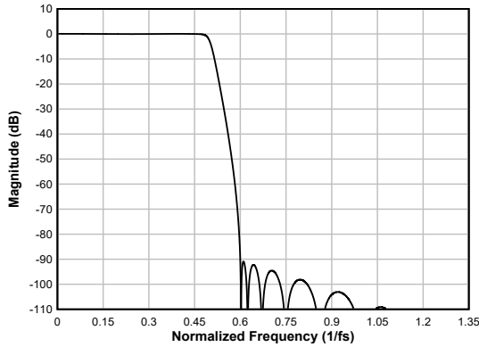
图 6-49. Low-latency Decimation Filter Magnitude Response
