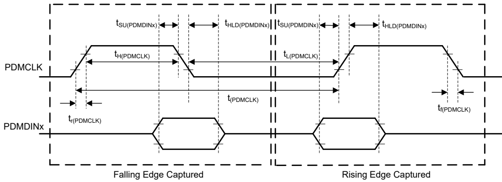
图 5-4. PDM Digital Microphone Interface Timing Diagram
