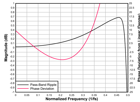
图 6-52. Ultra Low-latency Decimation Filter Pass-Band Ripple and Phase Deviation
