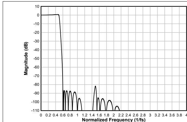
Figure 6-41. Low-latency Decimation Filter Magnitude Response
