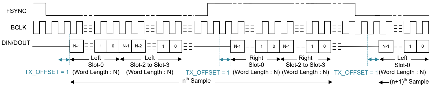
6-6. I 2 S Protocol Timing (PASI_TX_OFFSET = 1)
