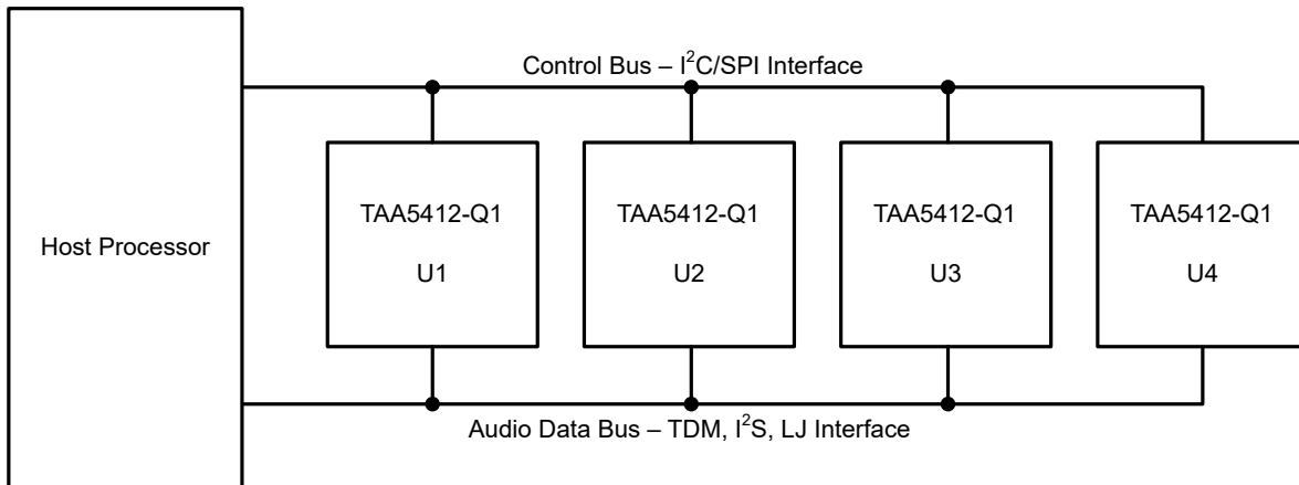
图 6-13. Multiple TAA5412-Q1 Devices With Shared Control and Audio Data Buses
