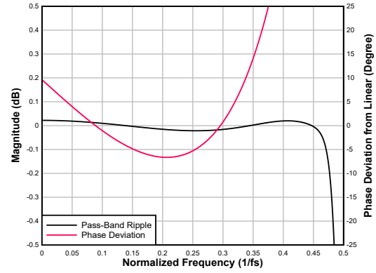
6-56. Ultra Low-latency Decimation Filter Pass-Band Ripple and Phase Deviation
