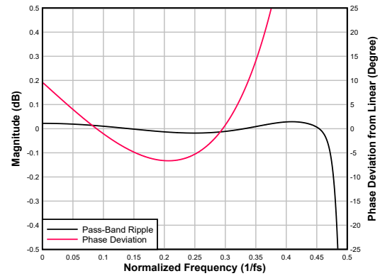
6-58. Ultra Low-latency Decimation Filter Pass-Band Ripple and Phase Deviation
