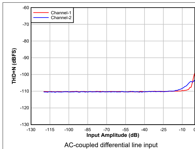
图 5-5. ADC THD+N Level vs Input
