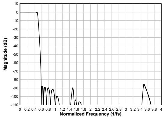
6-57. Ultra Low-latency Decimation Filter Magnitude Response
