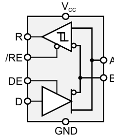
图 8-1. Logic Diagram (Positive)
