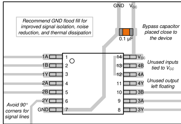
8-3. Example Layout for the SN74LVC7032A-Q1
