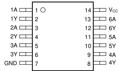
図 5-2. SN74LV6T07 PW Package, 14-Pin TSSOP (Top View)
