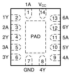
図 5-1. SN74LV6T07 BQA Package, 14-Pin WQFN (Top View)
