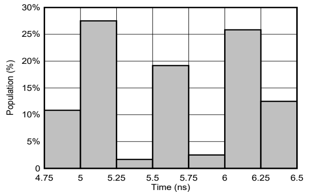
6-18. T PD Distribution; 5-V; T A = -55°C to 125°C (40 Samples)
