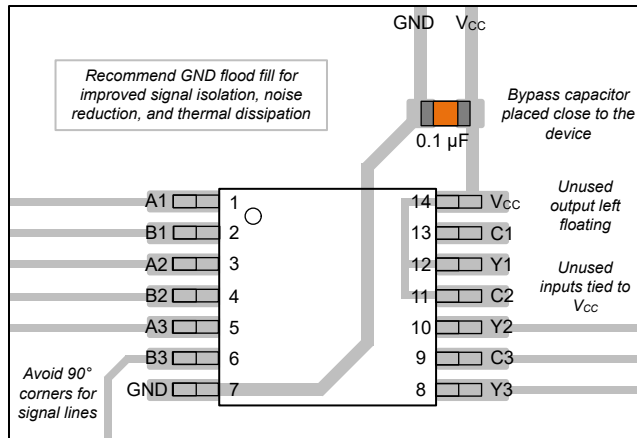
图 8-3. Example Layout for the SN54SC3T97-SEP
