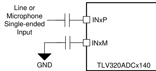
図 7-15. Single-Ended AC-Coupled Input Connection
