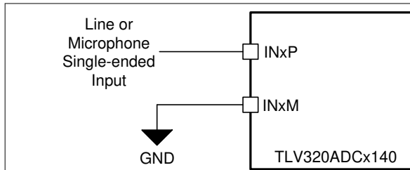
図 7-14. Single-Ended DC-Coupled Input Connection
