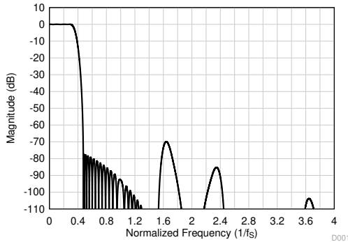
8-33. Linear Phase Decimation Filter Magnitude Response
