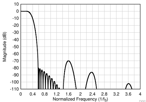
8-35. Linear Phase Decimation Filter Magnitude Response
