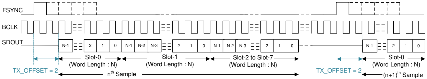
FIG 8-2. TDM Mode Protocol Timing (TX_OFFSET = 2)
