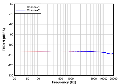
Plot9_MIC_THDN_VS_FREQ.grf
