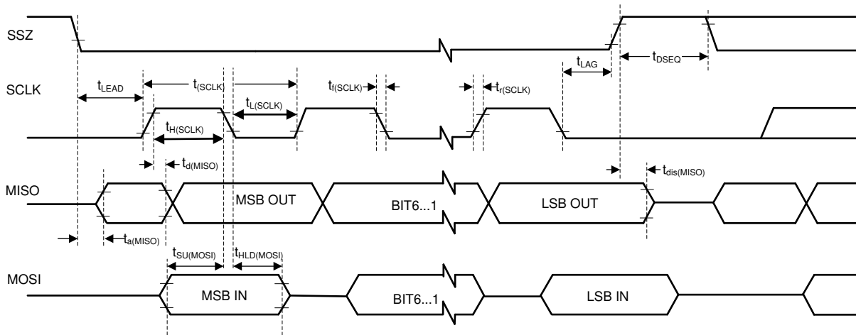
☒ 7-2. SPI Interface Timing Diagram
