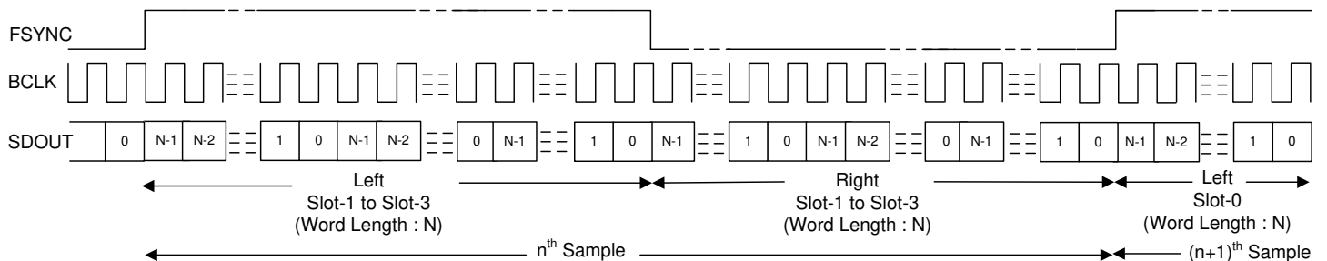
Fig 8-11. LJ Protocol Timing (No Idle BCLK Cycles, TX_OFFSET = 0)
