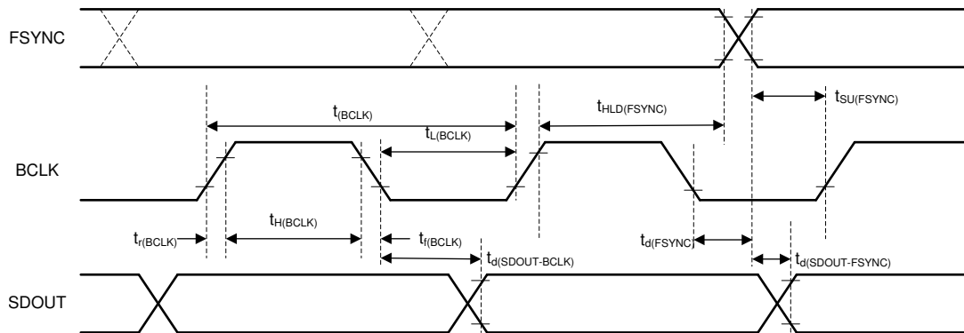
☒ 7-3. TDM, I 2 S, LJ Interface Timing Diagram
