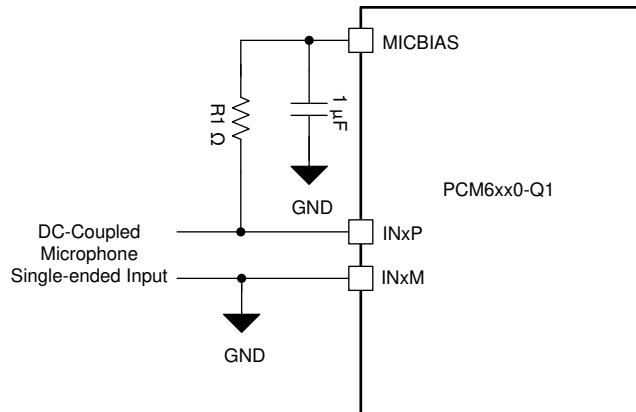
8-15. DC-Coupled Microphone Single-Ended Input Connection
