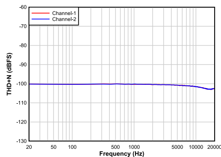
Plot10_MIC_SE_THDN_VS_FREQ.grf
