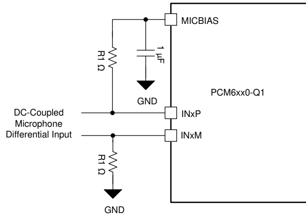
8-14. DC-Coupled Microphone Differential Input Connection
