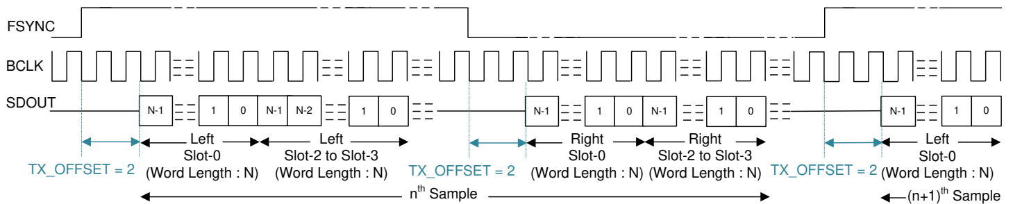
Fig 8-10. LJ Protocol Timing (TX_OFFSET = 2)
