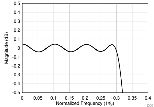
8-34. Linear Phase Decimation Filter Pass-Band Ripple
