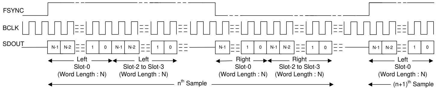
Fig 8-9. LJ Mode Standard Protocol Timing (TX_OFFSET = 0)
