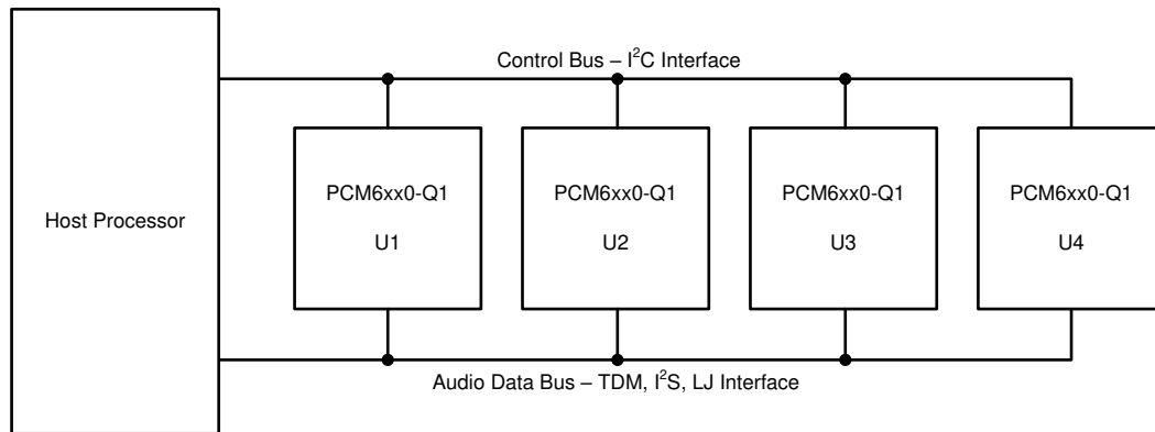
8-13. Multiple PCM6020-Q1 Devices With Shared Control and Audio Data Buses
