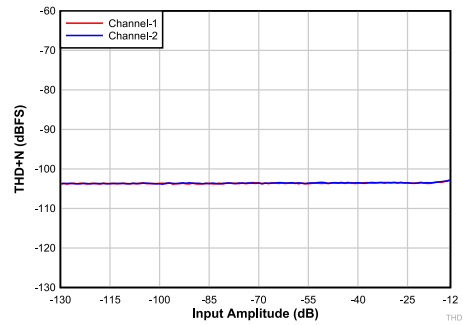
Plot8_MIC_SE_THDN_VS_AMPL.grf
