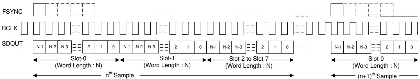
FIG 8-4. TDM Mode Protocol Timing (TX_OFFSET = 0 and BCLK_POL = 1)
