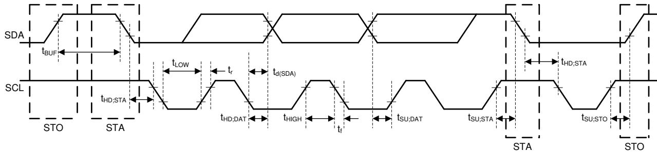
☒ 7-1. I 2 C Interface Timing Diagram
