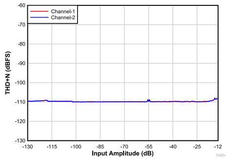
Plot7_MIC_THDN_VS_AMPL.grf
