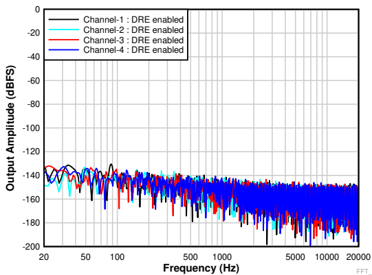
6-17. FFT With Idle Input With DRE Enabled
