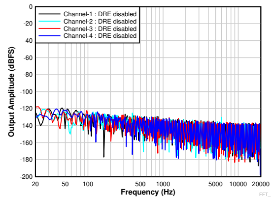
6-18. FFT With Idle Input With DRE Disabled
