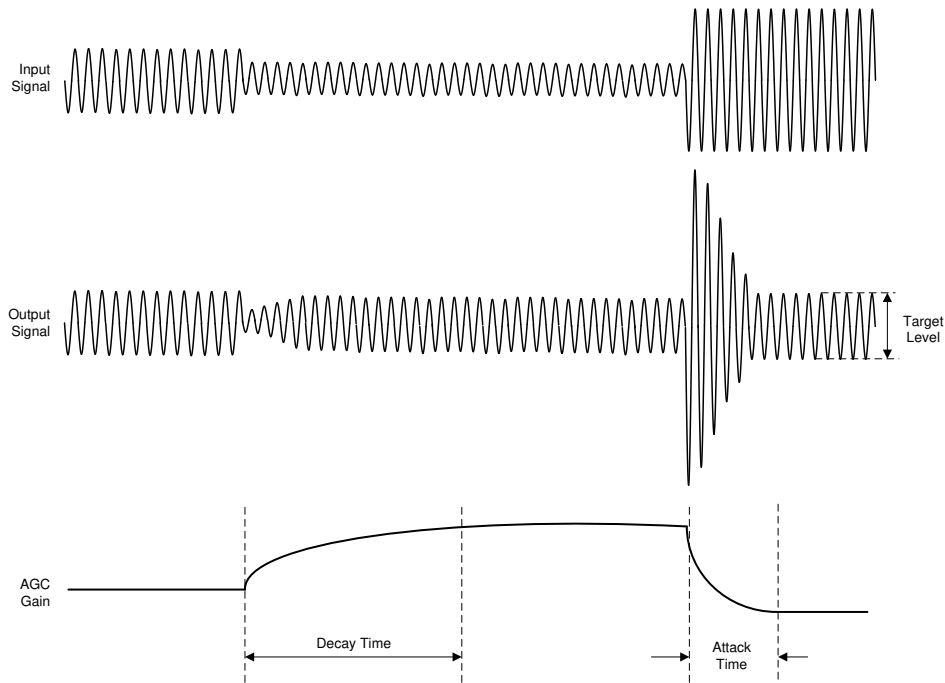
図 7-63. AGC Characteristics
