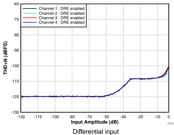
6-5. THD+N vs Input Amplitude With DRE Enabled
