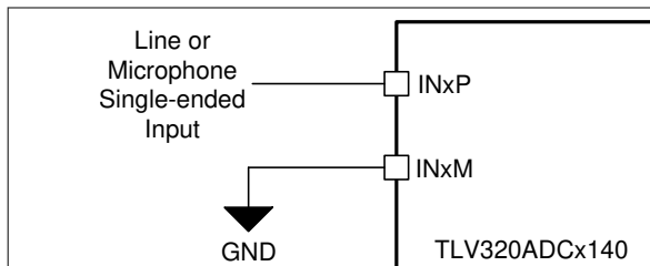
图 7-14. Single-Ended DC-Coupled Input Connection
