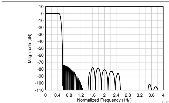
図 7-25. Linear Phase Decimation Filter Magnitude Response
