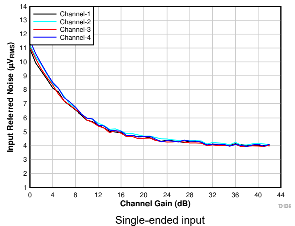
6-14. Input-Referred Noise vs Channel Gain
