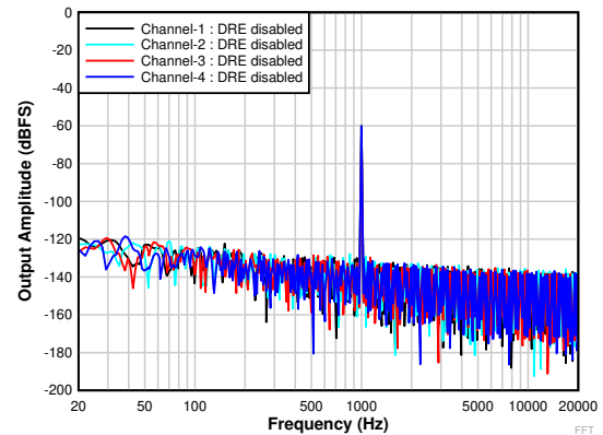
6-20. FFT With a -60-dBr Input With DRE Disabled
