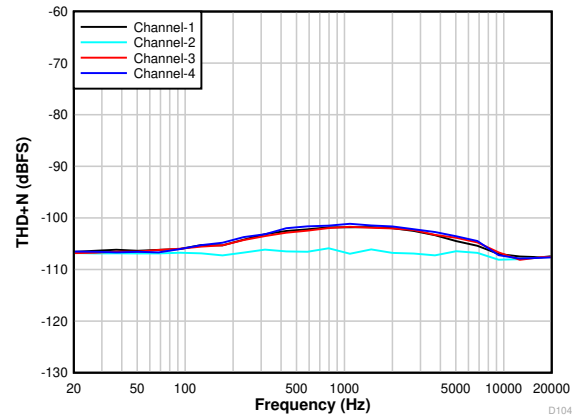
6-12. THD+N vs Input Frequency With a -1-dB Input
