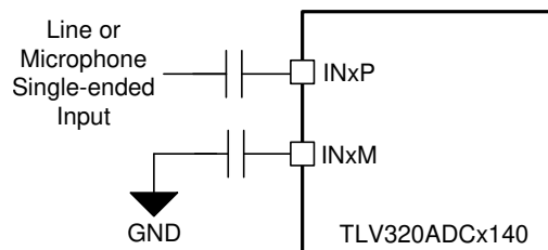
图 7-15. Single-Ended AC-Coupled Input Connection
