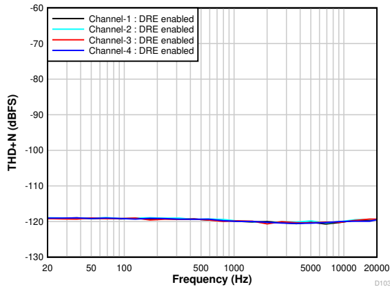
6-11. THD+N vs Input Frequency With a -60-dB Input
