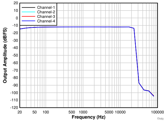
6-15. Frequency Response With a -12-dBr Input
