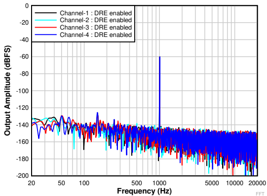
6-19. FFT With a -60-dBr Input With DRE Enabled
