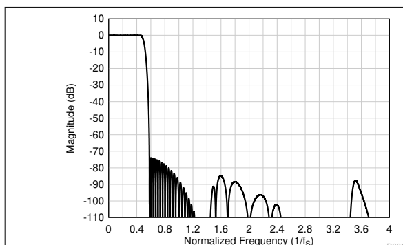
図 7-27. Linear Phase Decimation Filter Magnitude Response
