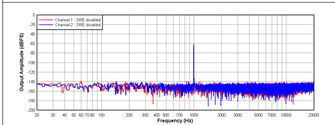
9-4. PCM1820-Q1: FFT With a -60-dBr Input With DRE Disabled
