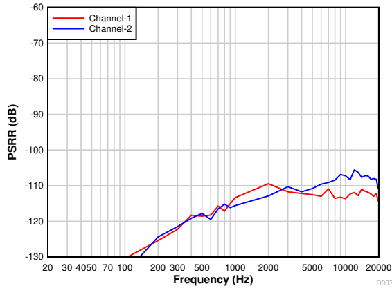
7-7. PCM1820-Q1: Power-Supply Rejection Ratio vs Ripple Frequency With a 100-mV PP Amplitude
