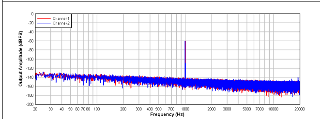
9-6. PCM1821-Q1: FFT With a -60-dBr Input
