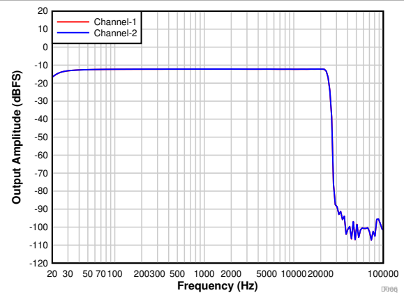
7-6. PCM1820-Q1: Frequency Response With a -12-dBr Input
