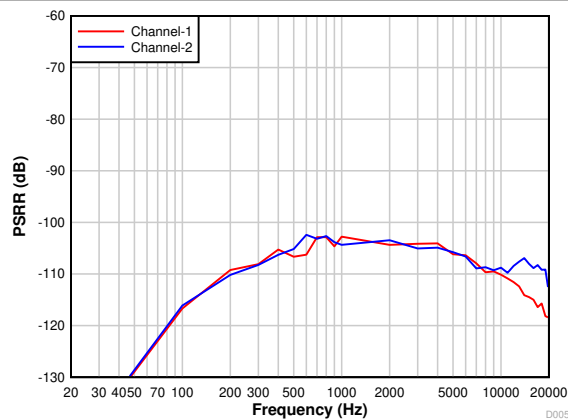
7-17. PCM1821-Q1: Power-Supply Rejection Ratio with Ripple Frequency With a 100\text{-mV}_{PP} Amplitude
