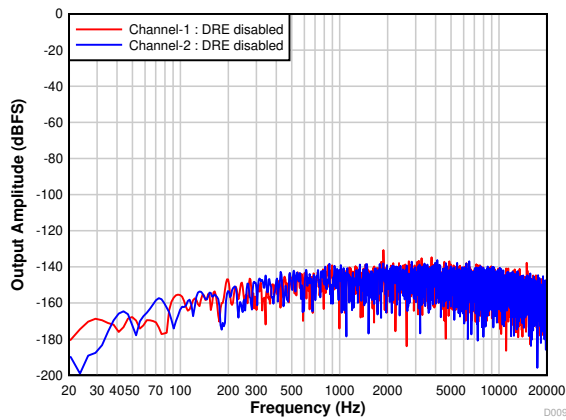
7-9. PCM1820-Q1: FFT With Idle Input and DRE Disabled
