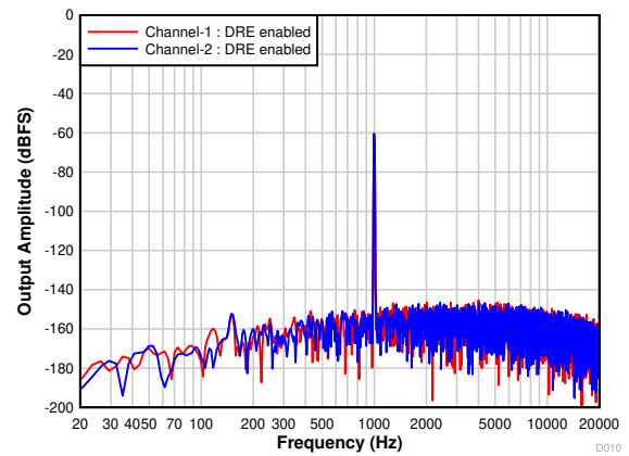
7-10. PCM1820-Q1: FFT With a -60-dBr Input and DRE Enabled
