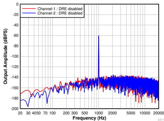
7-11. PCM1820-Q1: FFT With a -60-dBr Input and DRE Disabled
