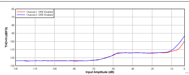
9-3. PCM1820-Q1: THD+N vs Input Amplitude With DRE Enabled
