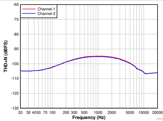
7-15. PCM1821-Q1: THD+N vs Input Frequency With a -1\text{-dB} Input
