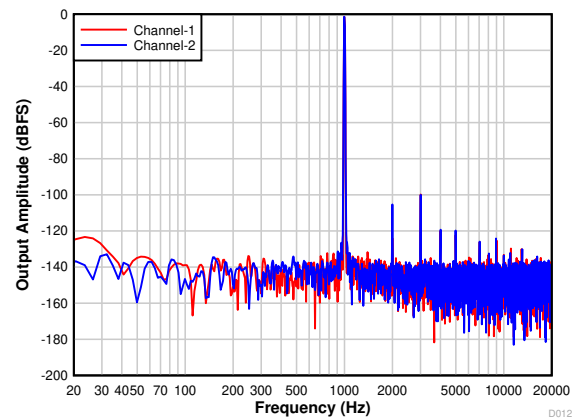
7-12. PCM1820-Q1: FFT With a -1-dBr Input
