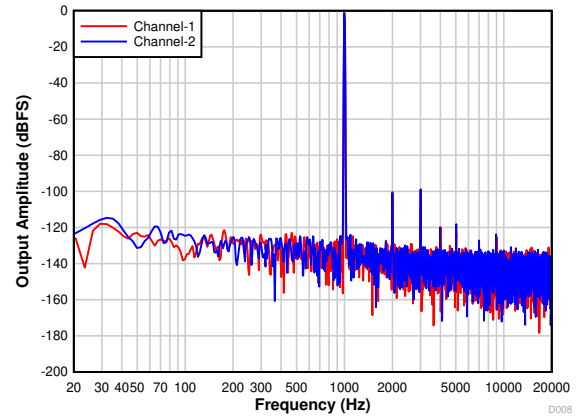
7-20. PCM1821-Q1: FFT With a -1\text{-dBr} Input
