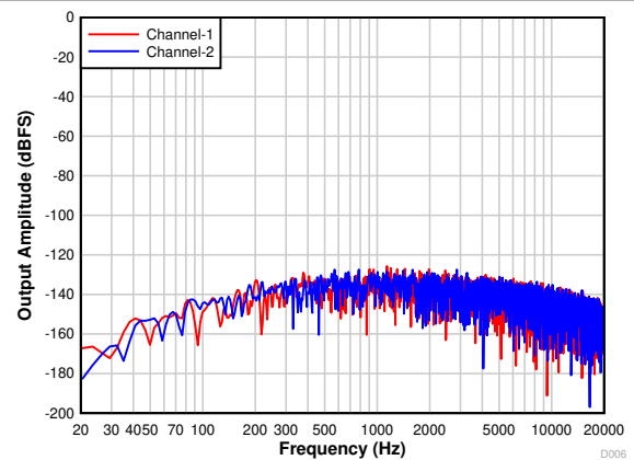
7-18. PCM1821-Q1: FFT With Idle Input and DRE Disabled
