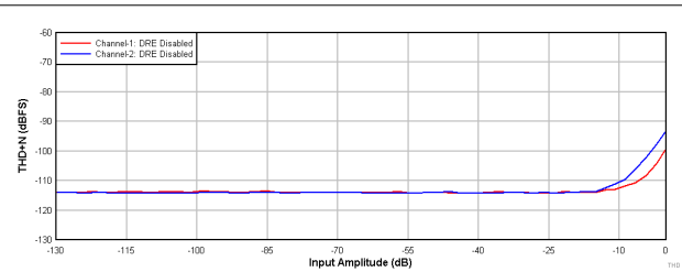
9-5. PCM1820-Q1: THD+N vs Input Amplitude With DRE Disabled
