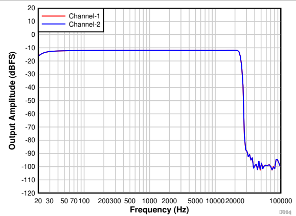
7-16. PCM1821-Q1: Frequency Response With a -12\text{-dB} Input
