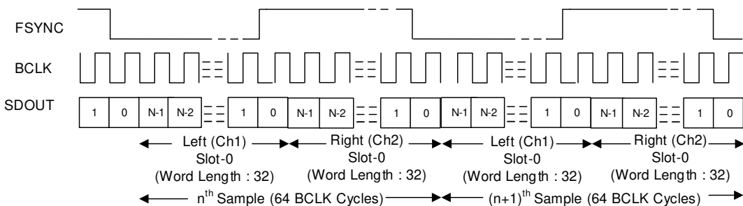
FIG 8-4. I 2 S Protocol Timing (FMT0 = LOW) In Master Mode
