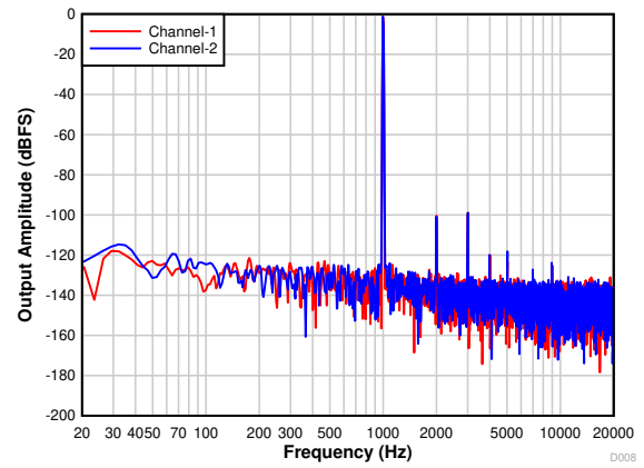
7-20. PCM1821: FFT With a -1-dBr Input
