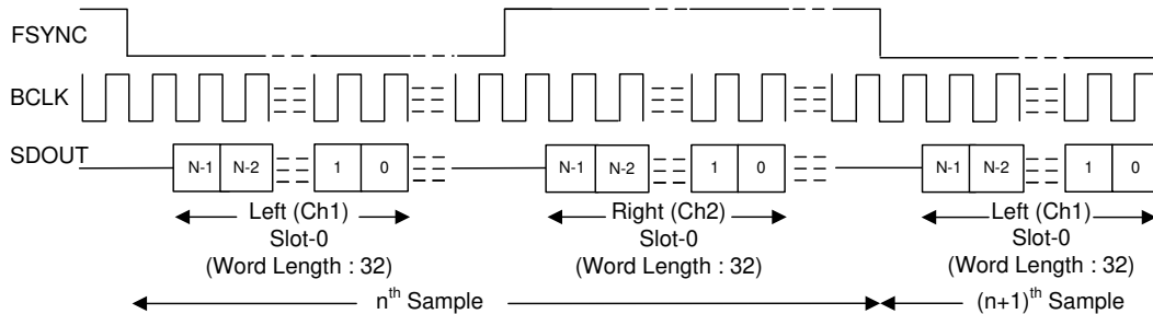
FIG 8-3. I 2 S Mode Protocol Timing (FMT0 = LOW) in Slave Mode
