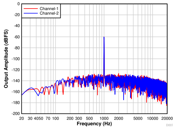
7-19. PCM1821: FFT With a -60-dBr Input
