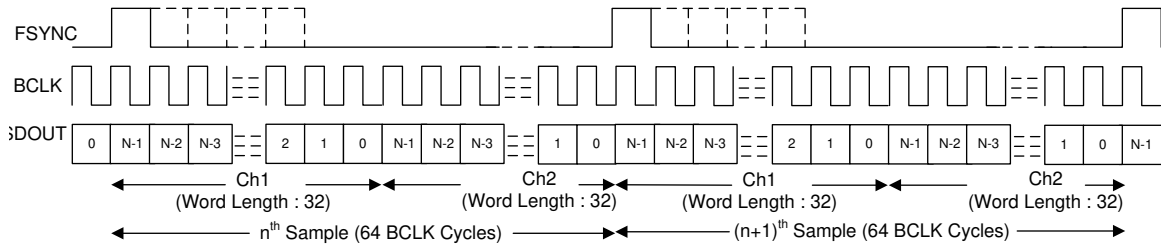
FIG 8-2. TDM Mode Protocol Timing (FMT0 = HIGH) In Master Mode
