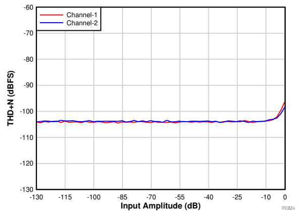
9-7. PCM1821: THD+N vs Input Amplitude
