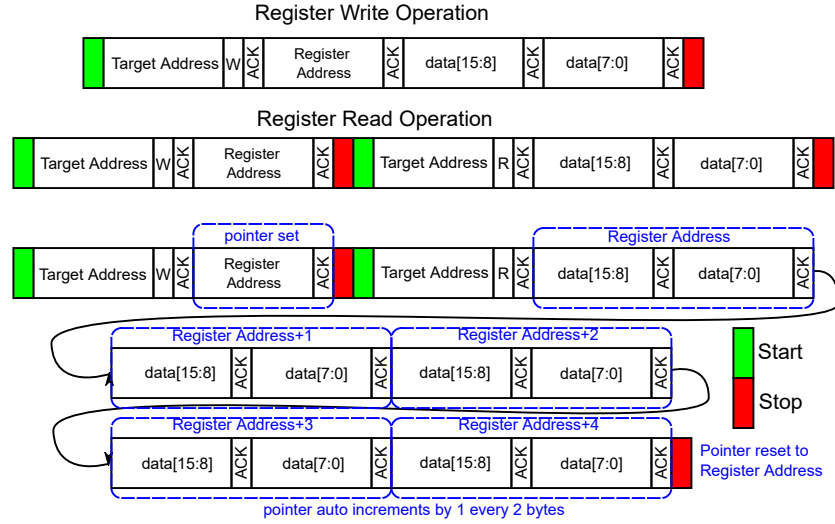
6-7. I 2 C Operations
