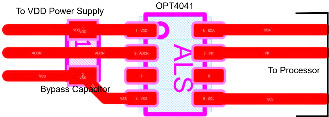
8-3. Layout Example for SOT-5X3 package
