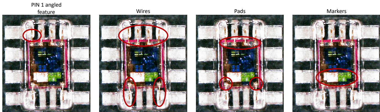
図 8-5. Identification Features for PIN 1 on Package
