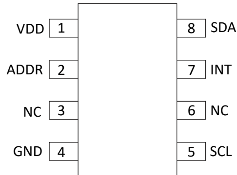
図 4-1. DTS Package, 8-Pin SOT 5X3, Top View
