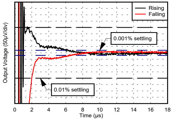
5-61. Large-Signal Step Response
