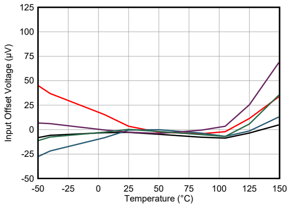
图 5-13. Offset Voltage Drift Distribution
