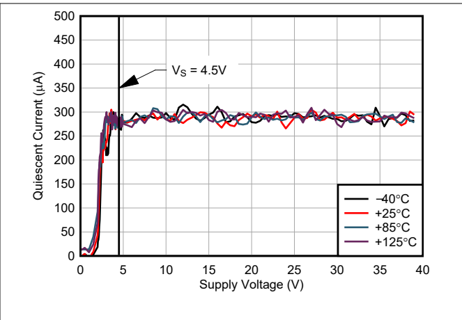
Figure 5-50. Quiescent Current vs Supply Voltage
