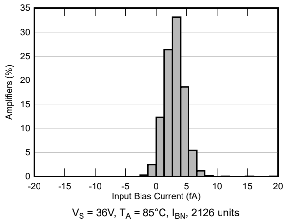
5-5. Input Bias Current Production Distribution
