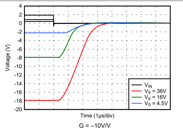
5-58. Negative Overload Recovery
