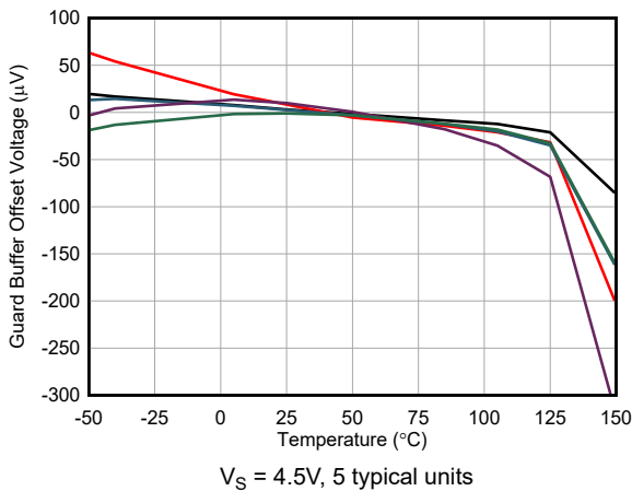
図 5-71. Guard Buffer Offset Voltage vs Temperature
