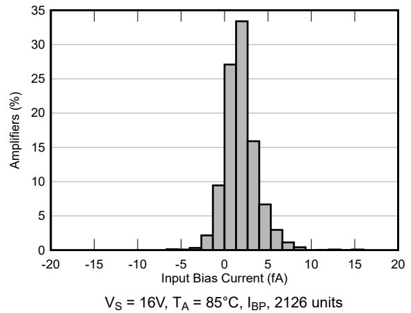
5-4. Input Bias Current Production Distribution
