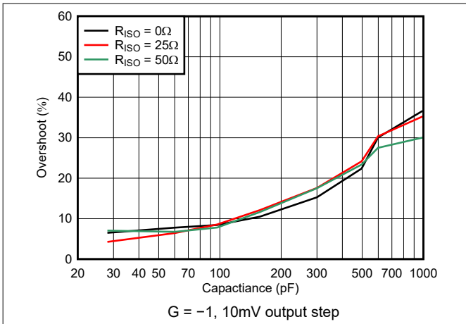
5-55. Small-Signal Overshoot vs Capacitive Load
