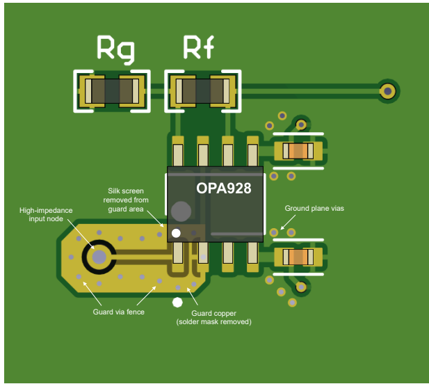
7-21. Layout Example: Noninverting Configuration
