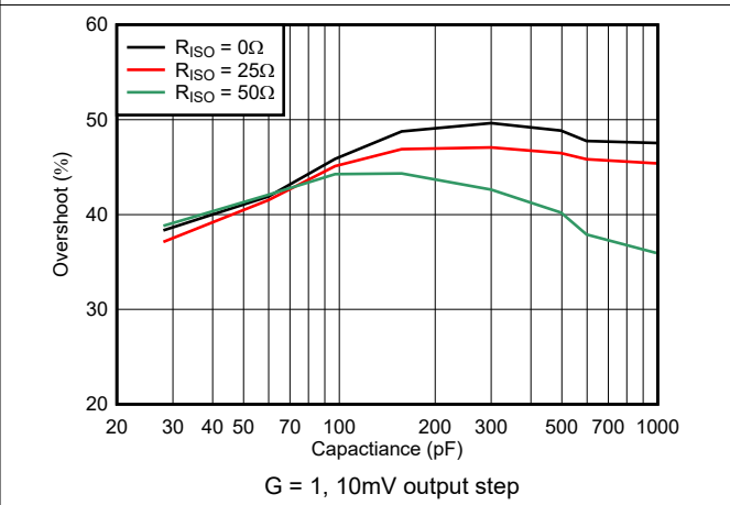
Figure 5-54. Small-Signal Overshoot vs Capacitive Load
