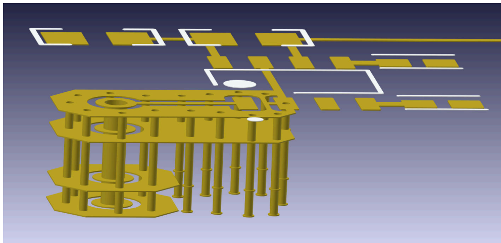
7-23. Layout Example: Three-Dimensional Guard (4-Layer PCB)
