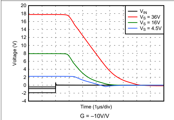
5-57. Positive Overload Recovery
