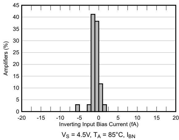
5-1. Input Bias Current Production Distribution
