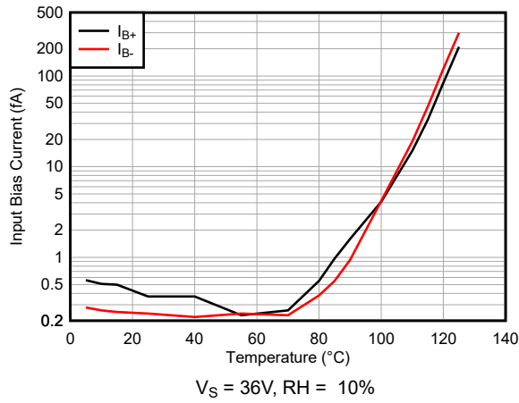
5-31. Input Bias Current vs Temperature
