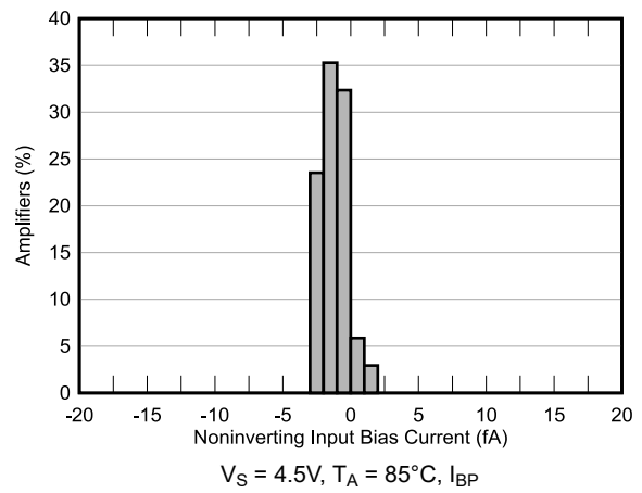
5-2. Input Bias Current Production Distribution
