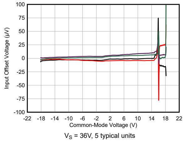
5-20. Offset Voltage vs Common-Mode Voltage in Transition Region
