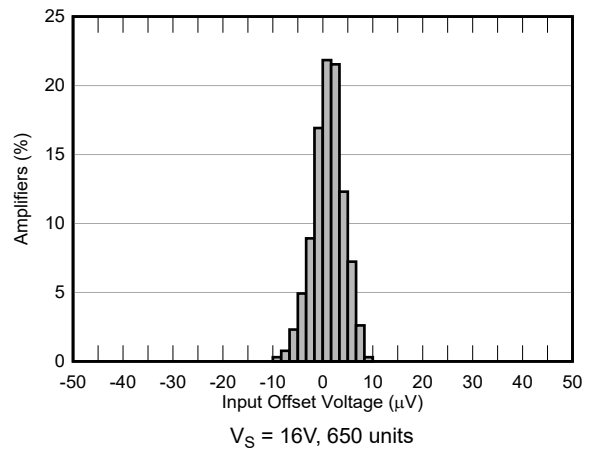
5-66. Guard Buffer Offset Distribution
