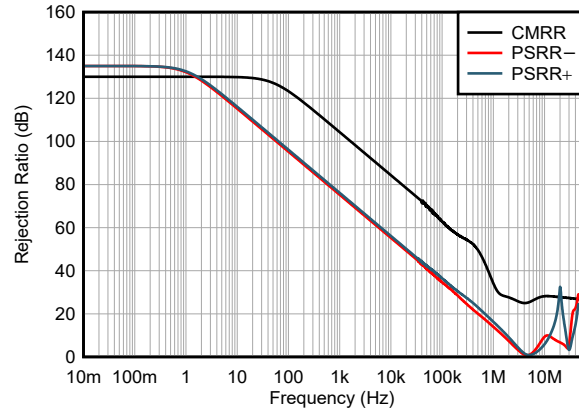
5-38. CMRR and PSRR vs Frequency
