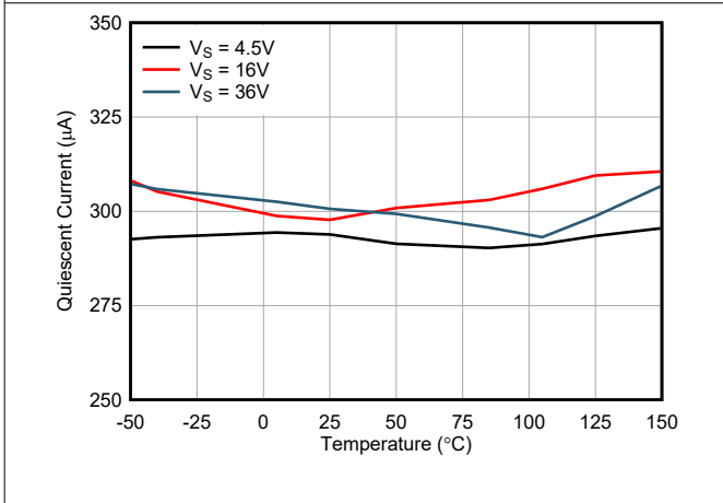
Figure 5-51. Quiescent Current vs Temperature
