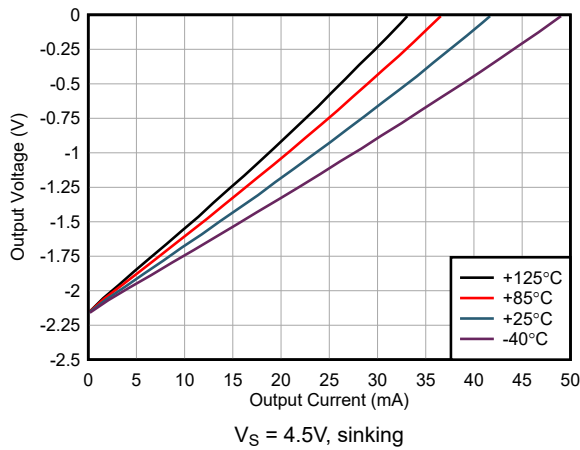
5-33. Output Voltage Swing vs Output Current
