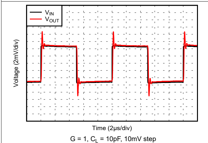
5-59. Small-Signal Step Response
