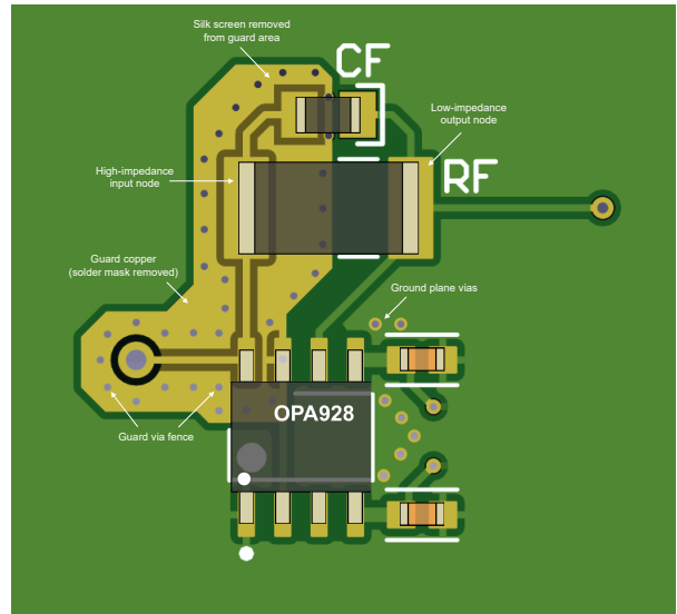
7-22. Layout Example: Inverting Configuration
