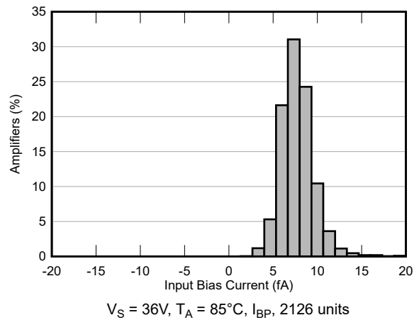
5-6. Input Bias Current Production Distribution
