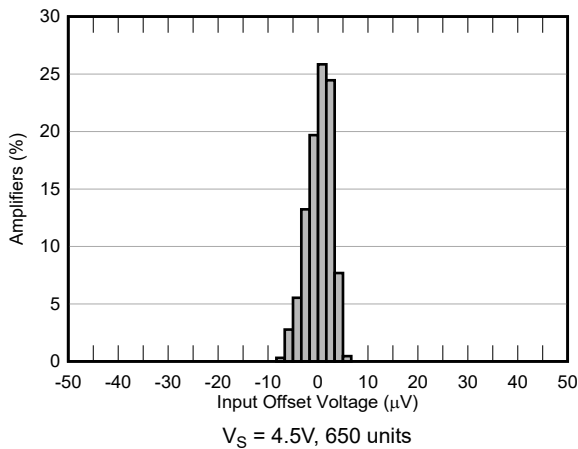
5-65. Guard Buffer Offset Distribution
