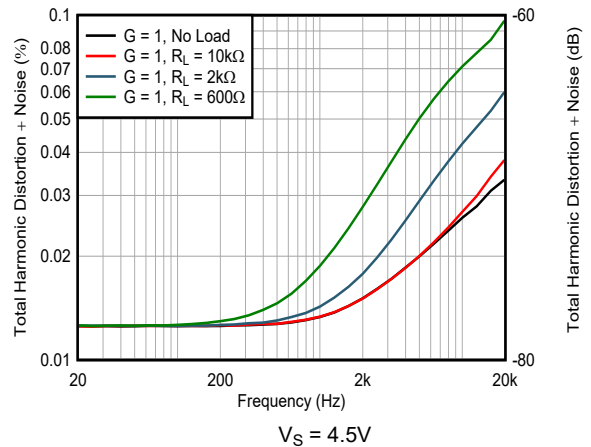
5-42. THD+N vs Frequency
