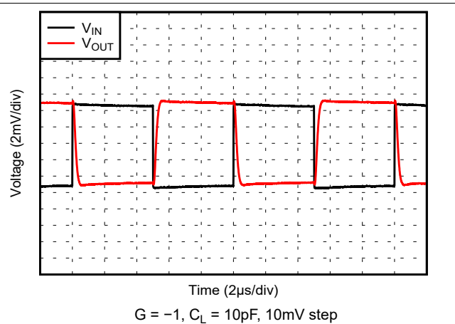
5-60. Small-Signal Step Response
