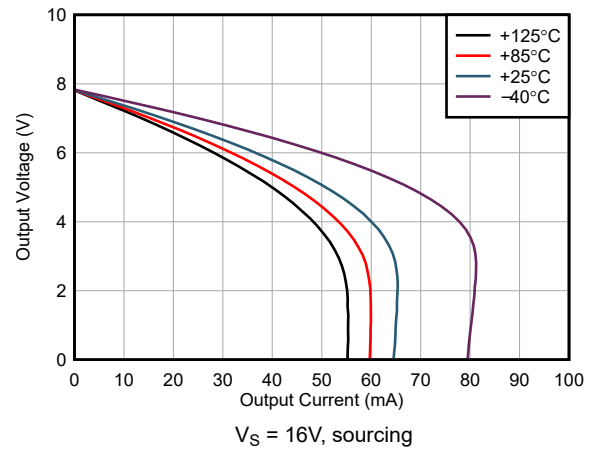
5-34. Output Voltage Swing vs Output Current
