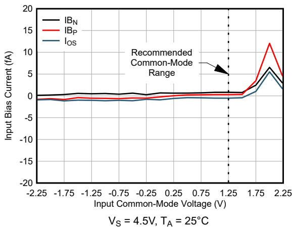
5-23. Input Bias Current vs Common-Mode Voltage
