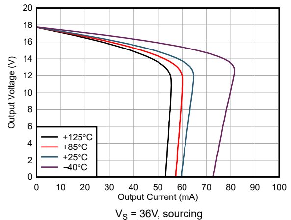
5-36. Output Voltage Swing vs Output Current
