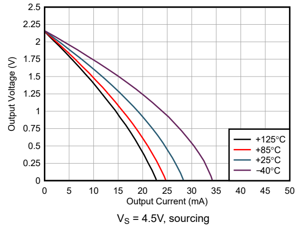
5-32. Output Voltage Swing vs Output Current
