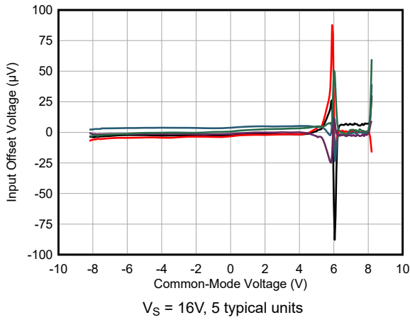
5-19. Offset Voltage vs Common-Mode Voltage in Transition Region
