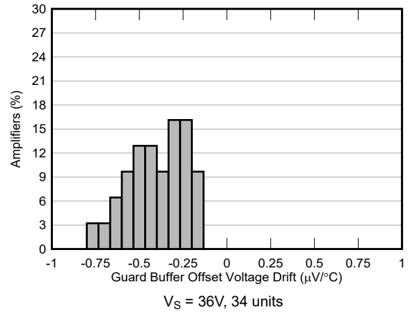
図 5-70. Guard Buffer Offset Drift Distribution
