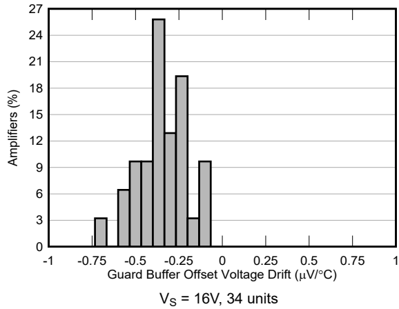
図 5-69. Guard Buffer Offset Drift Distribution
