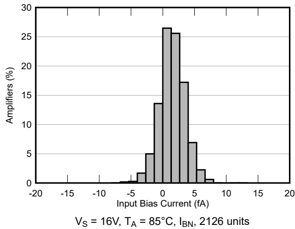
5-3. Input Bias Current Production Distribution
