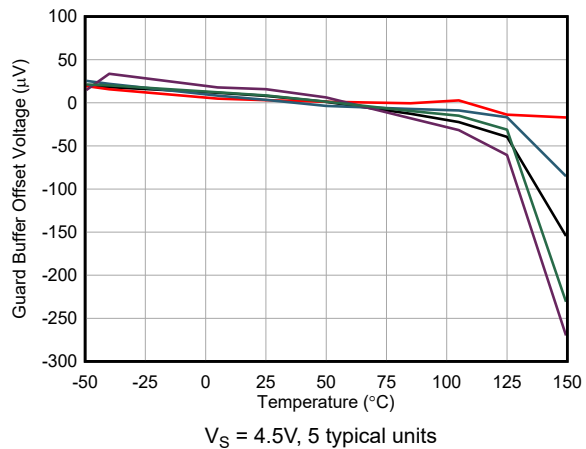
図 5-72. Guard Buffer Offset Voltage vs Temperature
