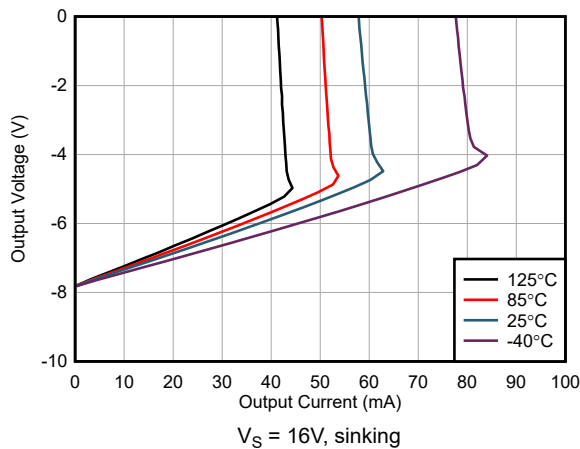
5-35. Output Voltage Swing vs Output Current
