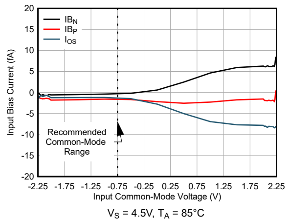
5-24. Input Bias Current vs Common-Mode Voltage
