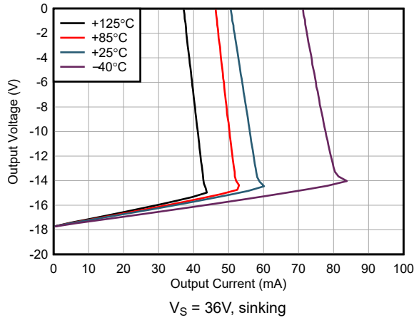
5-37. Output Voltage Swing vs Output Current
