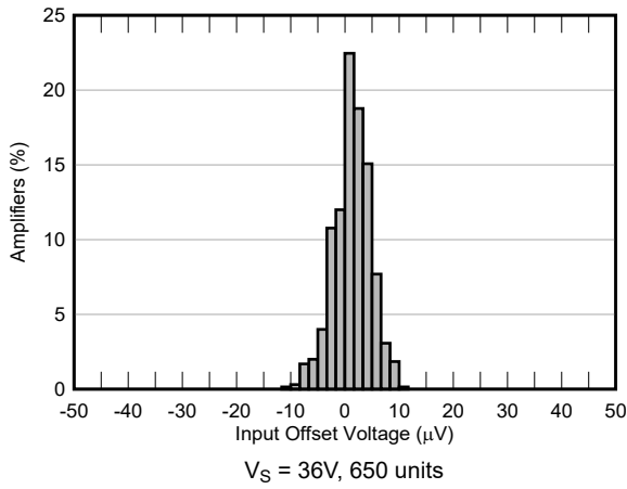
図 5-67. Guard Buffer Offset Distribution
