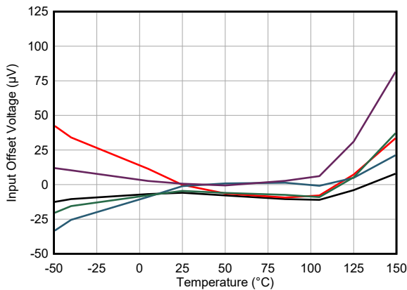
图 5-15. Offset Voltage vs Temperature
