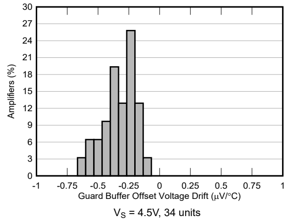
図 5-68. Guard Buffer Offset Drift Distribution
