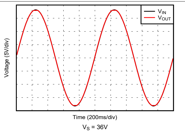
5-56. No Phase Reversal
