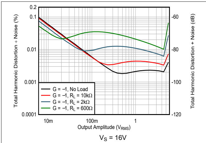
Figure 5-49. THD+N vs Output Amplitude
