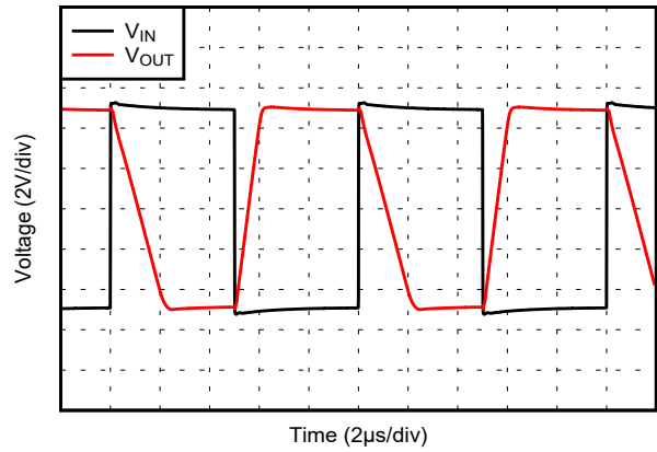
5-62. Large-Signal Step Response
