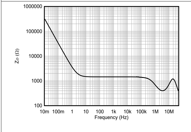
Figure 5-53. Open-Loop Output Impedance vs Frequency
