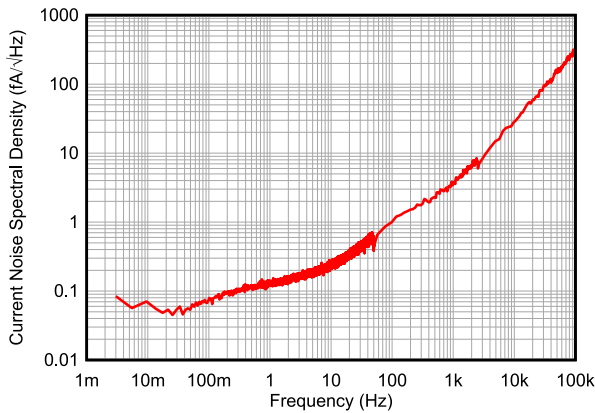
5-41. Input Current Noise Spectral Density vs Frequency
